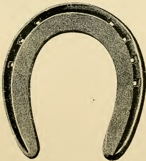
FIG. 241.—Thin heeled fullered seated fore shoe. Made from 1 \times \frac{5}{8} inch iron.
