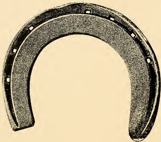
FIG. 370.—Three-quarter fullered seated fore shoe. Made from 1 \times \frac{1}{2} inch iron.
