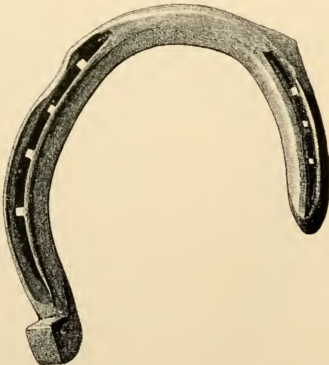
FIG. 299.—Concave three-quarter hind shoe. Made in concave tool from \frac{3}{4} \times \frac{1}{2} inch iron.
