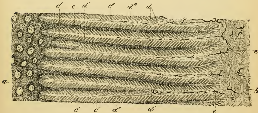
FIG. 50.—Transverse incision through the laminal sheath. a , inmost part of the middle sheath; the horn tubules are seen to reach right up to the horny laminae; b , body of the sensitive wall; c , cornified portion of laminae connected with middle sheath of wall; c' , irregular laminae, which do not extend as far as body of sensitive wall; c'' , non-cornified portion of rete mucosum; d , vascular laminae; d' , vascular laminae which during development have split, thence given rise to the irregular horny laminae c' ; e , injected artery.
