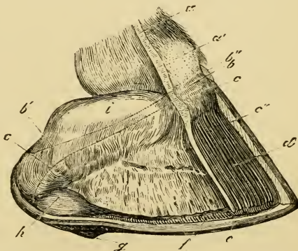
FIG. 41.—Foot from which the outer portion of the horn wall and the greater part of the sensitive structures have been removed, so as to show their relations to the lateral cartilage. a , divided surface of the hair-bearing corium; the cut is continued perpendicularly downwards through the sensitive wall, showing that the latter is only a continuation of the former; a' , hairless portion of hair-bearing corium; b , perioplic ring; b' , line indicating its upper border; b'' , section of perioplic horn; c , coronary band; c (to the left), line indicating the upper border of the coronary band; c'' , section of wall at toe; d , sensitive wall; e , horny sole; f , white line; g , horny frog; h , plantar cushion; i , lateral cartilage.
