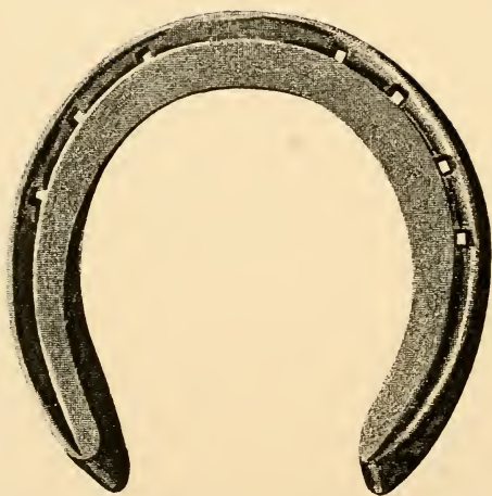
FIG. 211.—Fullered seated fore shoe with thick heels. Made of \frac{7}{8} × \frac{5}{8} inch iron.
