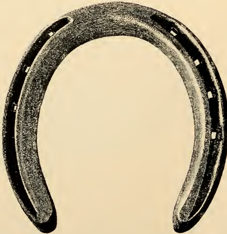
FIG. 217.—Concave partially-fullered, 'dub-toed' fore shoe. Made from \frac{3}{4} \times \frac{1}{2} inch iron.
