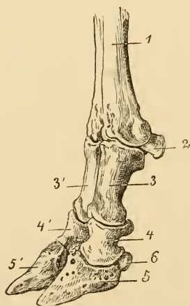
FIG. 397.—Antero-external view of ox's left fore-foot. 1, lower end of metacarpal bone; 2, external sesamoid bone; 3, external, and 3', internal pastern bone; 4, external, and 4', internal coronet bone; 5, external, and 5', internal claw bone; 6, left navicular bone.
