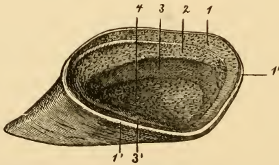
FIG. 399.—Supero-posterior view of an ox's hoof removed by maceration (seen from the inner side). The inner wall is foreshortened owing to the point of view. 1, periople, which at 1' becomes continuous with the bulbs; 2, furrow for reception of coronary band; 3, laminal sheath of the outer wall, and 3', of the inner wall; 4, upper surface of sole.
