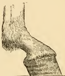
FIG. 169.—Peculiar distortion, in which the os pedis becomes upright, while the suffraginis is much inclined.
