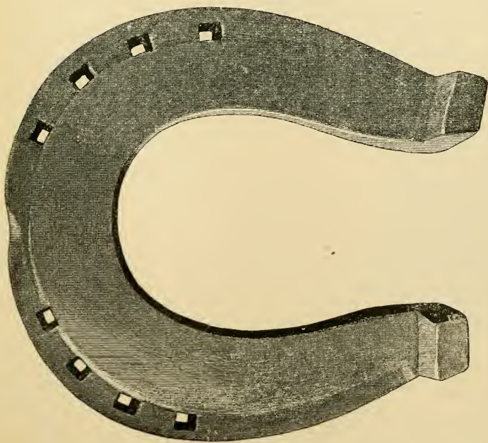
FIG. 325.—Stamped fore shoe (for cart horse), 'set' around outer margin. Made from 1\frac{1}{2} \times \frac{5}{8} inch iron.
