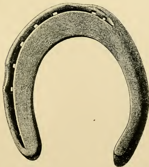
FIG. 293.—Fullered seated feather-edged fore shoe. Made from 1\frac{1}{8} \times \frac{1}{2} inch iron.
