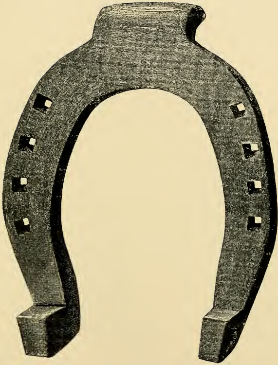
FIG. 328.—Stamped cart hind shoe, with toe-piece. Made from 1\frac{1}{4} \times \frac{5}{8} inch iron.
