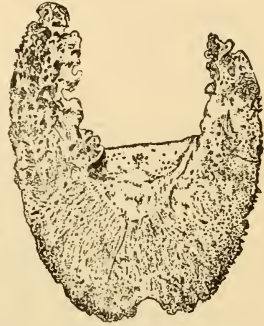
FIG. 367.—Ground surface of pedal bone showing bony enlargements on the wings (retrosal processes) in consequence of old standing corn.
