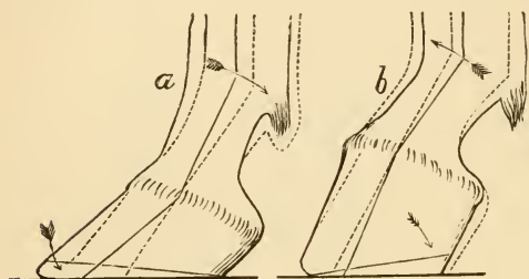
FIG. 168.—Two feet viewed from the side. a , with foot axis distorted in a backward direction; b , in a forward direction. The arrows indicate the proper position of the fetlock, which is given in dotted outline. In a the toe and in b the heels require shortening.
