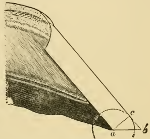
FIG. 198.—Vertical section through wall at toe. a-c , absolute; a-b , apparent thickness. The curve, c-b , indicates the necessary rounding of the toe.
