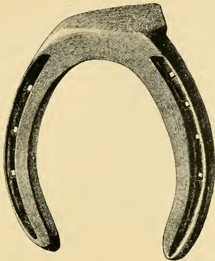
FIG. 276.—Fullered hind shoe for harness horse which forges and wears wall of hind foot. Made from \frac{3}{4} \times \frac{1}{2} inch iron.
