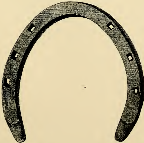
FIG. 223.—Charlier hind shoe, made from Charlier steel, 7-16th inch square.
