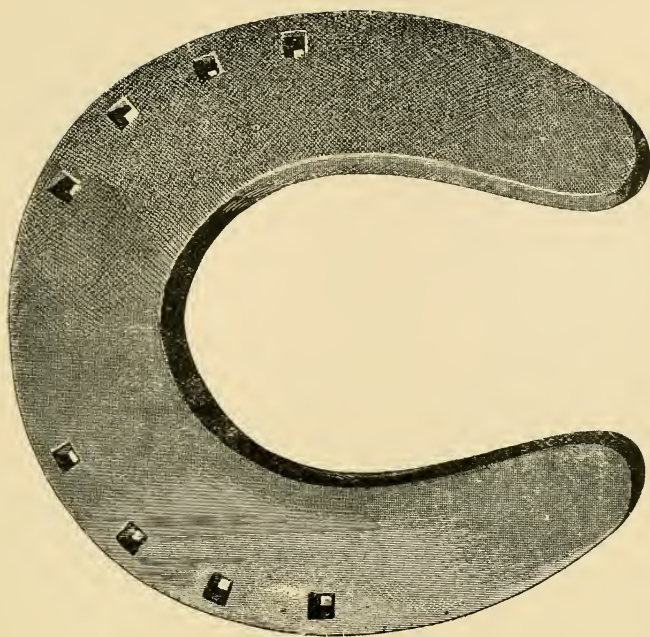
FIG. 324.—Stamped fore shoe (for cart horse). The 'quoit' shoe. Made from 1\frac{5}{8} \times \frac{5}{8} inch iron.
