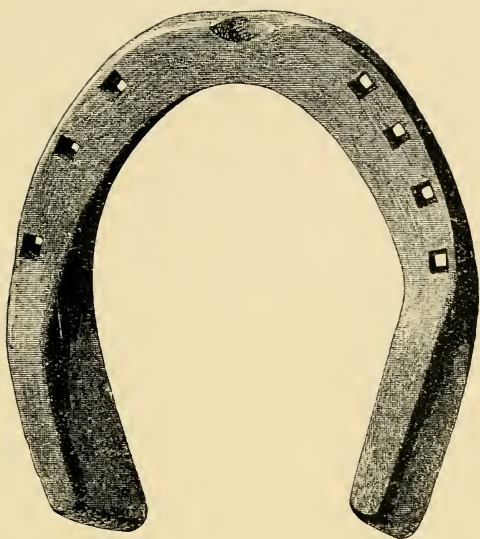
FIG. 389.—Stamped wedge-heeled hind shoe. Made from \frac{3}{4} \times \frac{1}{2} inch iron.
