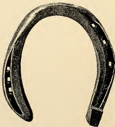
FIG. 295.—Fullered hind shoe for hack. Made from \frac{5}{8} \times \frac{1}{2} inch iron.
