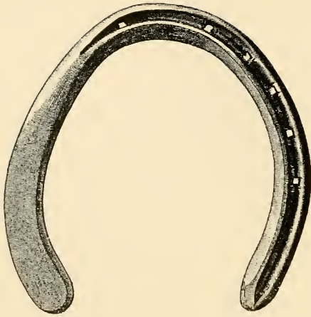
FIG. 298.—Feather-edged fullered concave fore shoe. Made in concave tool from \frac{1}{2} \times \frac{1}{4} inch iron or steel.
