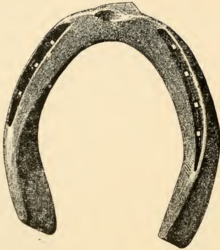
FIG. 391.—Fullered wedge-heeled hind shoe (for harness horse). Made from \frac{3}{4} \times \frac{1}{2} inch iron.
