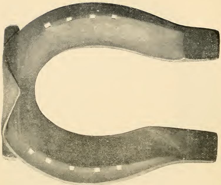
Fig. 249.—'North Country' stamped fore shoe. Made from 1\frac{1}{2} \times \frac{1}{2} inch iron.
