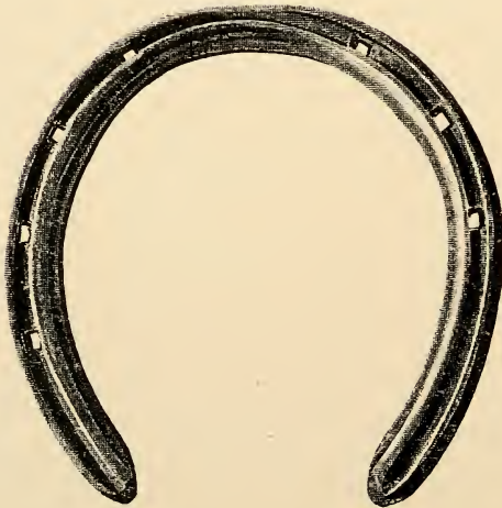
FIG. 227.—Concave fullered fore shoe (for steeplechasing). Made from \frac{3}{8} \times \frac{3}{8} inch iron.
