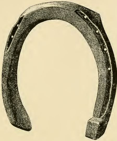
FIG. 288.—Partially feather-edged fullered hind shoe. Made from \frac{3}{4} \times \frac{1}{2} inch iron.
