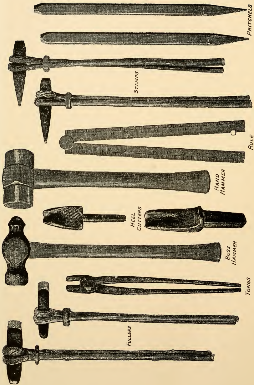
FIREMAN'S TOOLS.
