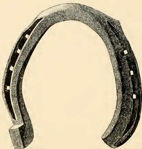
FIG. 290.—Fullered hind shoe, 'set' inside. Made from \frac{5}{8} square iron.
