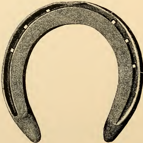
FIG. 396.—Fullered seated fore shoe. Made from \frac{7}{8} \times \frac{1}{2} inch iron.
