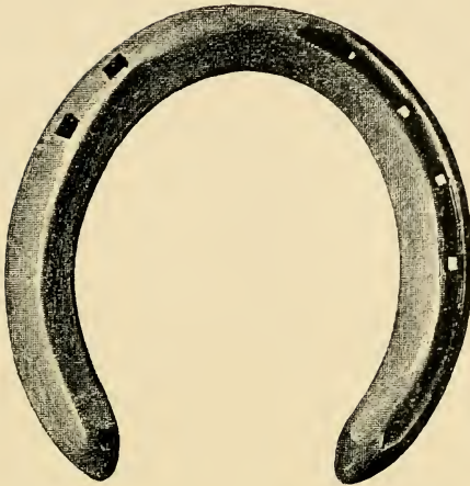
FIG. 218.—Concave fullered, feather-edged fore shoe. Made of \frac{3}{4} \times \frac{1}{2} inch iron in concave tool.
