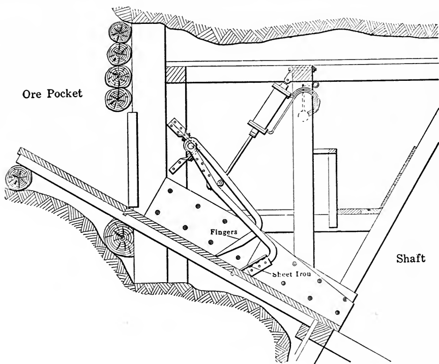
FIG. 101.—GATE FOR SKIP-LOADING CHUTE, GRANBY CONSOLIDATED MINES.
