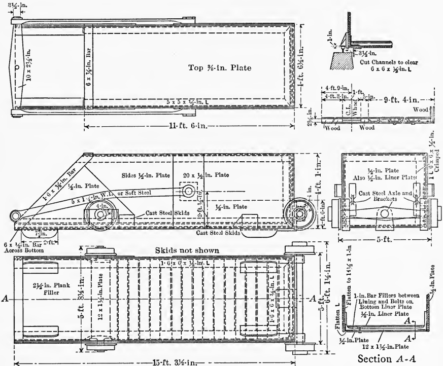
FIG. 162.—THE 10-TON SKIP FOR THE FRANKLIN MINE.
