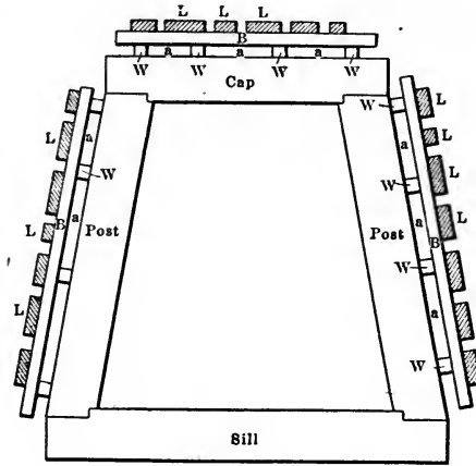
FIG. 65.—DRIFT TIMBERING IN RUNNING GROUND.
