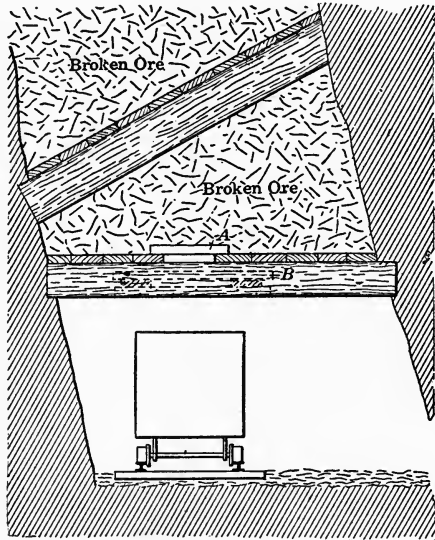
FIG. 90.—THE IMPROVED "CHINAMAN."
