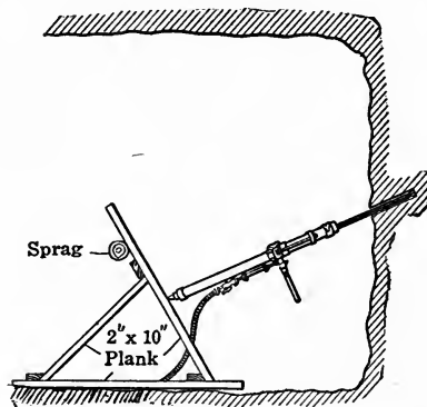
FIG. 59.—FOOT FRAME FOR STOPING DRILL.
