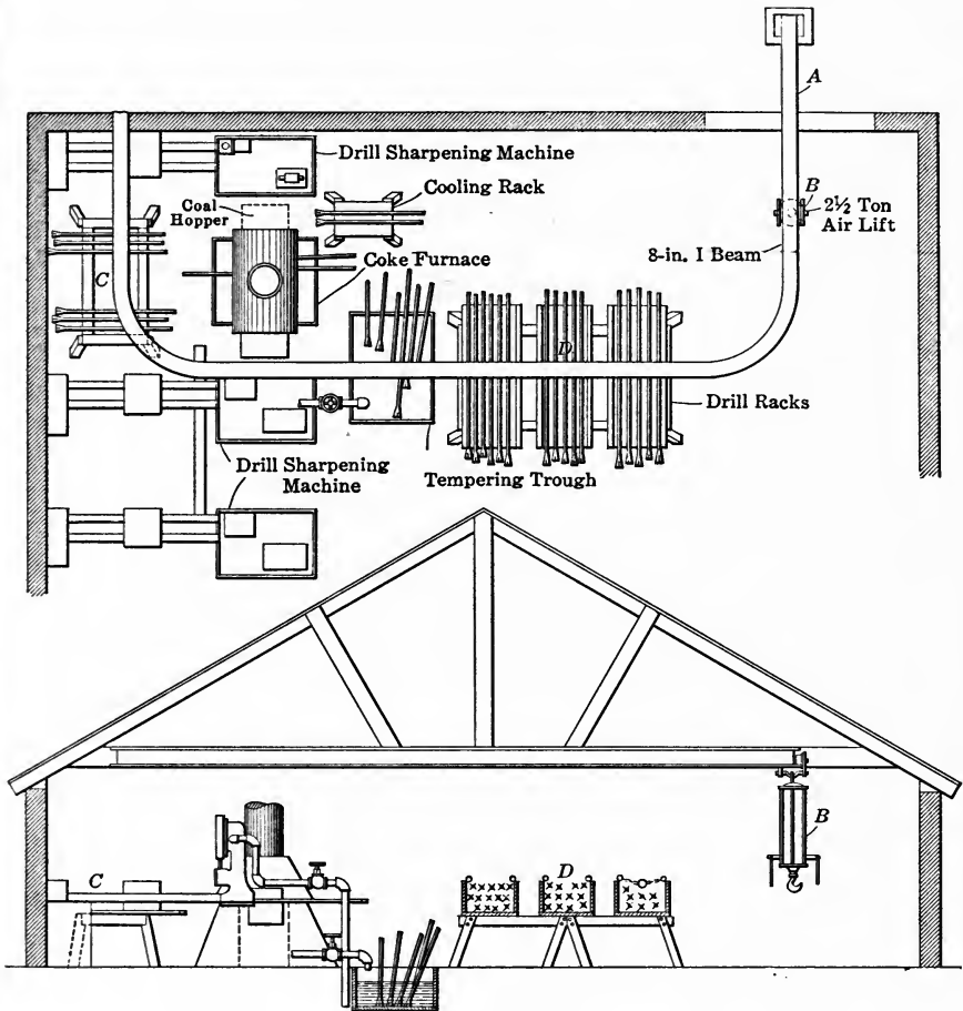
FIG. 30.—DRILL SHARPENING PLANT AT CHAMPION MINE.
