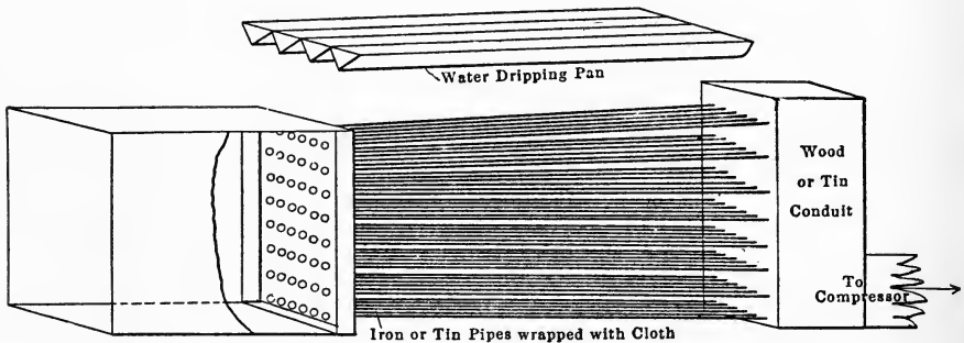
FIG. 246.—PRECOOLER FOR AIR COMPRESSORS.
