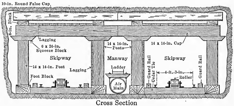
FIG. 46.—POSTS AND SQUARE TIMBERS IN AN INCLINED SHAFT.
