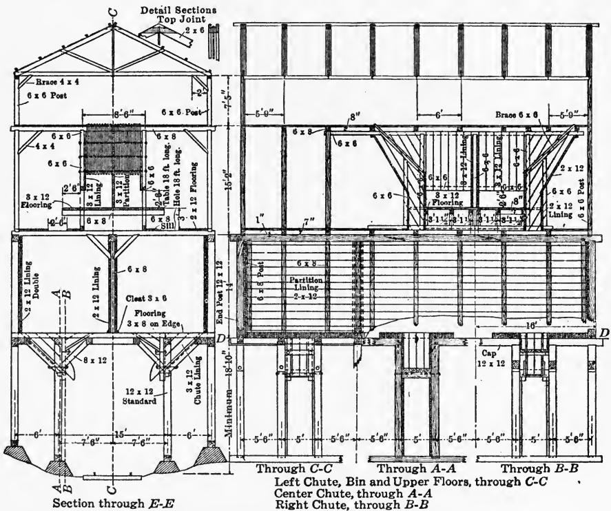
FIG. 114.—SECTIONS OF TONOPAH-BELMONT OREHOUSE.
