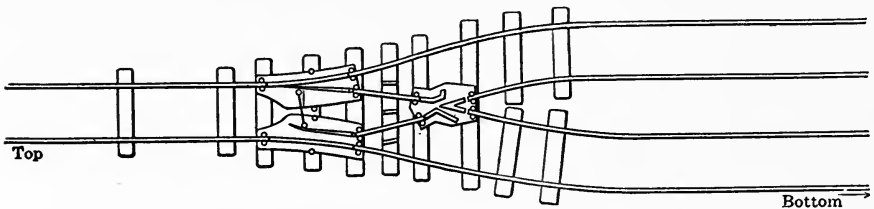
FIG. 219.—SWITCH FOR GRAVITY TRAM.
