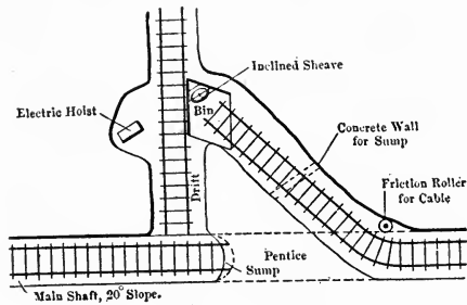
FIG. 37.—PLAN OF STELLA SHAFT.
