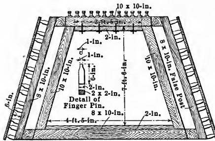
FIG. 70.—BRIDGE SETS WITH LAGGING OVER FINGER PINS.
