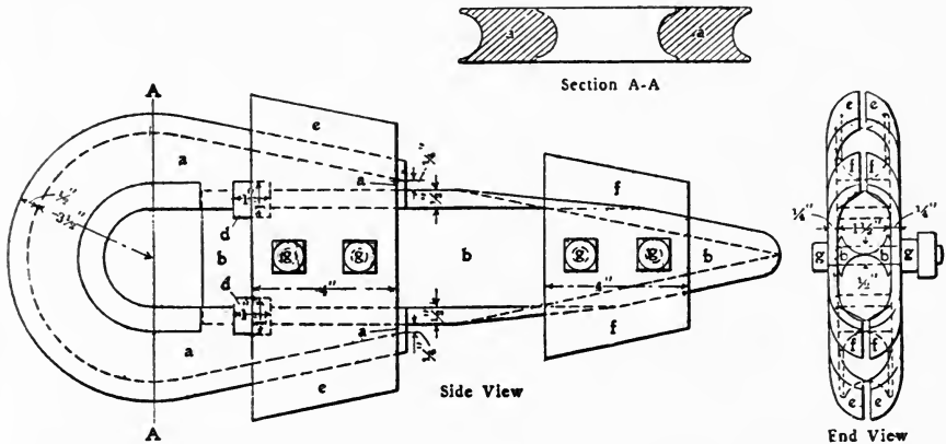
FIG. 195.—DETAILS OF HOISTING-CABLE THIMBLE.
