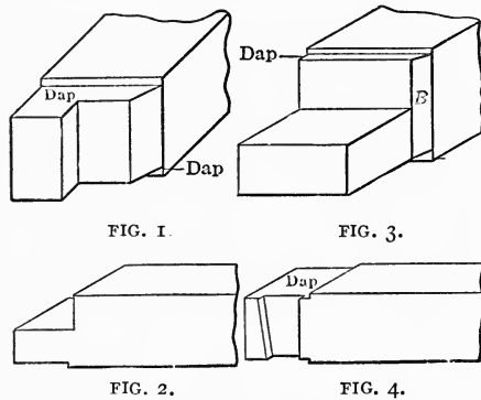
FIG. 40.—SHAFT TIMBER ENDS.
