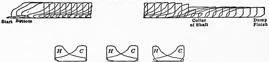
FIG. 134.—CONTINUOUS DIAGRAM FROM AN AUTOMATIC CUTOFF HOISTING ENGINE.
