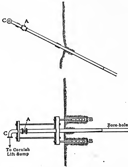
FIG. 235.—DRILL HOLE AND FITTINGS.
