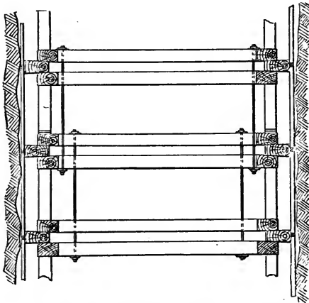
FIG. 47.—SHAFT TIMBERING IN SWELLING GROUND.
