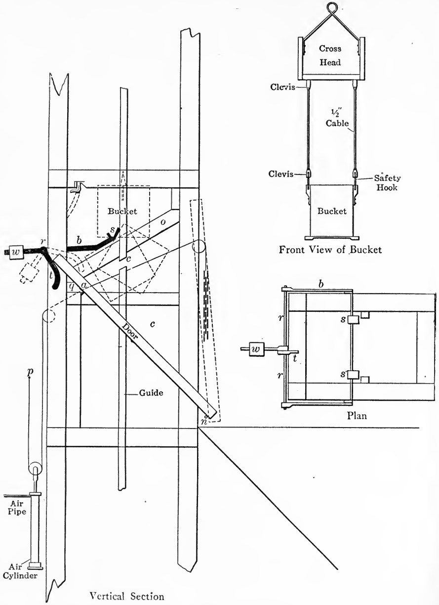
FIG. 178.—SELF-DUMPING BUCKET USED AT BULLY HILL MINE.
