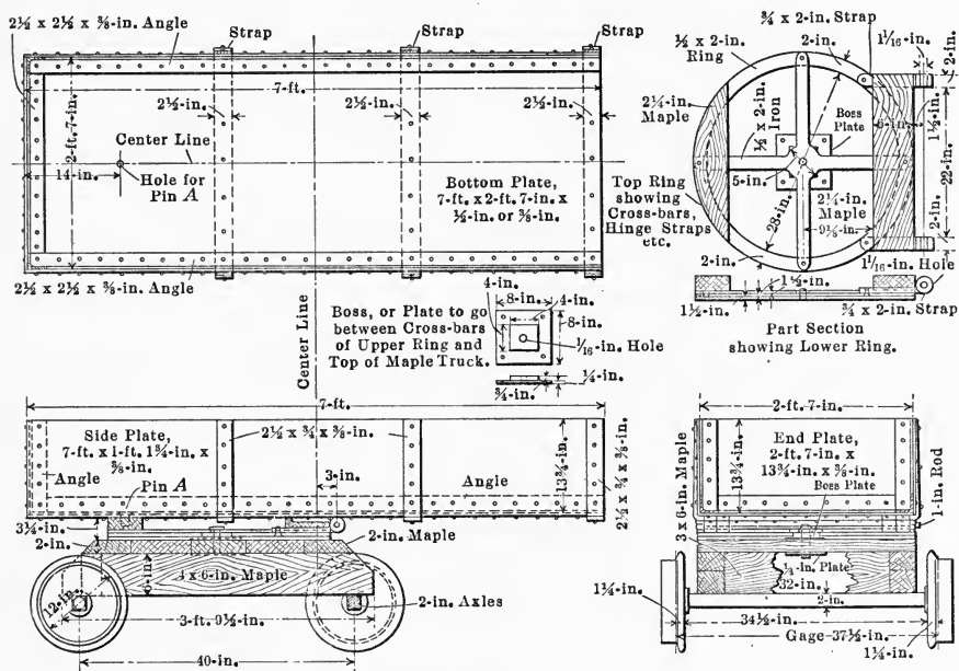
FIG. 155.—TRIMOUNTAIN CAR FOR STOPE FILLING.
