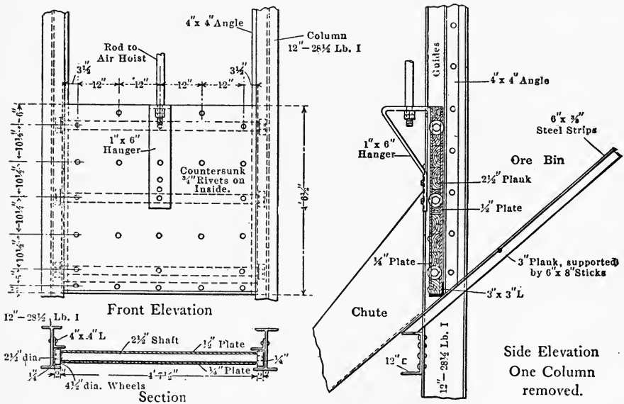
FIG. 94.—AIR-HOIST GATE FOR COARSE ORE.
