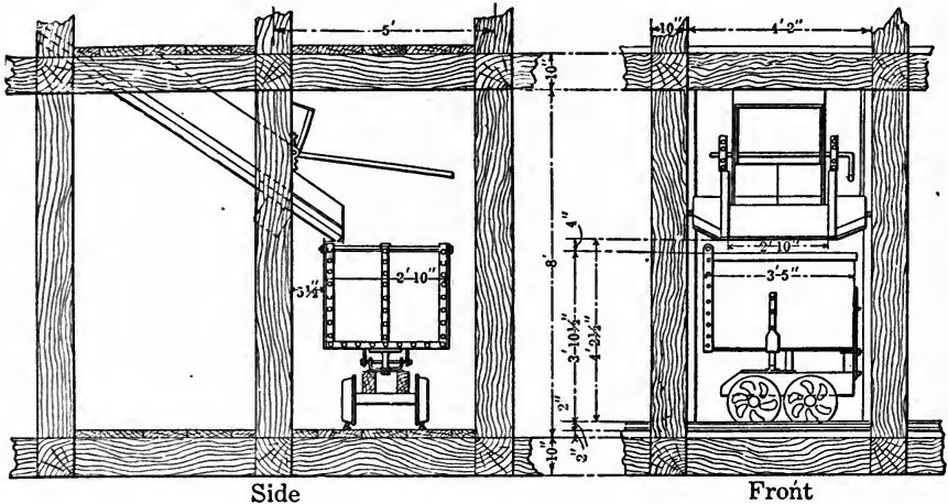
FIG. 91.—STANDARD ORE CHUTE IN GOLDFIELD CONSOLIDATED MINE.
