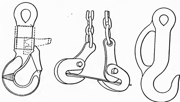
FIG. 193.—TYPES OF SAFETY CRANE HOOKS.
