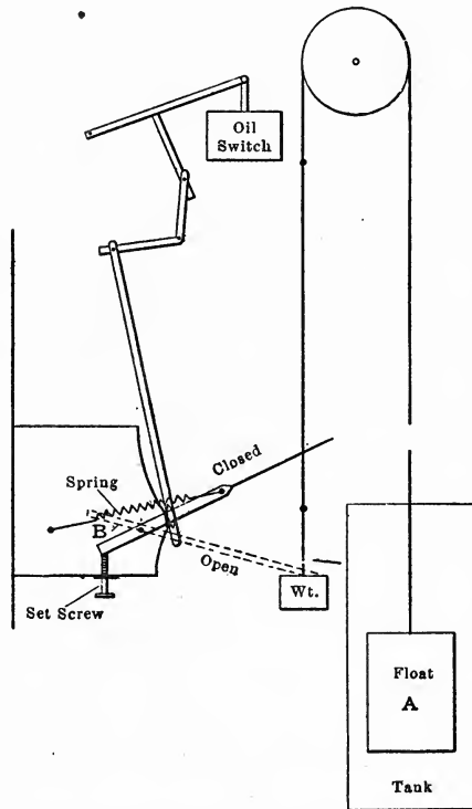
FIG. 226.—ARRANGEMENT OF AUTOMATIC CUT-OFF.
