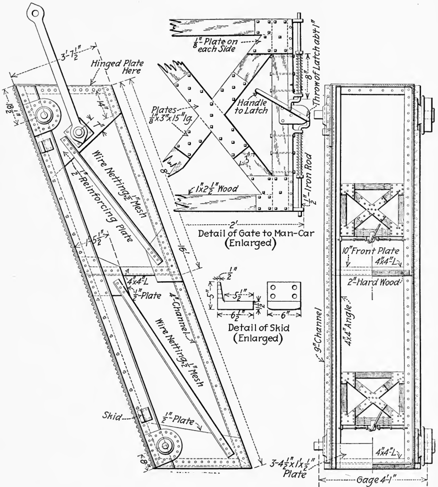
FIG. 160.—MAN CAR FOR AN INCLINED SHAFT.
