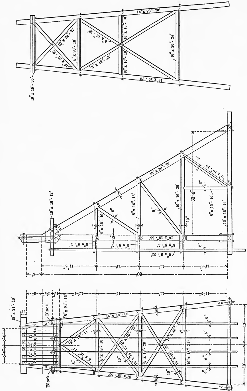
FIG. 110.—THE CLERMONT HEADFRAME, GOLDFIELD CONSOLIDATED MINES CO.
