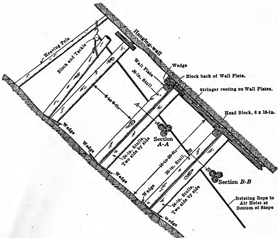
FIG. 83.—BATTERY STULLS IN CALUMET & HECLA STOPE.
