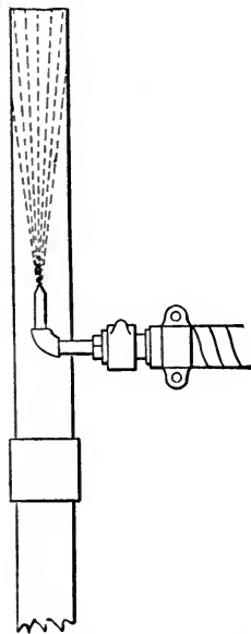
FIG. 236.—JET FOR VENTILATING BY COMPRESSED AIR.
