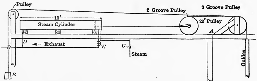
FIG. 129.—SKETCH SHOWING PISTON ARRANGEMENT FOR COAL LIFT.
