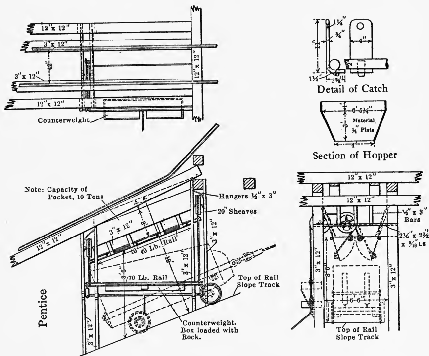
FIG. 105.—UNDERGROUND ORE POCKET
