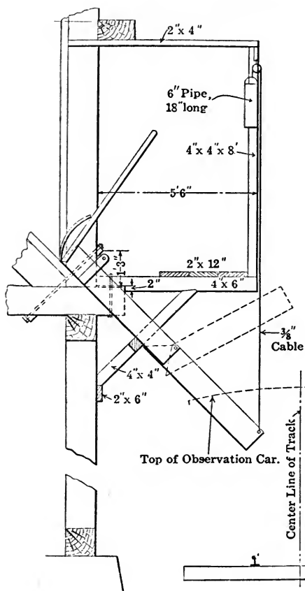
FIG. 97.—ELEVATION OF CANANEA BINS.
