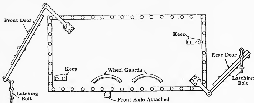
Side Elevation of Car Body.
