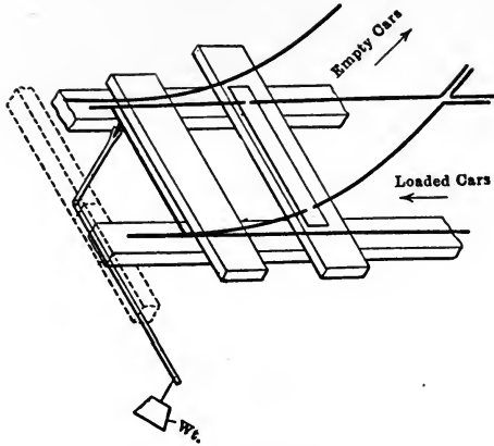
FIG. 221.—GRAVITY SWITCH FOR ORE CARS.
