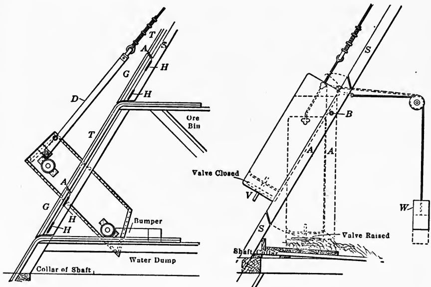
FIG. 171.—AUTOMATIC DISCHARGING BAILERS.
