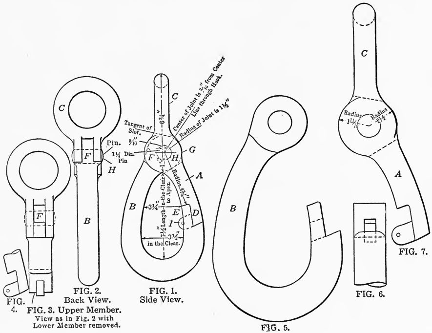
FIG. 194.—A NEW SAFETY CRANE HOOK.
