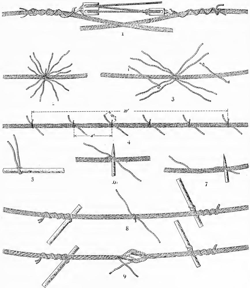
FIG. 6.—METHODS OF SPLICING WIRE ROPE.
