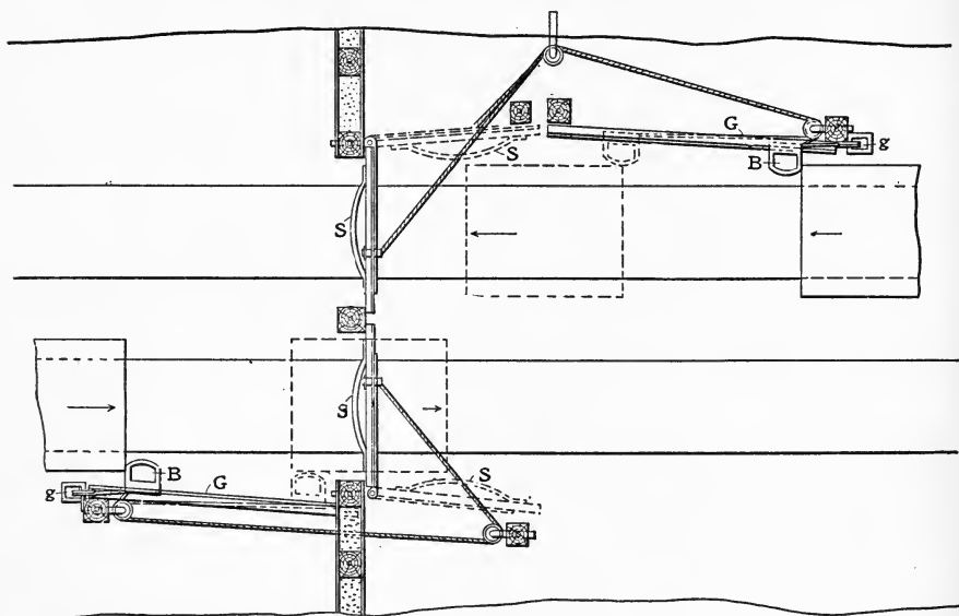
FIG 242.—SELF-ACTING MINE DOORS FOR DOUBLE TRACK DRIFT OR TUNNEL.
