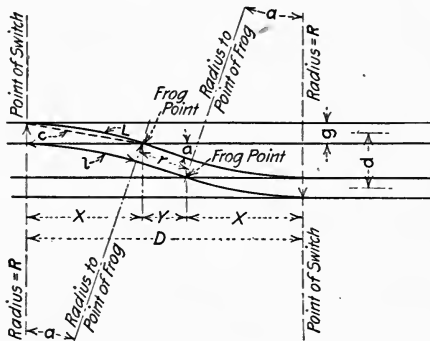
FIG. 218.—CALCULATING A CROSSOVER SWITCH.
