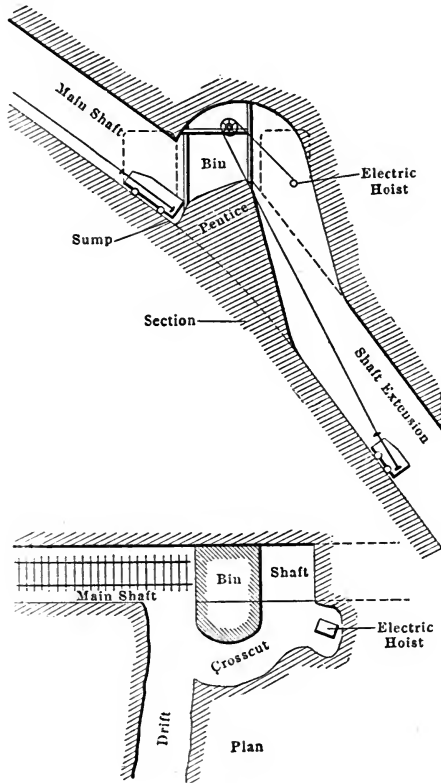
FIG. 36.—DETAILS OF ANNA SHAFT EXTENSION.
