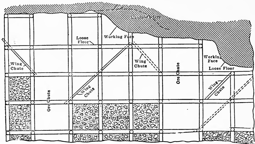
FIG. 73.—SECTION OF STOPE SHOWING DIVERTING WING CHUTES.
