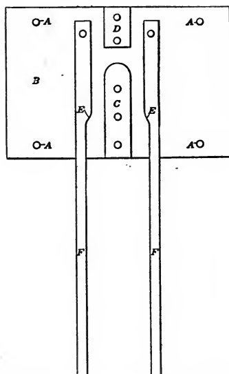
FIG. 23.—DEVICE FOR SHAPING CHUCK BOLTS.
