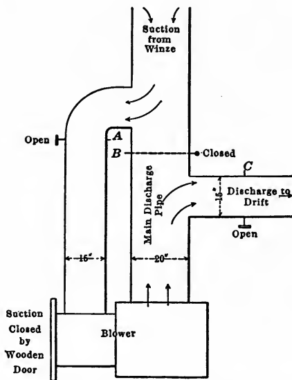
FIG. 240.—PIPE ARRANGEMENT FOR FAN BLOWER USED ON COMSTOCK LODE.
