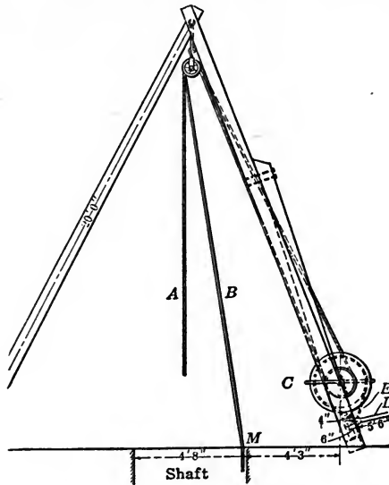
FIG. 130.—DEVICE FOR LOWERING TIMBERS IN IRON MINES.
