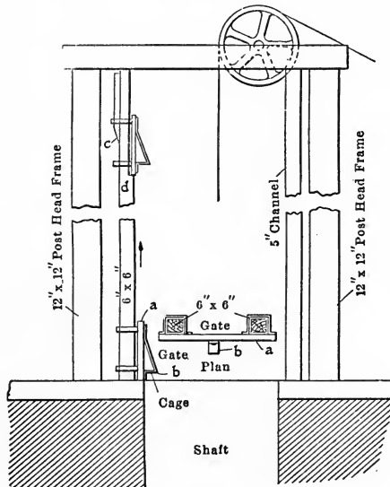
FIG. 211.—OPERATION OF SHAFT GATES.
