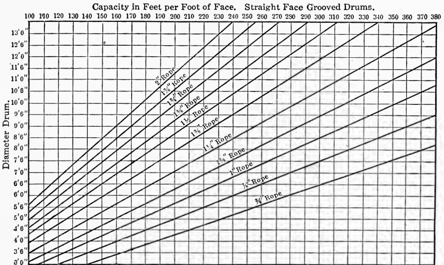
FIG. 121.—CHART FOR DETERMINING THE FACE OF A GROOVED DRUM.
