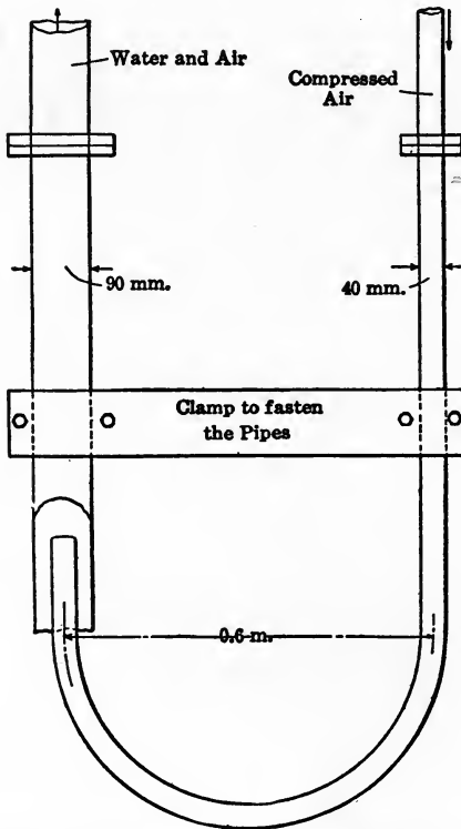
FIG 229.—AIR LIFT FOR UNWATERING SHAFT.
