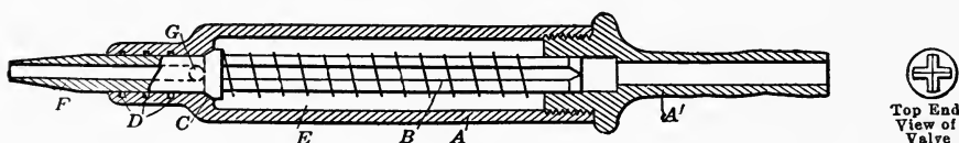
FIG. 147.—NONLEAKING OILER FOR TRAMWAY BUCKETS.
