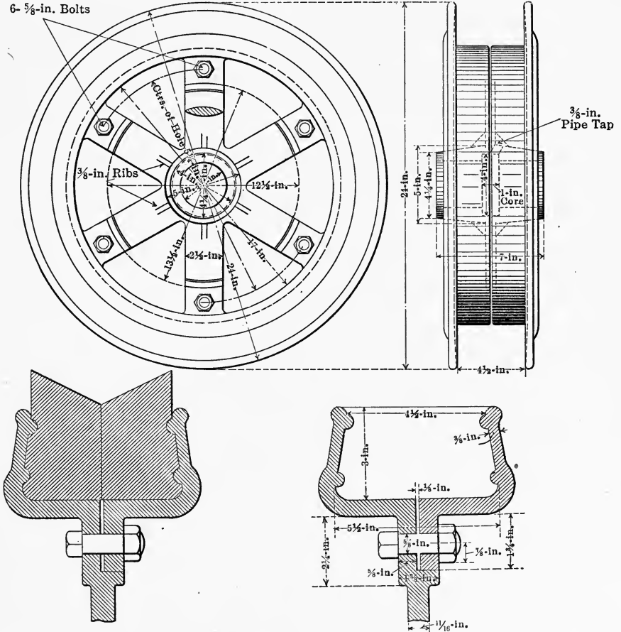
FIG. 139.—IDLER FOR HOISTING ROPES USED AT CHAMPION MINE.
