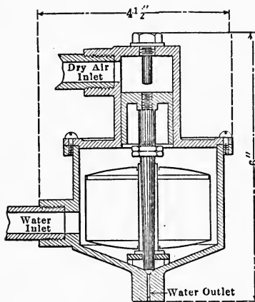
FIG. 252.—EJECTOR VALVE FOR AIR LINE.
