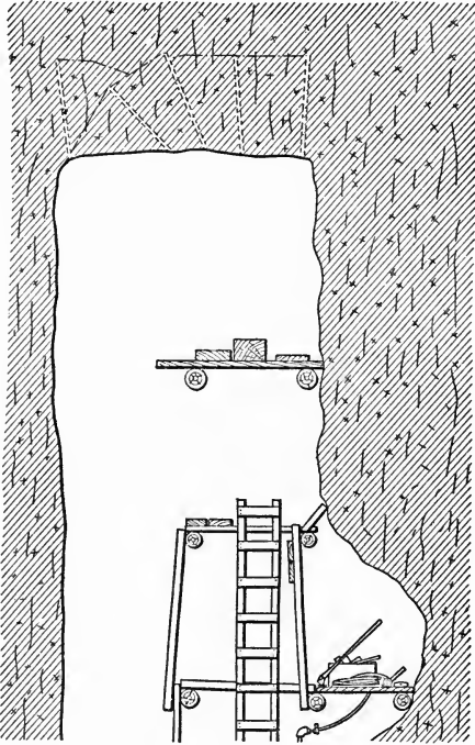
FIG. 61.—STATION AND TIMBERING IN VERTICAL RAISE.
