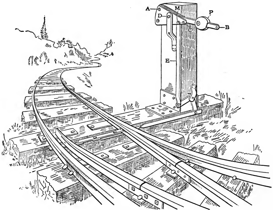
FIG. 222.—THE PETERSEN SWITCH.
