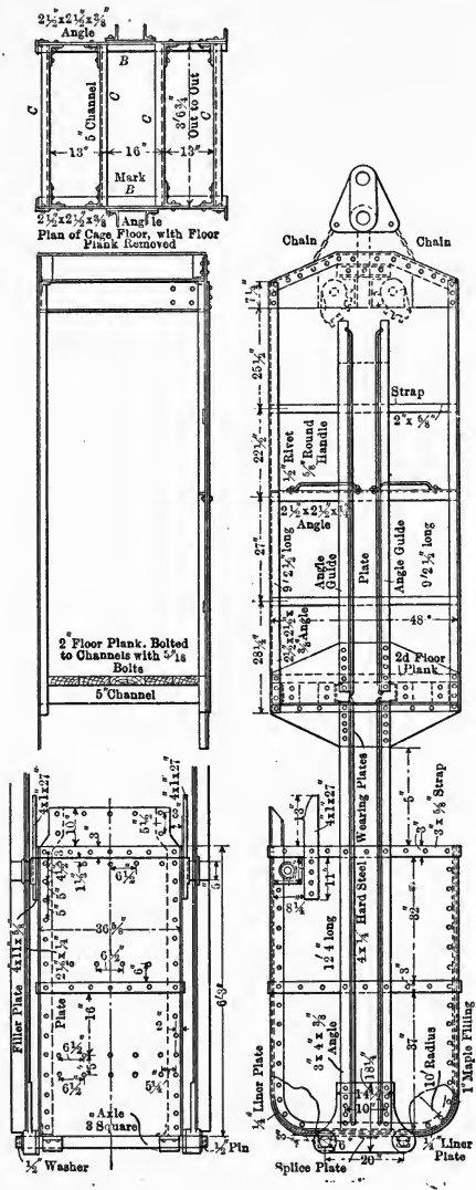
FIG. 167.—HIAWATHA CAGE WITH SKIP ATTACHED.
