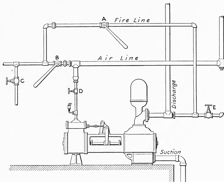
FIG. 227.—PUMP CONNECTED TO AIRLINES FOR FIRE SERVICE.
