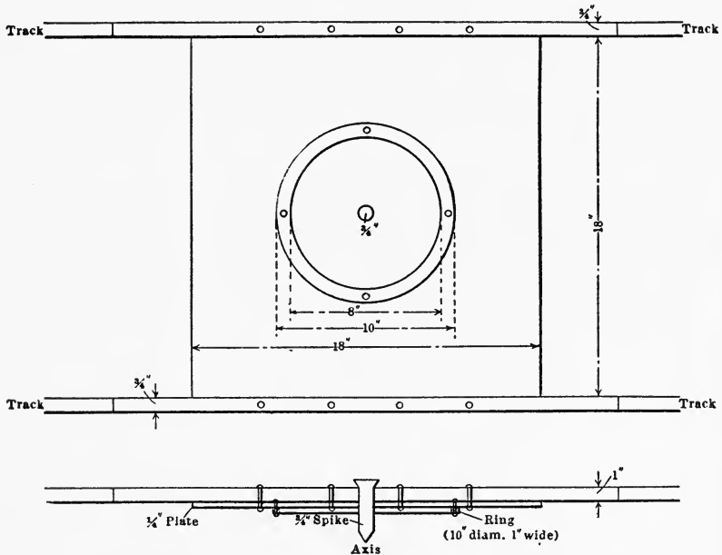
FIG. 223.—TURNTABLE USED IN HIGHLAND BOY MINE.
