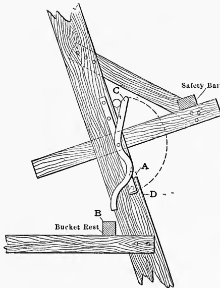
FIG. 176.—AUTOMATIC BUCKET TRIP.
