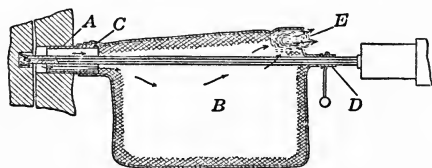
FIG. 33.—DWYER DUST-COLLECTING DEVICE.
