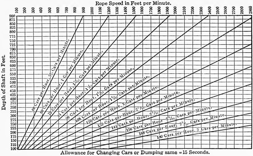
FIG. 120.—CHART TO DETERMINE NUMBER OF CARS HOISTED PER HOUR.
