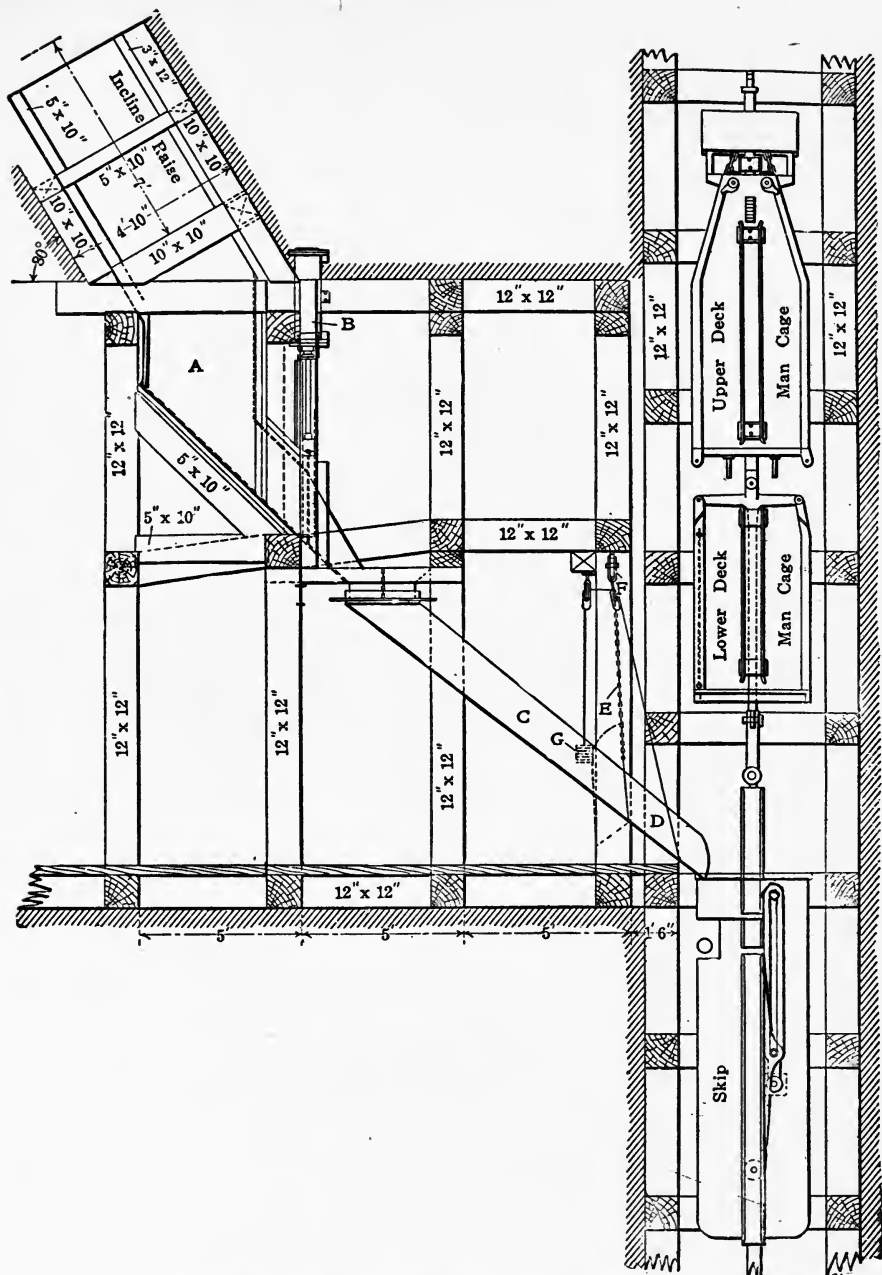
FIG. 99.—SKIP LOADING ARRANGEMENT FOR ORIGINAL CONSOLIDATED MINING CO., BUTTE, MONT.
