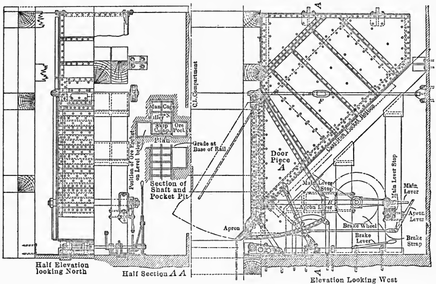
FIG. 103.—DETAILS OF A STEEL ORE POCKET IN RED JACKET SHAFT.
