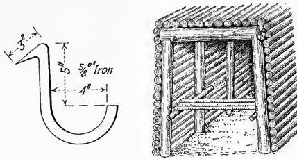
FIG. 62.—STAGING STAPLE AND MANNER OF USING IT.
