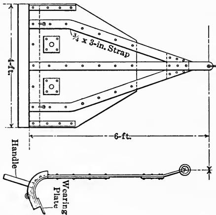
FIG. 173.—A LAKE SUPERIOR STOPE-FLOOR SCRAPER.
