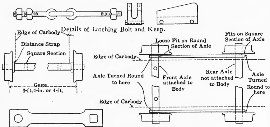
Plan of Truck.
