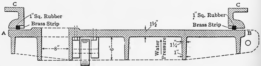
FIG. 234.—CAST IRON GATE FOR MINE DRIFTS.
