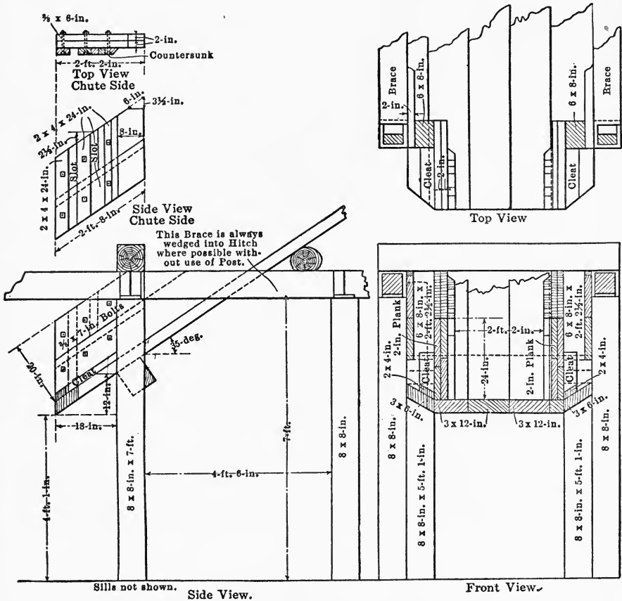
FIG. 92.—STANDARD ORE CHUTE USED AT NEVADA-DOUGLAS MINES.
