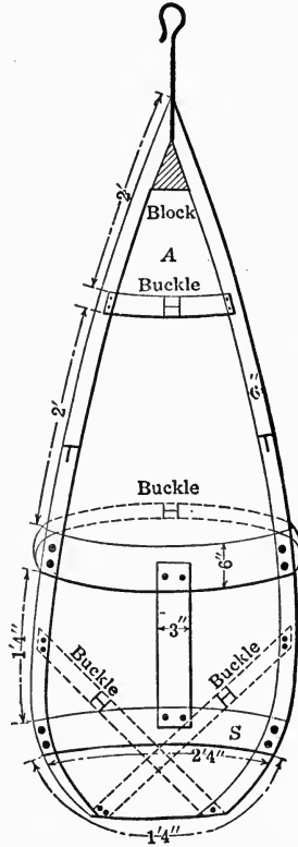
FIG. 170.—HARNES FOR LOWERING MULES.
