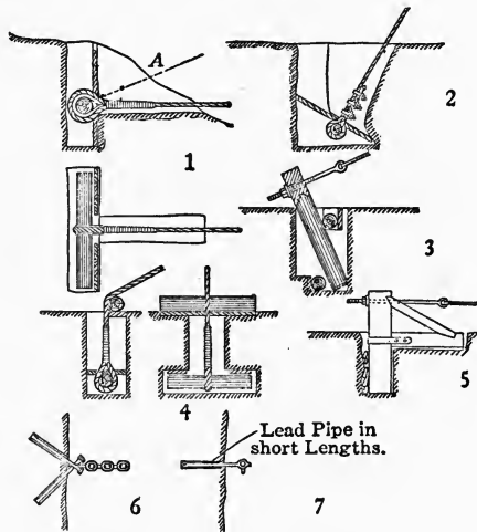
FIG. 148.—WIRE-ROPE ANCHORAGE.
