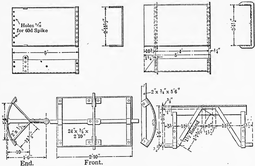
FIG. 98.—DETAILS OF METAL PART OF ARC-TYPE GATE FOR CHUTES.
