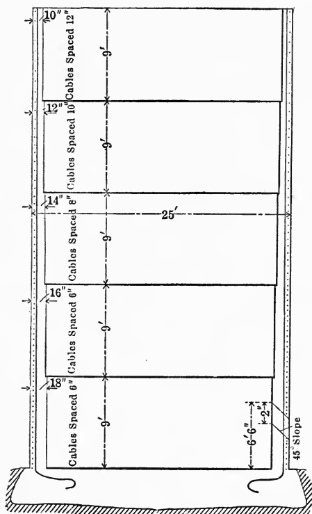
FIG. 116.—CONCRETE STORAGE BIN, MINERVILLE, N. Y.
