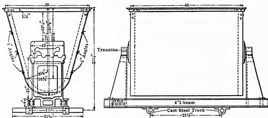
FIG. 156.—SIDE-DUMP CAR USED AT NORTH STAR MINE, GRASS VALLEY, CALIF.
