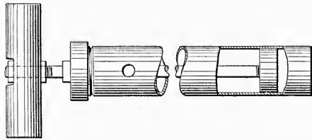
FIG. 11.—DEVICE FOR MOLDING TAMPING CARTRIDGES.
