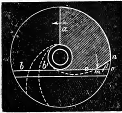
FIG. 74.—Shearing edge.
