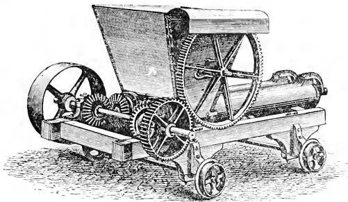
FIG. 59.—Double-spiral pulp peat machine.
