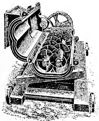
FIG. 45.—Double-spiral, rapidly rotating peat machine, with discontinuous screw-threads, for fibrous peat.
