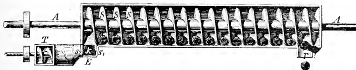
FIG. 24.—Eichhorn's "ball peat drum."
