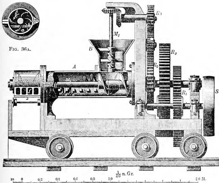
FIG. 36.—Peat Machine of Henry Clayton, Son, and Hewlett, London.
