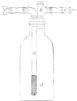
Natronkalkflasche zu Benedict's Apparat.
