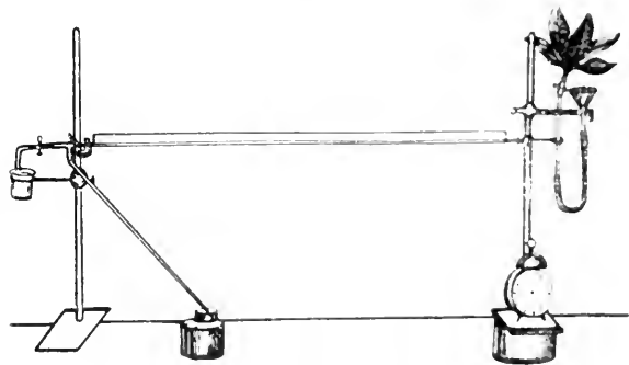
O. Renner's Potometer.
