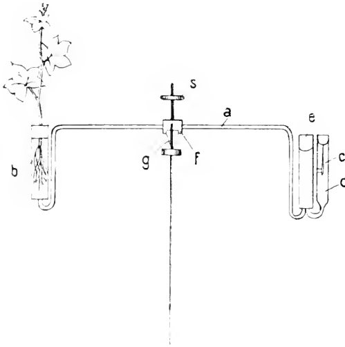
J. Vesque Apparat zur Transpirationmessung.
