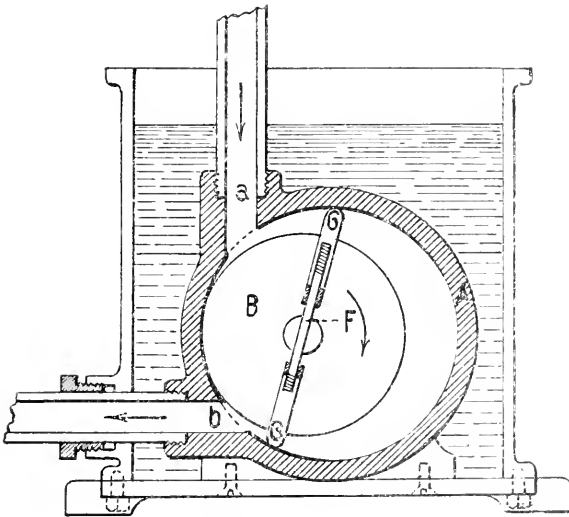
Rotationspumpe.
