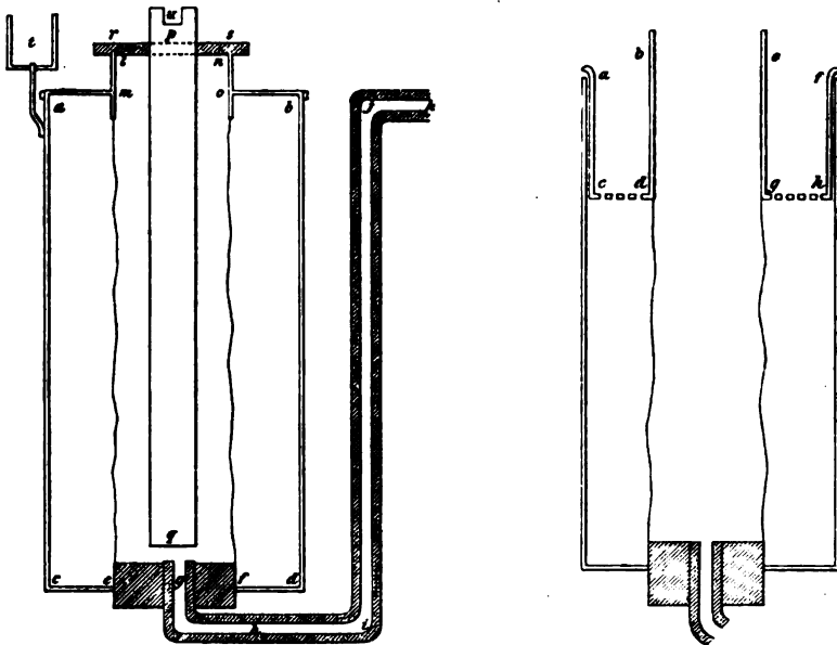
Fig. 10. Original-Daniell-Element.
