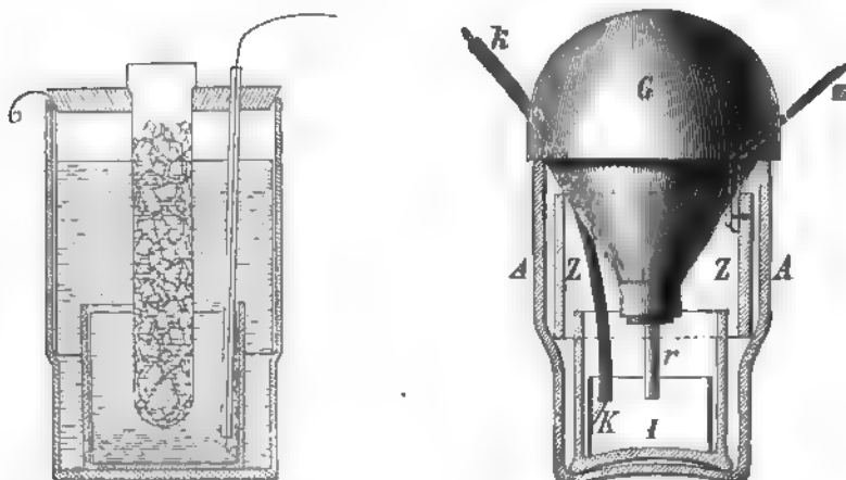
Fig. 12 (Originalform) Meidinger-Element. Fig. 13. (Neue Form)
