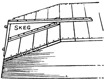
FIG. 451. — Attachment of Skeg.
