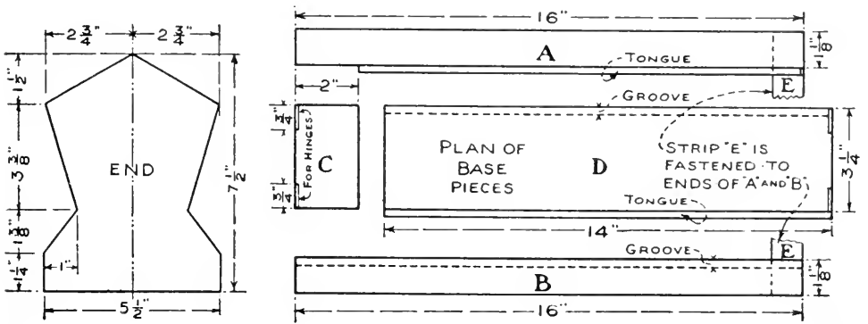
FIG. 121. — Details of Extension Book-rack shown in Fig. 114.
