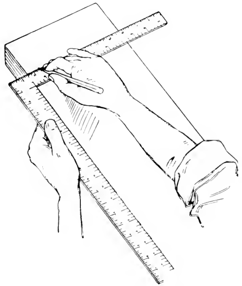
FIG. 69. — Gauging with Pencil and Carpenter's Square.
