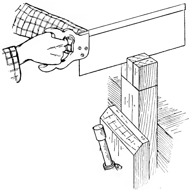
FIG. 80. — Cutting the Sides of a Tenon.
