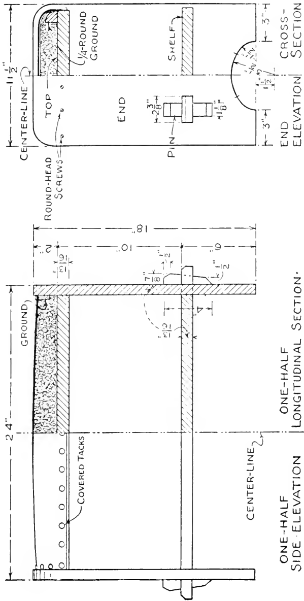
FIG. 129. — Details of Footstool shown in Fig. 125.
