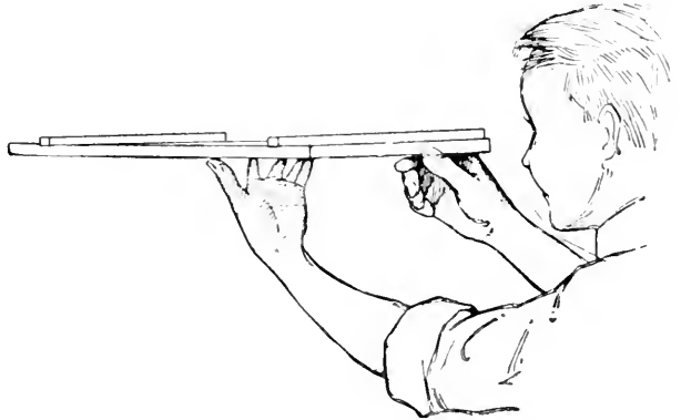
FIG. 73. — Testing with Winding-sticks.
