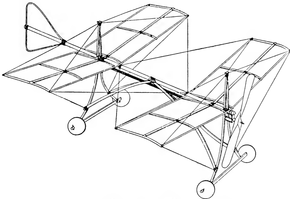
FIG. 397. — A More Elaborate Monoplane Model.
