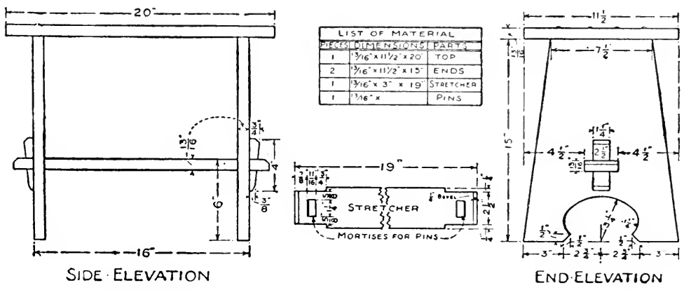
FIG. 128. — Details of Plant Stand shown in Fig. 124.
