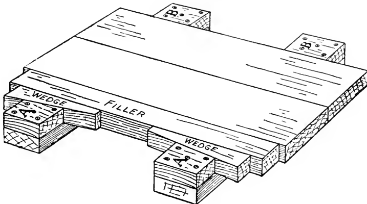
FIG. 42.—Home-made Clamps for Holding Glued-up Work.
