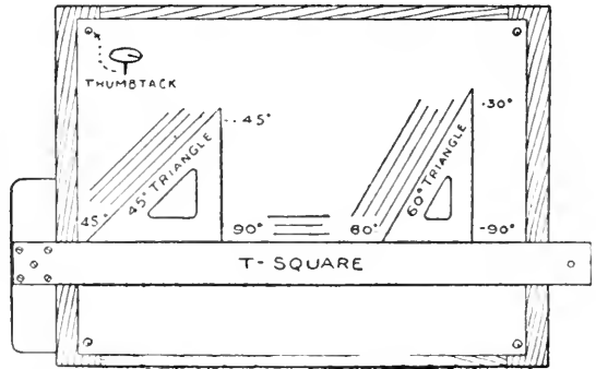
FIG. 93. — A Student's Drawing-board (size 16" × 22") and T-square and Triangles.
