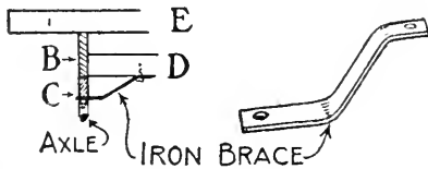
FIG. 461. — Brace for the Front Axle.
