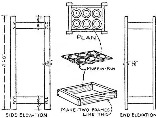
FIG. 138. — Details of Umbrella-stand shown in Fig. 134.
