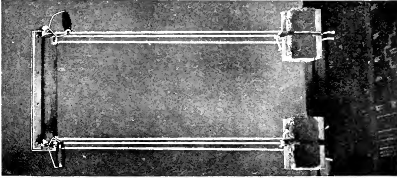
FIG. 206. CONSTRUCT YOUR CHEST-WEIGHTS FIRST.
