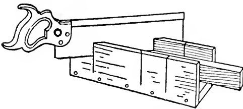
FIG. 59. — Home-made Miter-box.
