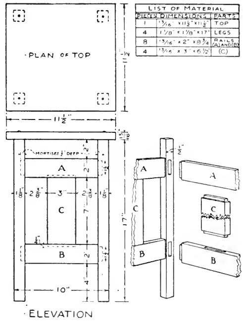
FIG. 127. — Details of Tabouret shown in Fig. 123.
