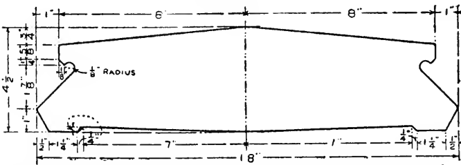
FIG. 118. — Detail of Back of Towel-rack shown in Fig. 111.
