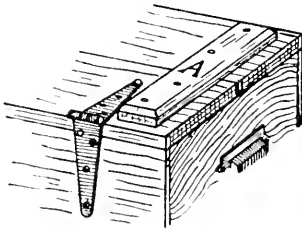
FIG. 44. How to hinge the Cover.
