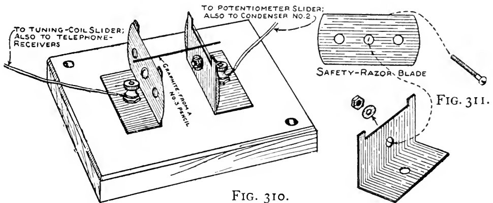
FIG. 310. — A Safety-razor Blade Microphone Detector.
