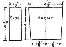
FIG. 115. — Whisk-broom Holder shown in Fig. 108.
