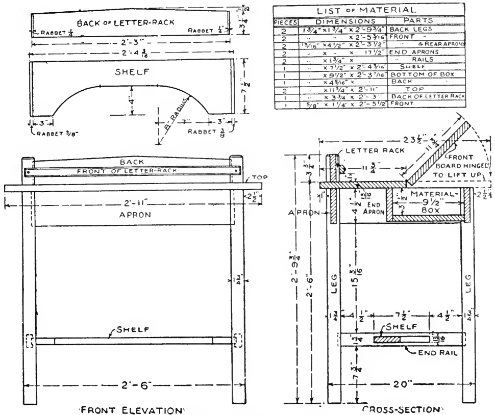
FIG. 145. — Details of Mission Writing-desk shown in Fig. 141.
