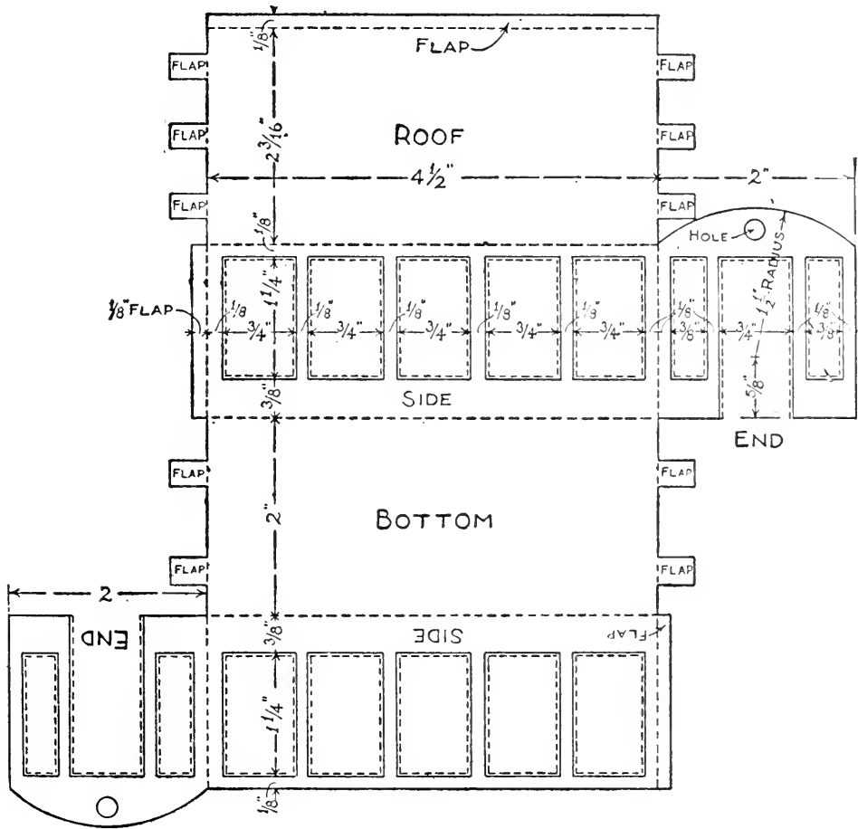
FIG. 276. — Pattern for the Ferris Wheel Cars.
