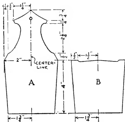
FIG. 248. — Patterns for Whisk-broom Holder.
