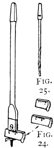
FIG. 24. — Expansive-bit. FIG. 25. — Wood Drill Bit.
