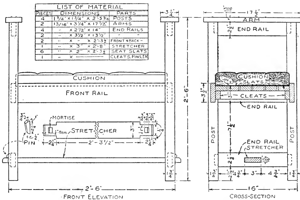
FIG. 143. — Details of Roman Chair shown in Fig. 139.
