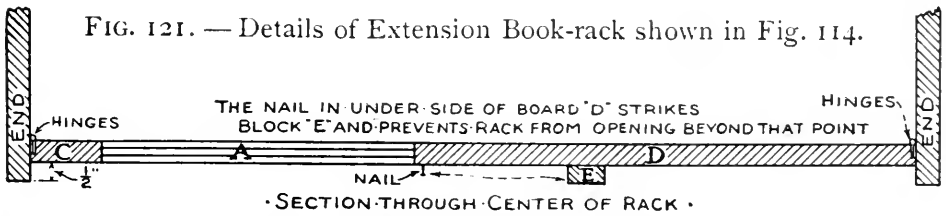
FIGS. 119-121. — Working-drawings for Book-racks.
