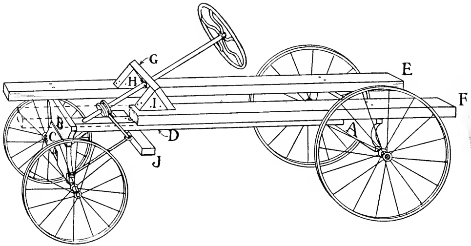
FIG. 462. — Framework of the Pushmobile.
