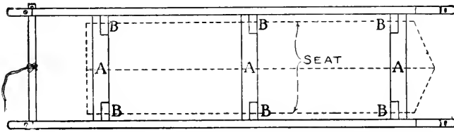
FIG. 370. — Plan of Runners and Cross-pieces.
