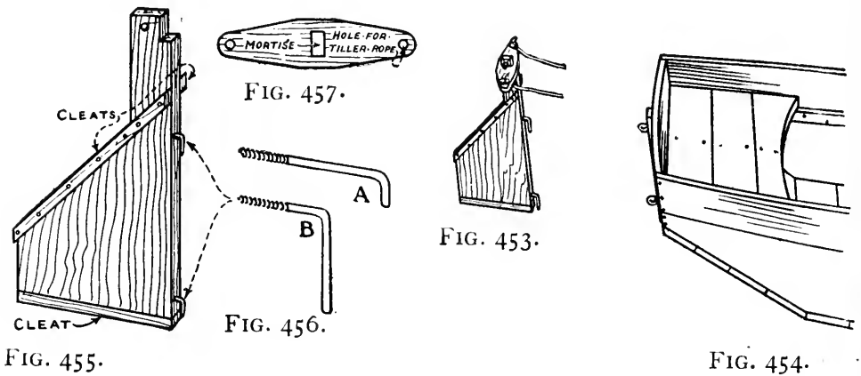
FIGS. 453-457. — Details of an Easily Made Rudder.
