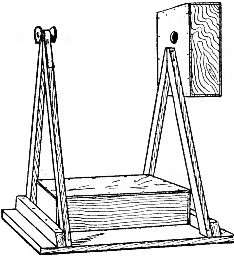
FIG. 267. — Standard for the Ferris Wheel.
