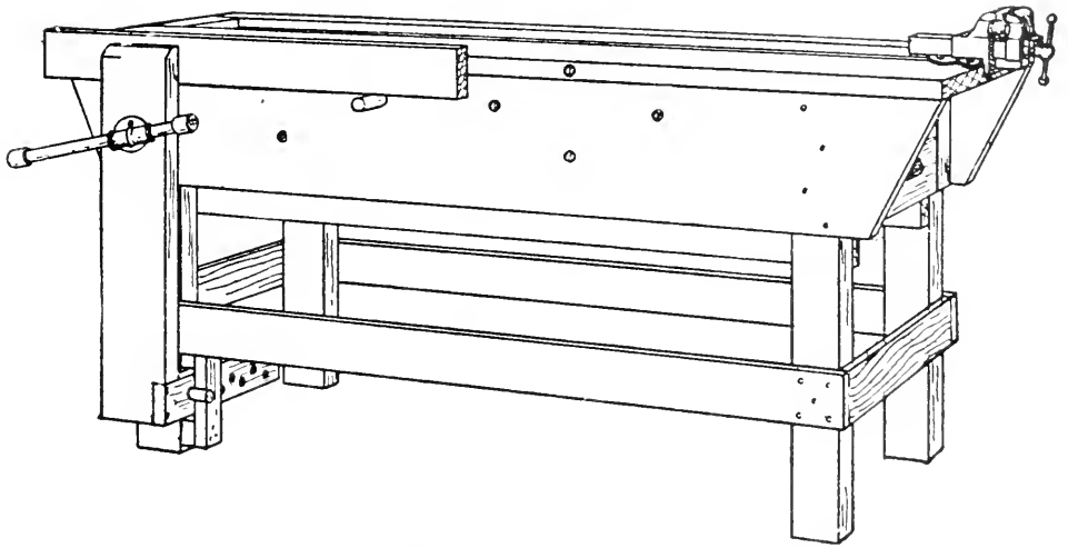
FIG. 6. — A Work Bench with Tool Drawers.
