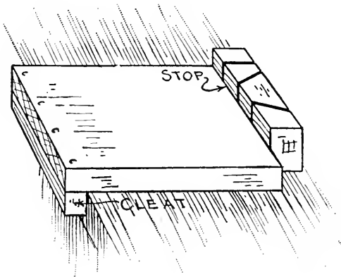
FIG. 60. — Bench-hook.
