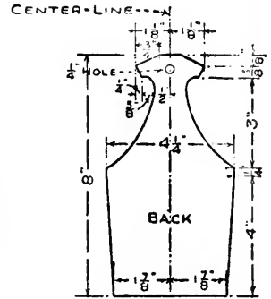
FIG. 115. — Whisk-broom Holder shown in Fig. 108.
