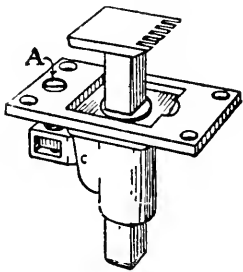
FIG. 15. — An Adjustable Bench-stop.
