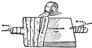
FIG. 323. — The Fixed Condenser is completed by covering it as above with Bicycle Tape. (See Figs. 325 and 326.)
