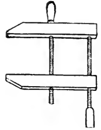
FIG. 40.—Wood Handscrews.
