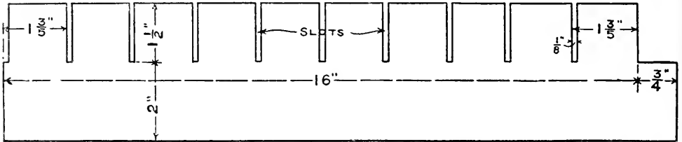
FIG. 353. — Pattern for Cardboard Cylinders.
