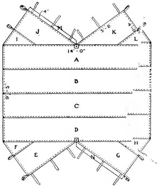
FIG. 420.—Diagram for Making an "A" Tent, 7 feet by 9 feet and 5 inches.
