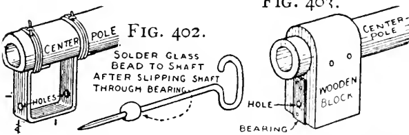
FIGS. 402 and 403. — Propeller Shaft and Two Forms of Shaft Bearing.
