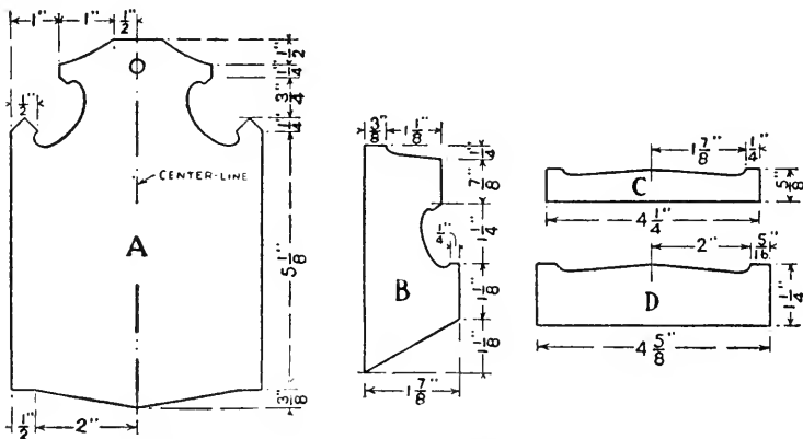
FIG. 249. — Patterns for Kitchen Match-box.
