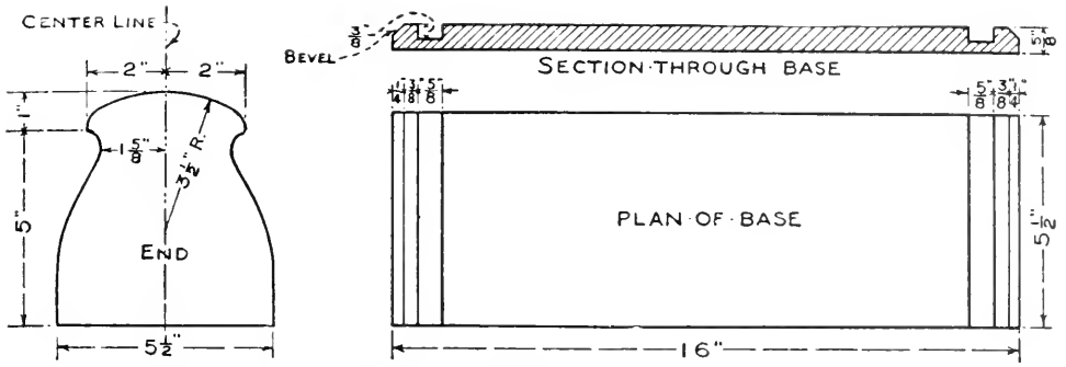
FIG. 119. — Details of Book-rack shown in Fig. 112.
