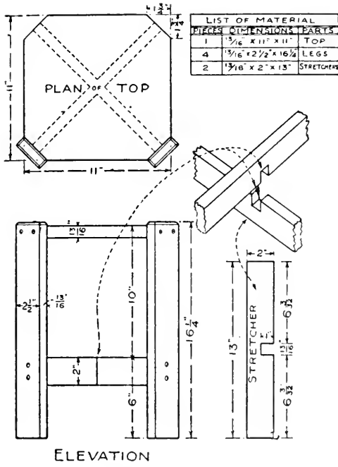
FIG. 126. — Details of Tabouret shown in Fig. 122.
