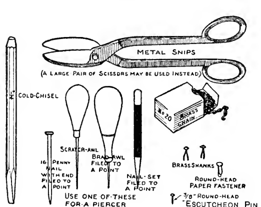
FIG. 278. — Some of the Tools and Materials Required.
