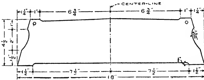
FIG. 117. — Detail of Back of Necktie Rack shown in Fig. 110.
