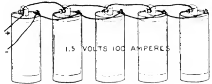
5 DRY-CELLS WIRED IN "PARALLEL" OR "MULTIPLE"
