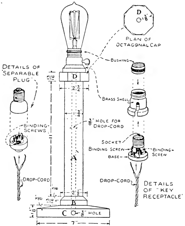
FIG. 146. — Details of Electric Lamp shown in Fig. 142.
