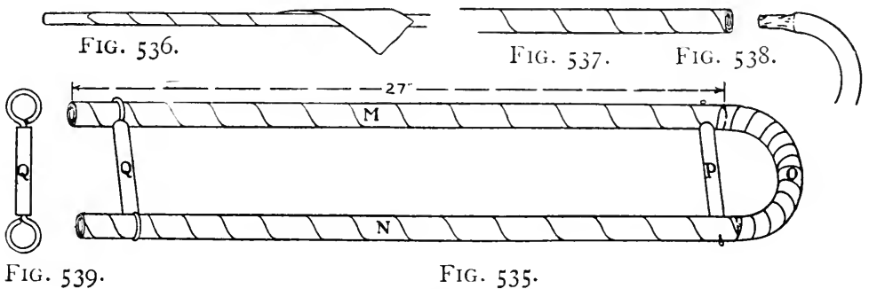
FIGS. 535 to 539. — Details of Trombone Slide.
