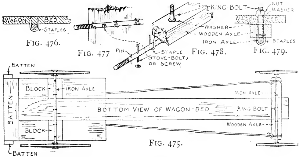
FIG. 475. — Bottom View of Wagon-bed.
