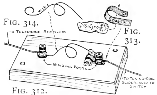
FIG. 312. — A Home-made Silicon Detector. (See Fig. 325.)
