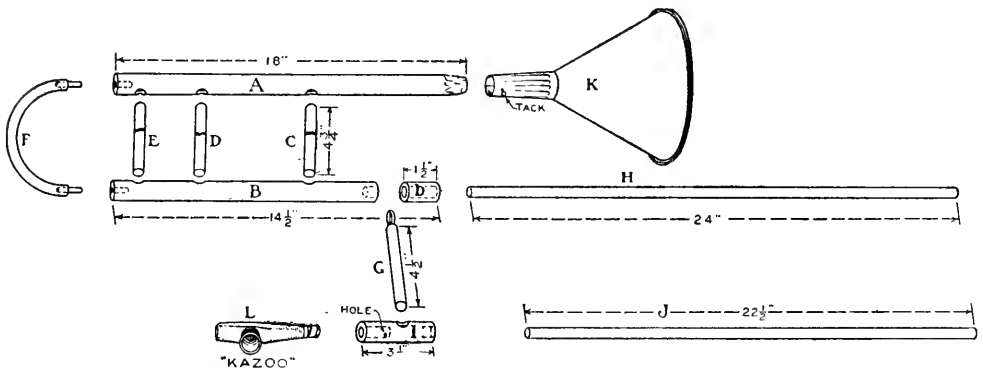
FIG. 534. — Details of the Trombone.
