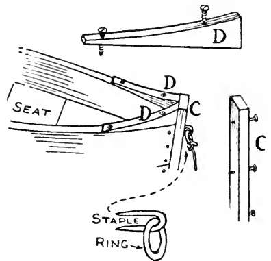
FIG. 452. — Finishing of Bow.
