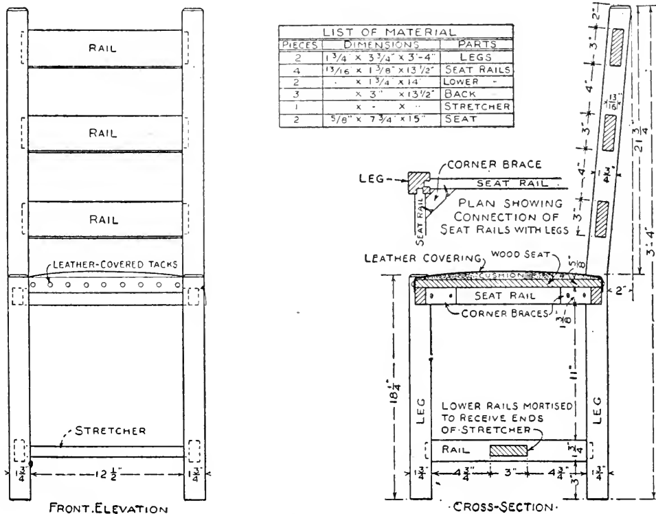
FIG. 144. — Details of Mission Chair shown in Fig. 140.
