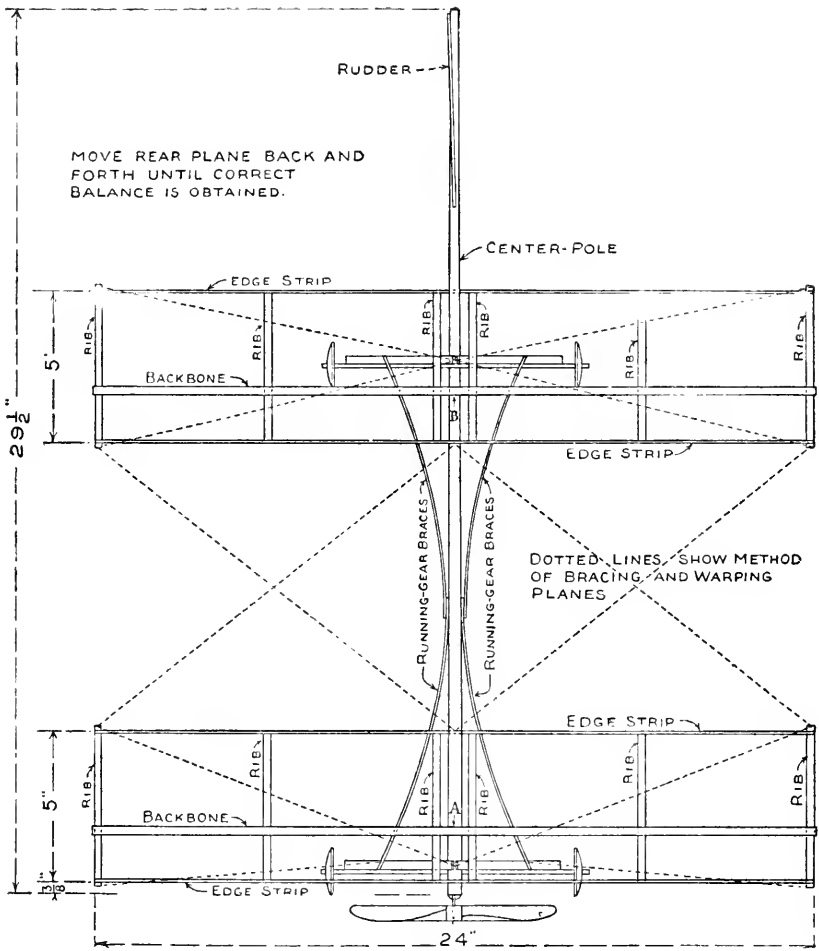
FIG. 398. — Plan or Top View.
