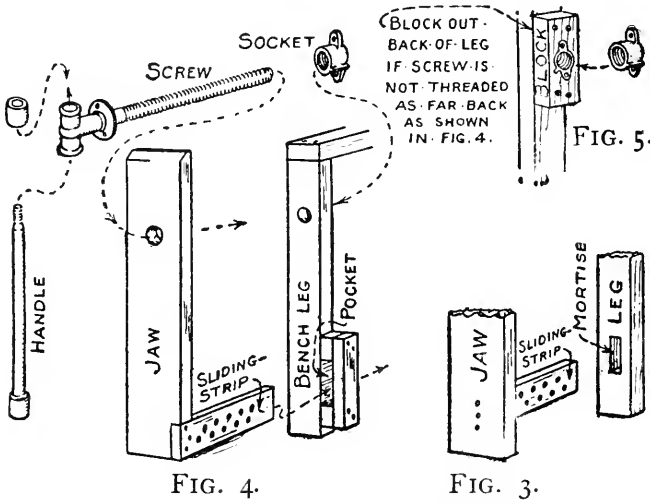
FIGS. 3-5. — Details of the Bench-vise.
