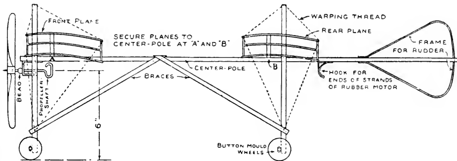
FIG. 400. — Side Elevation of Monoplane Model shown in Fig. 397. (Scale \frac{1}{8}'' = 1'' .)
