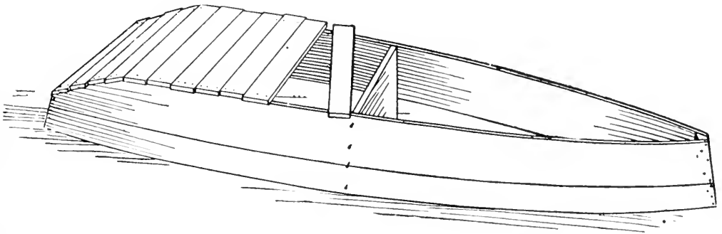
FIG. 450. — How the Bottom Boards are put On.
