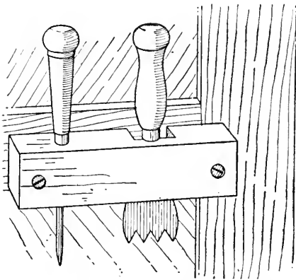
FIG. 169. — Ice-pick and Ice-chisel Rack.
