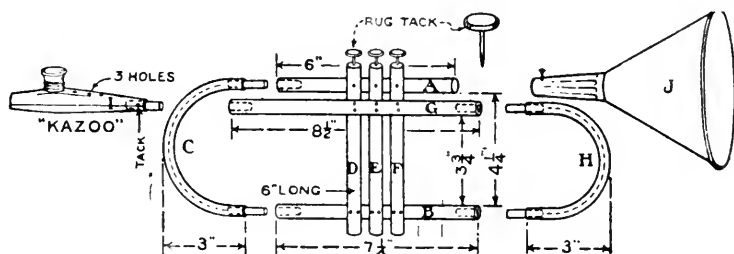
FIG. 533. — Details of Cornet.
