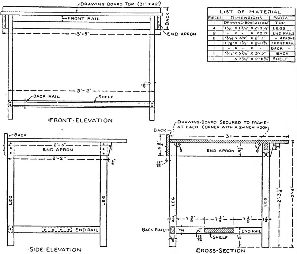
FIG. 147. — Details of Drafting Table shown opposite page 86.
