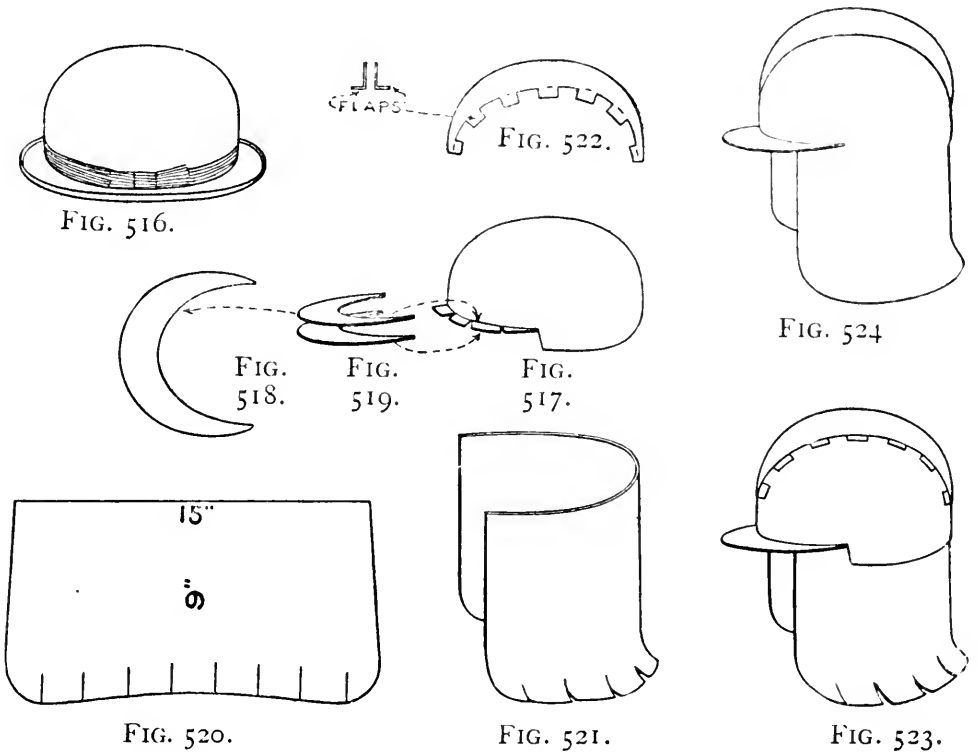
FIGS. 516 to 524. — Details for making the Helmet.
