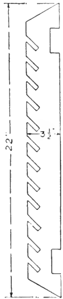
FIG. 154. — Pattern for Side Pieces.
