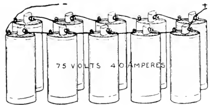
10 DRY-CELLS WIRED IN SERIES-PARALLEL
