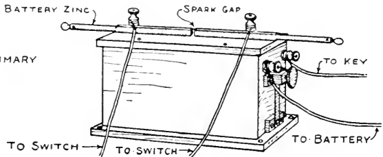
FIG. 328. — How to make a Spark-gap on Coil Box with Battery Zincs.
