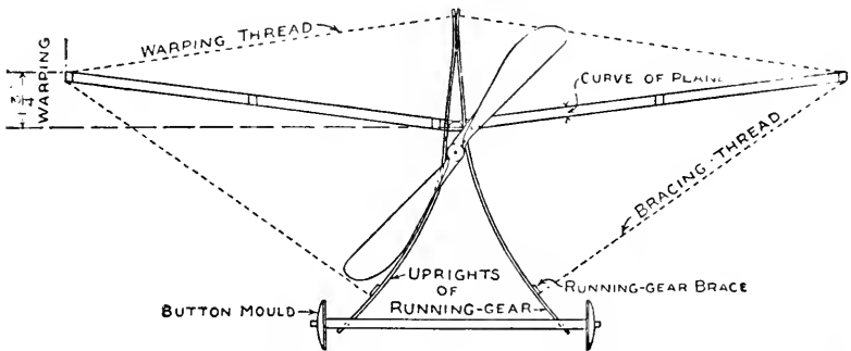
FIG. 399. — Front Elevation of Monoplane Model shown in Fig. 397.
