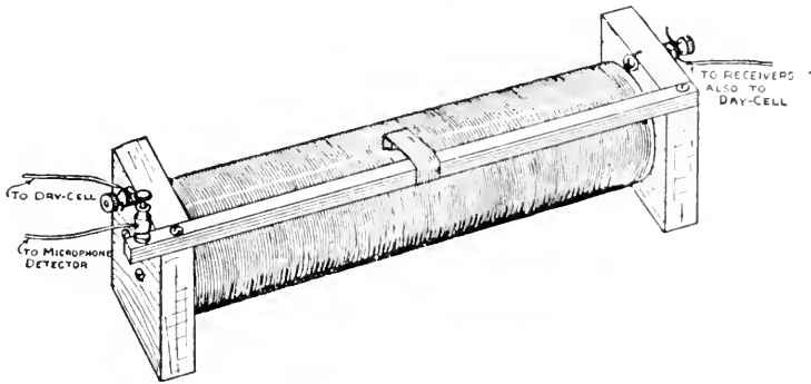
FIG. 324. — A Home-made Potentiometer. (See Fig. 326.)
