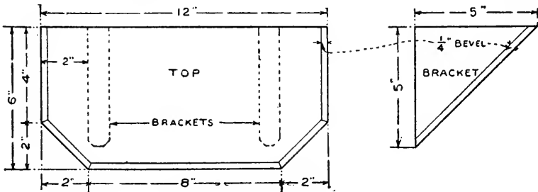
FIG. 116. — Details of Clock-shelf shown in Fig. 109.
