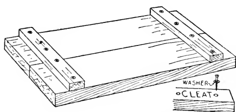
FIG. 85. — The Proper Way to cleat Boards.
