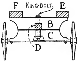
FIG. 460. — The Front Axle.
