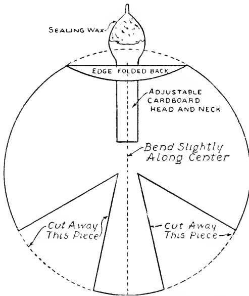
FIG. 382. — A Cardboard Bird Glider.
