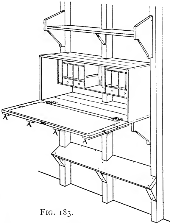
FIG. 183. — The Writing-desk.
