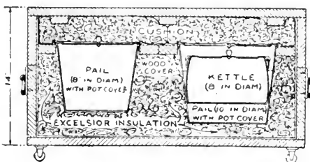
FIG. 150. — Cross-section.
