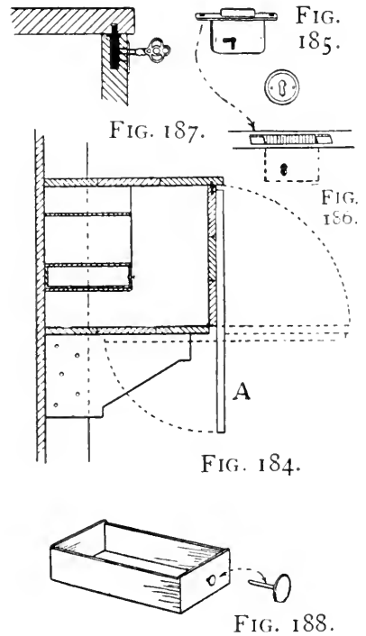
FIG. 185. — A Desk or Cupboard Mortise-lock and Escutcheon for Key-hole.
