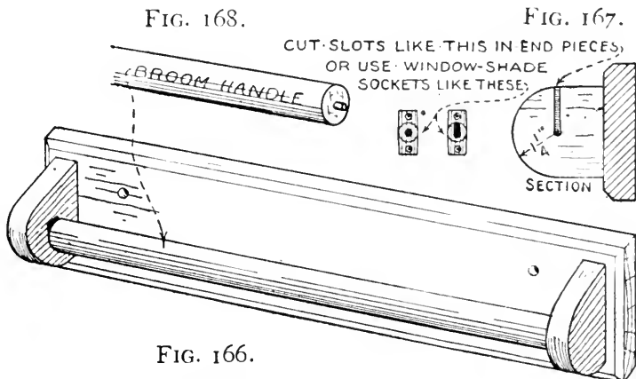
FIG. 166. — Towel-roller.
