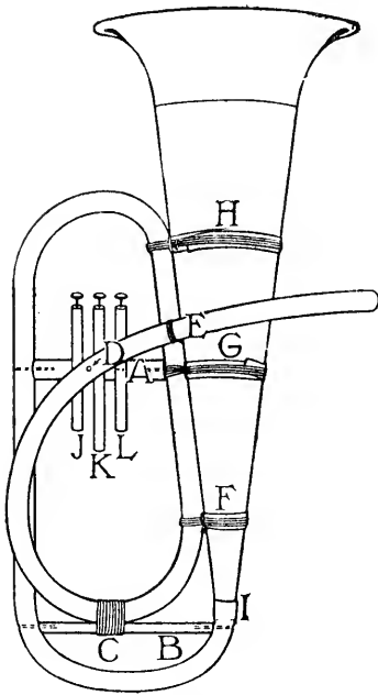
FIG. 540. — Detail of Bass Horn.
