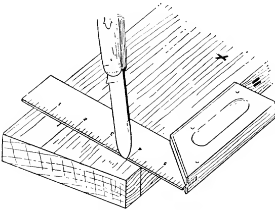
FIG. 67. — Scribing with Knife and Try-square.
