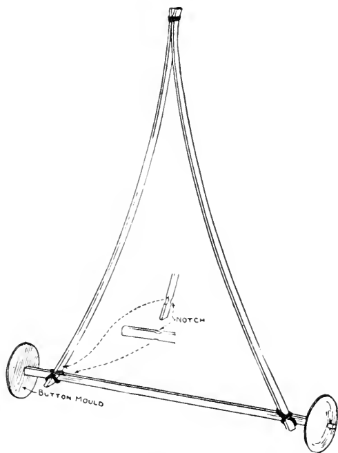
FIG. 401. — Running-gear of Mono-plane shown in Fig. 397.
