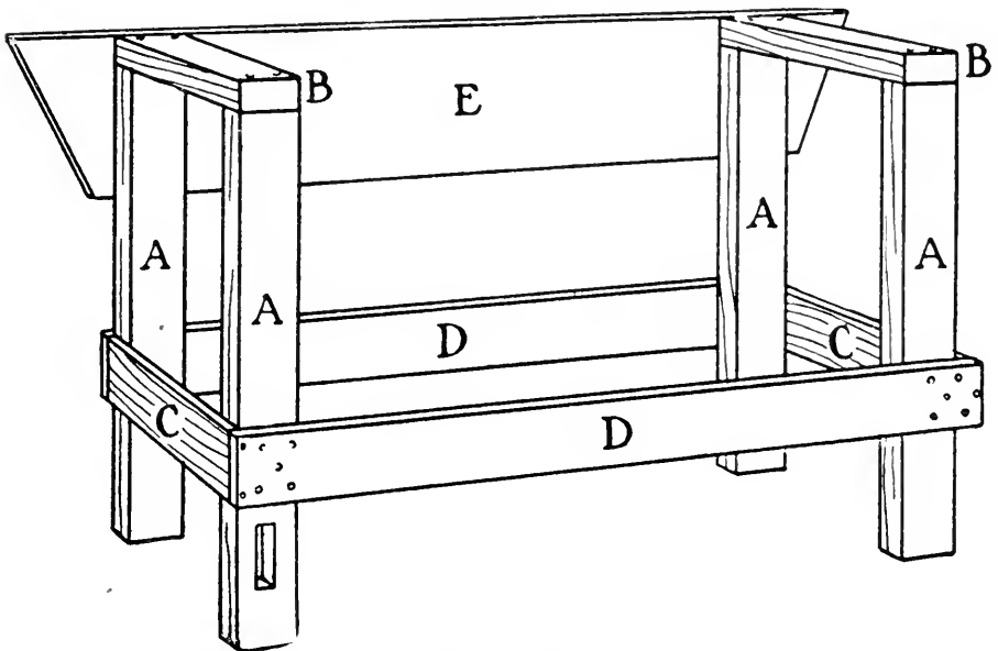
FIG. 2. — Detail of Framework.
