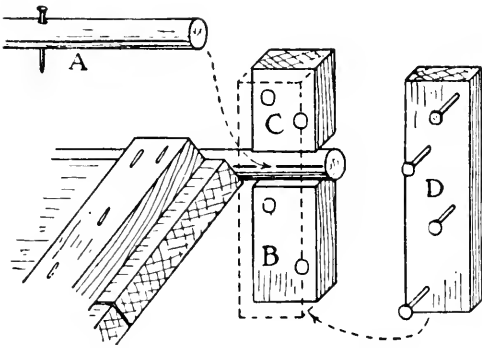
FIG. 510.—Sockets for the Drawbridge.
