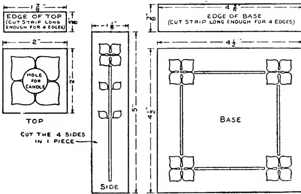
FIG. 292. — Patterns for Brass Pieces of the Candle-stick.
