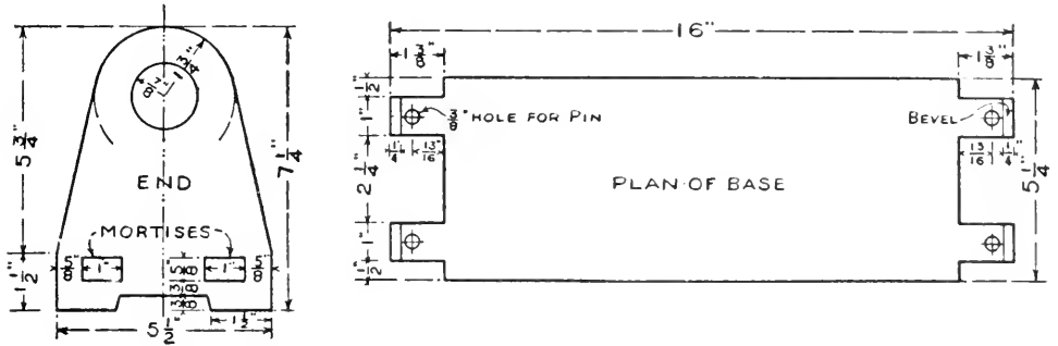
FIG. 120. — Details of Book-rack shown in Fig. 113.
