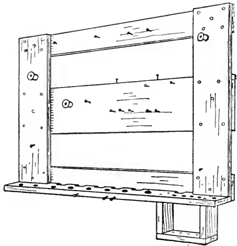
FIG. 46. — A Tool-rack.
