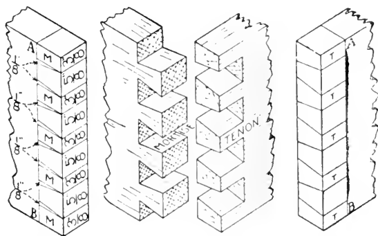
FIG. 81. FIG. 82. FIG. 84. FIG. 83. FIGS. 81-84. — Details of the Dovetail-joint.
