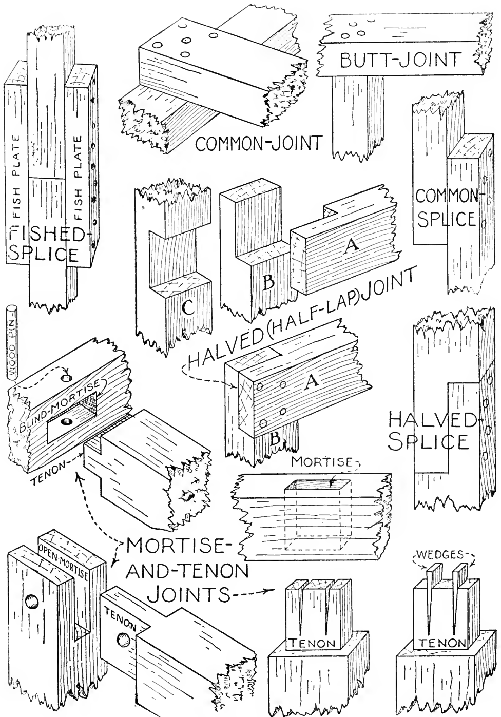
FIG. 74. — Common Forms of Joints and Splices.
