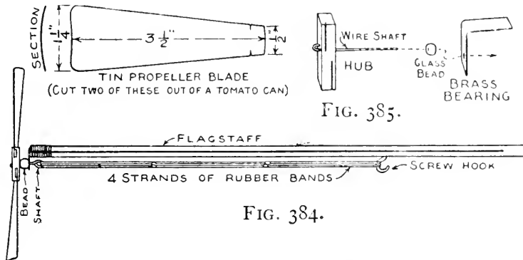
FIG. 384. — Center-pole of Monoplane with Motor in Place. FIG. 385. — Details of Propeller, Shaft and Bearing.
