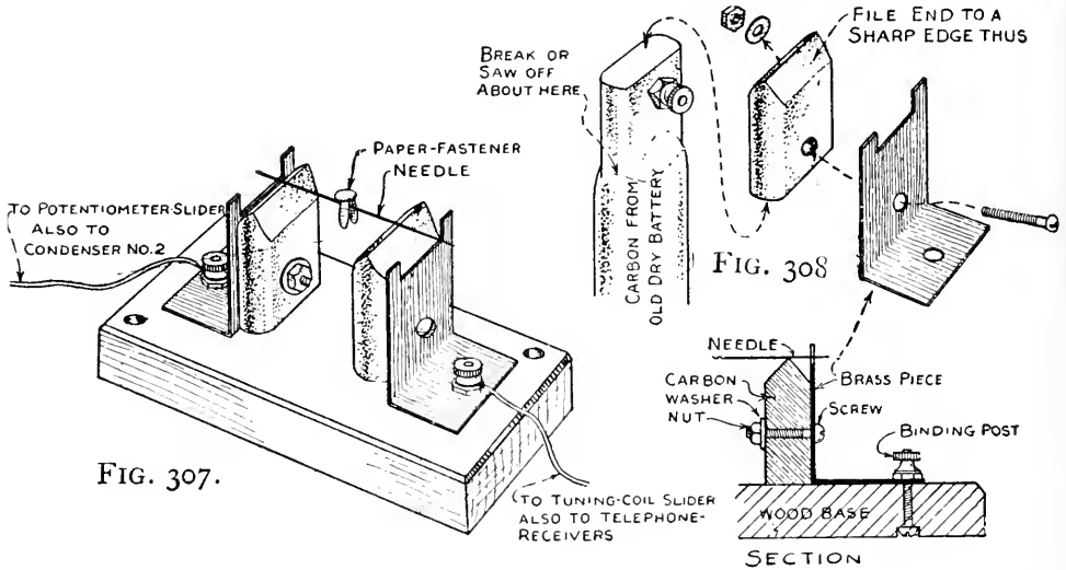
FIG. 307. — A Home-made Microphone Detector. (See Fig. 326.)
