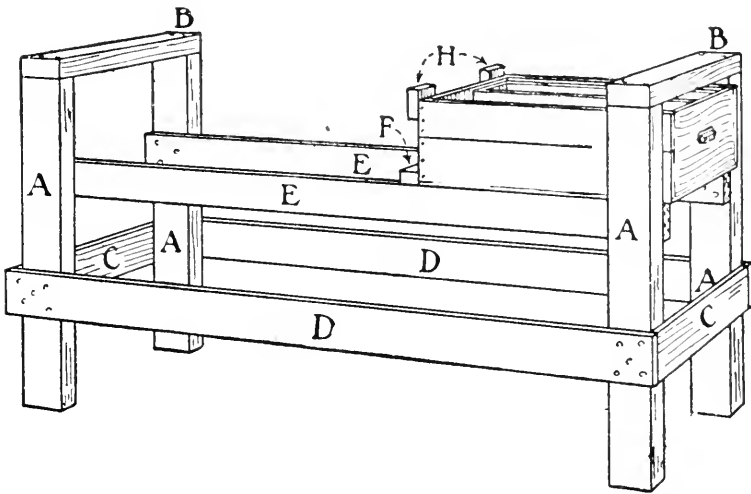
FIG. 7. — Detail of Framework.
