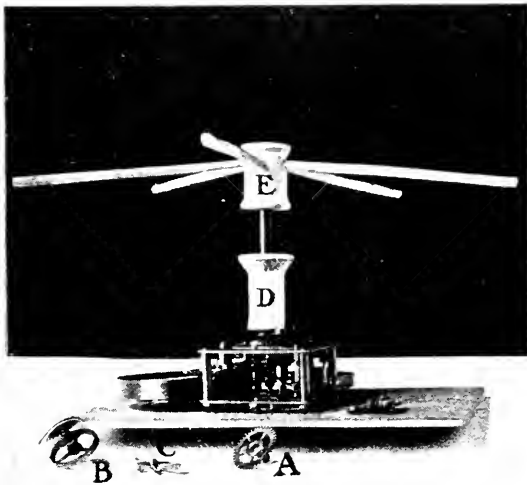
FIG. 254. A CLOCKWORK MOTOR.
