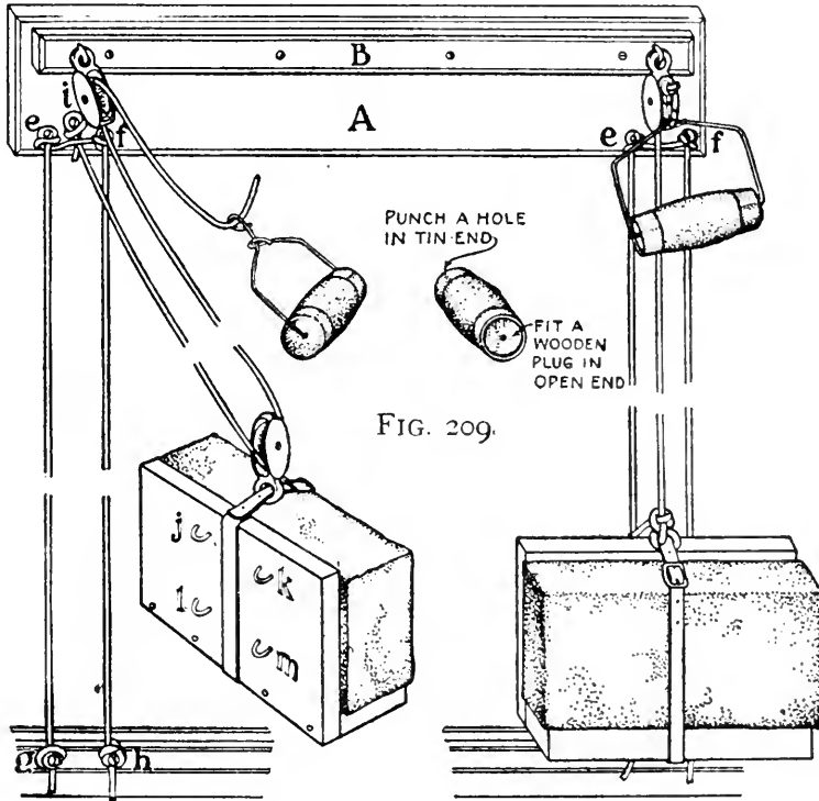
Two-pulley Scheme.
