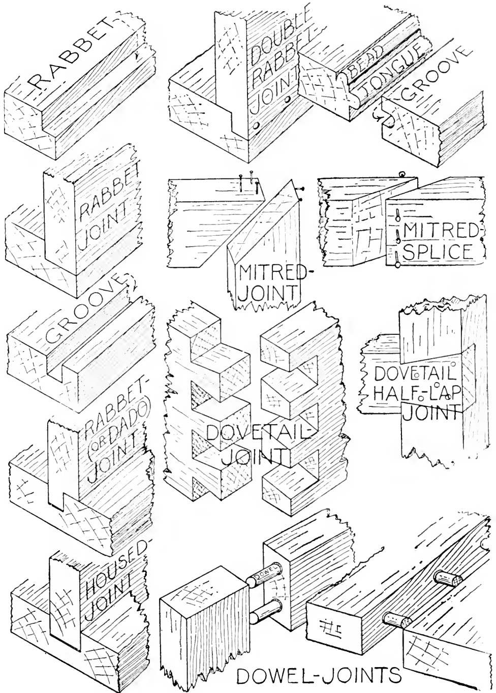
FIG. 75. — Common Forms of Joints and Splices.
