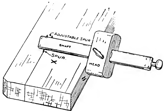
FIG. 68. — Gauging with a Marking-gauge (a Mortise-gauge).
