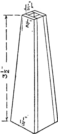
FIG. 235. Pedestal of Center-table.
