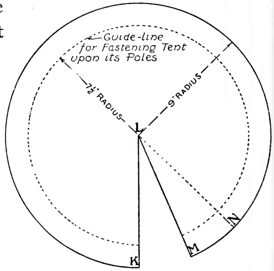
FIG. 259. — Pattern for Tent of Merry-go-round.
