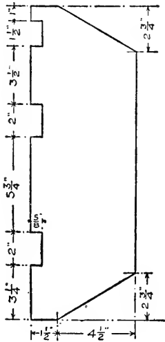
FIG. 159.— Pattern for Side Pieces.
