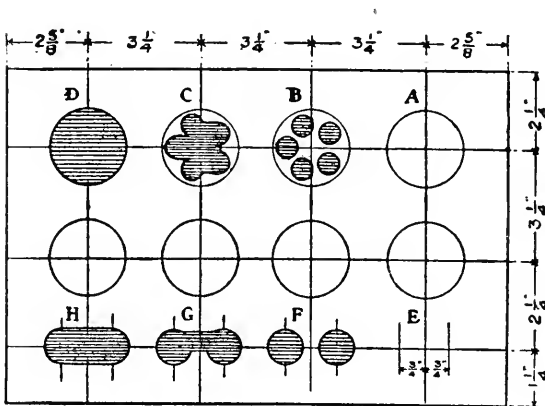
FIG. 156. — Plan of Bottle-rack.
