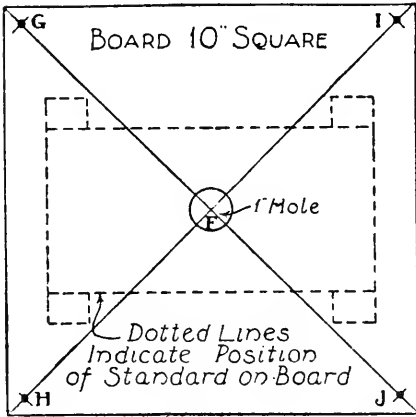
FIG. 258. — Plan of Top of Standard for Merry-go-round.
