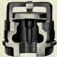
Bottom Attachment for Fig. 1315. Brass Cage Screws onto Bottom Cap
