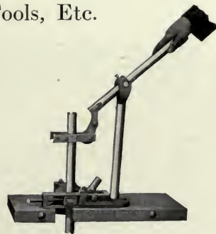
BABCOCK'S PIPE LIFTER AND HOLDER, FIG. 884
