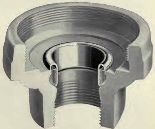
Bottom attachment of a Deming cylinder cut open to show Deming Brass Valve Seat. This clearly illustrates how it is impossible for the seat to "break, chip, flatten, corrode, wear out or become loosened from the cap."
