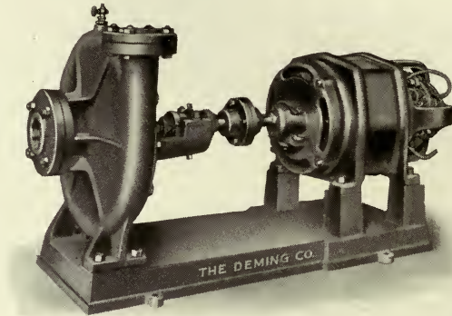
Fig. 599 arranged for direct connected motor drive.
