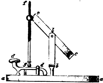
Heliograph von Mance.
