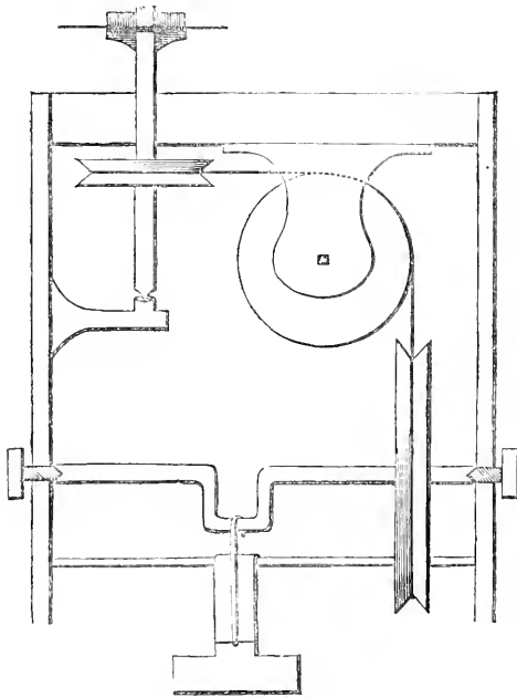
Fig. 14. Section Cutter.
