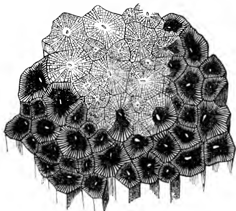
Fig. 10.— Lithostrotion basaltiforme , an abundant compound rugose Coral in the Carboniferous limestone.—The lighter parts show the transverse structure, as seen when the coral is cut for sections.
