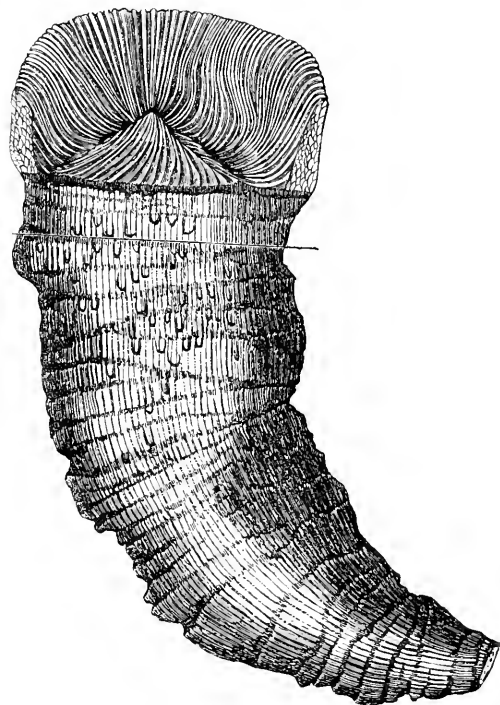
Fig. 12.— Clisiophyllum , a single coral, characteristic of the Carboniferous limestone formation.
