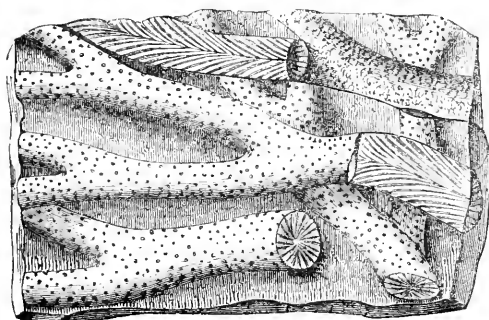
Fig. 31.— Stenopora (or Favosites ) fibrosa , an abundant Silurian Coral.
