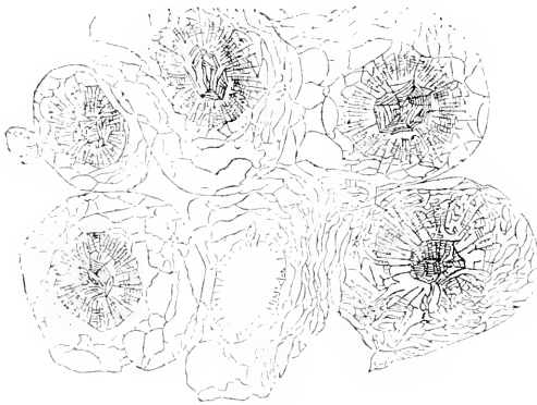
Fig 120.—Transverse section of Lonsdalia rugosa .
