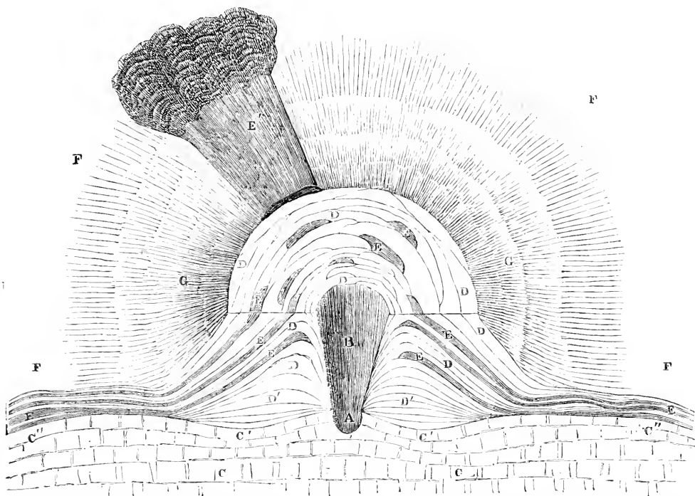
Fig. 136.—Diagrammatic bird's-eye view of a volcanic core. The upper part is supposed to be removed by a horizontal section and one half of the remaining base by another longitudinal one. A, vent; B, chimney; C, basement rock, compressed downwards at C' and upwards at C''; D, ash-beds; E, lava streams, one of which E' is seen to have run down the slopes G of the cone, and spread over the plain F.
