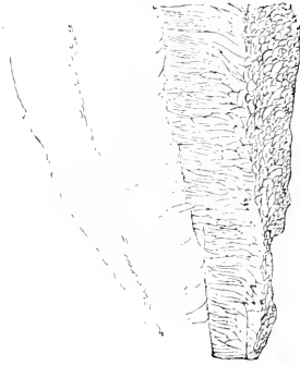
Fig 118.—Vertical section of Fossil Coral ( Koninckophyllum ).
