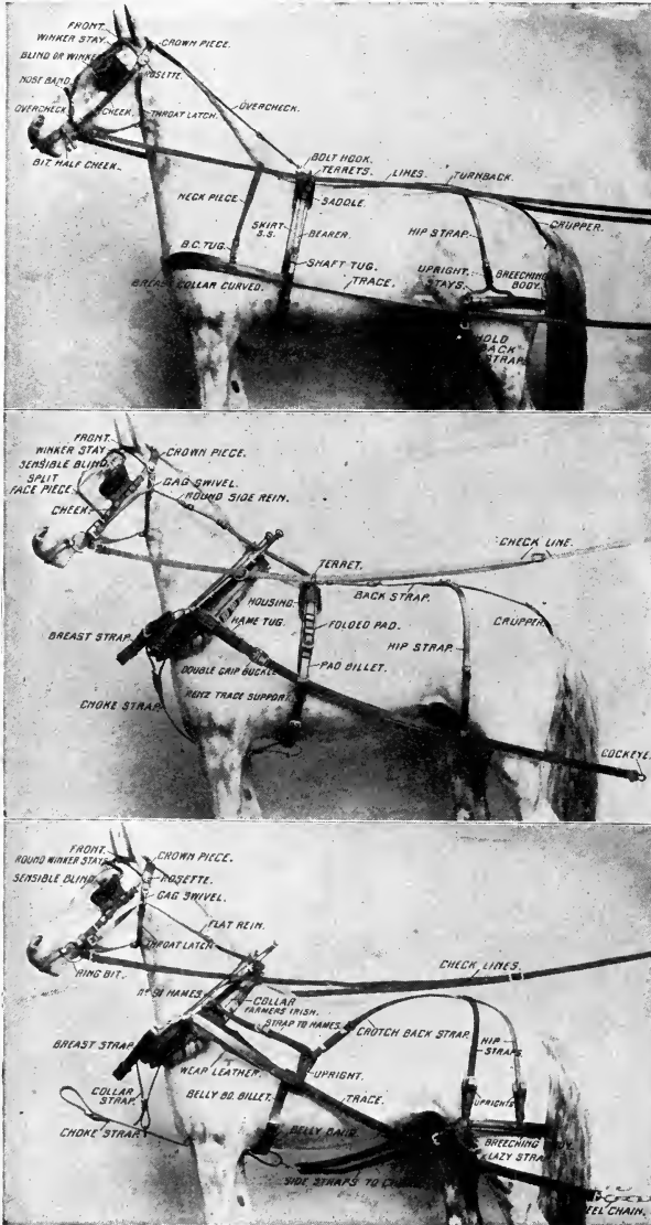
Fig. 1. Typical Harnesses with Principal Parts Named.
