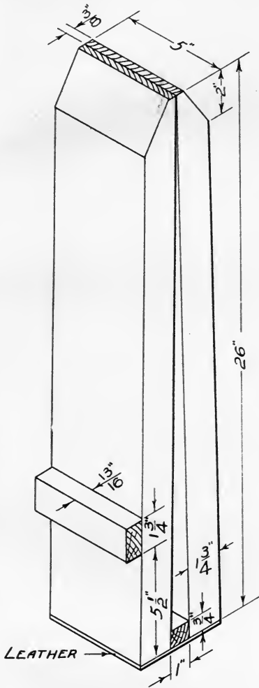
HARNESS STITCHING CLAMP TO BE USED WITH FARM SHOP WORKBENCH VISE
