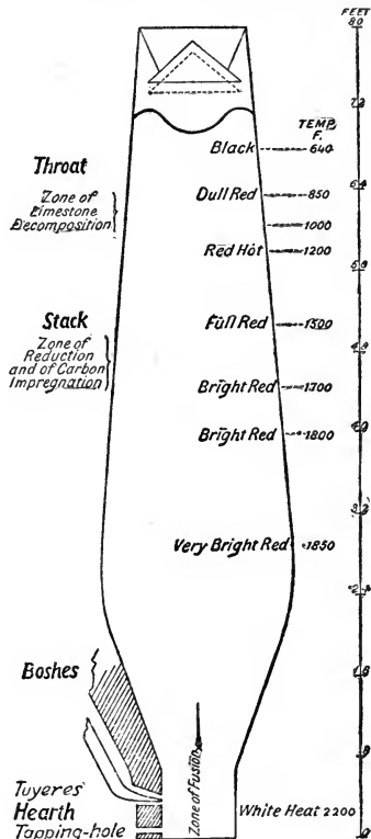
DIAGRAM OF A MODERN BLAST-FURNACE.
