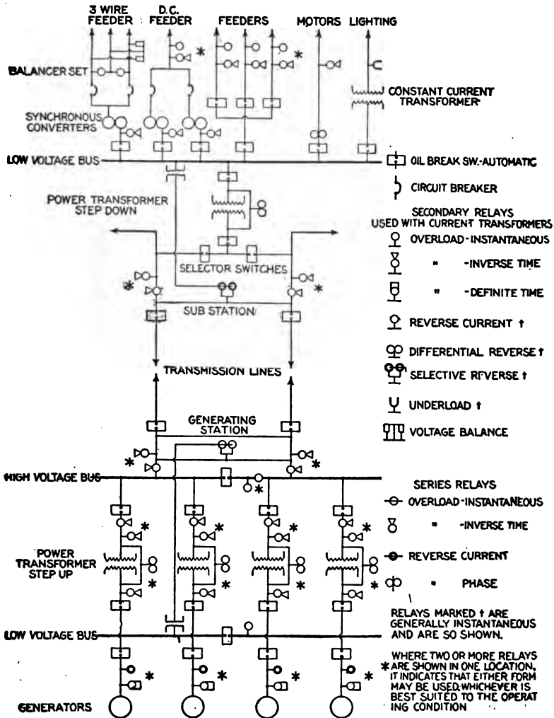
FIG. 2,323.—Diagram of modern power house wiring and buses showing location of relays.
