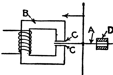
Figs. 2,505 and 2,506. —Plan and elevation of shielded pole type of induction instrument.
