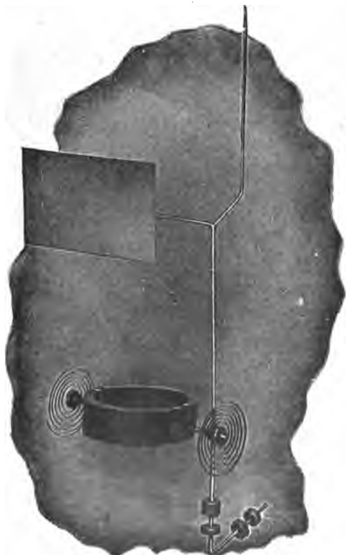
FIG. 2,517. —Moving element of Keystone dynamometer instrument. The illustration shows the movable coil, pointer, aluminum air vane for damping the oscillations, controlling springs, and counter weights.
