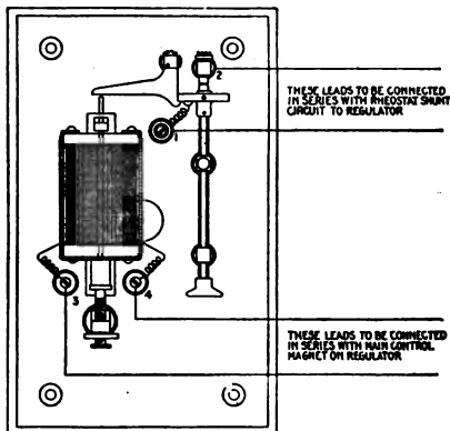
FIG 2,434.—Diagram of connections of General Electric high voltage cut out relay (form 2) for voltage regulators. Its use in connection with the regulator protects the system from any sudden rise in voltage due to some accident to the regulator which might cause the relay contacts to stick, thus producing full field on the exciter. In construction, the control magnet is connected in series with the alternating current control magnet on the regulator and the contacts are connected in series with the rheostat shunt circuit. Then, should the voltage rise beyond a certain value, predetermined by the setting of the thumb screw supporting the plunger of the control magnet, the contacts of the relay are tripped open which, by inserting all the resistance in the exciter field, reduces the exciter voltage which in turn reduces the alternating current voltage. This relay has to be reset by hand.
