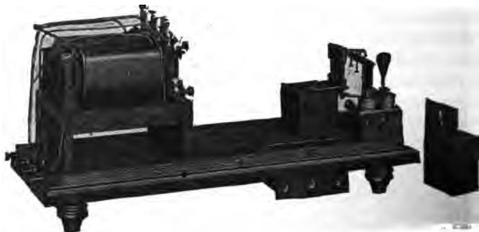
FIG. 2,601. —General Electric moving coil oecillograph with case removed, showing interior construction and arrangement of parts. The oscillograph is furnished complete with a three element electromagnet galvanometer, optical system, shutter and shutter operating mechanism, film driving motor and cone pulleys, photographic and tracing attachments, 6 film holders, and the following repair parts, for vibrators: 6 extra suspension strips; 6 vibrator mirrors; 1 box gold leaf fuses; 1 bottle mirror cement; 1 bottle damping liquid.
