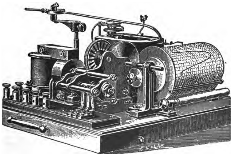
Fig. 2,598. —View of Hospitalier ondograph. In operation, a long pivoted pointer carrying a pen and actuated by electromagnets, records on a revolving drum a wave form representing the alternating current, pressure or current wave.
