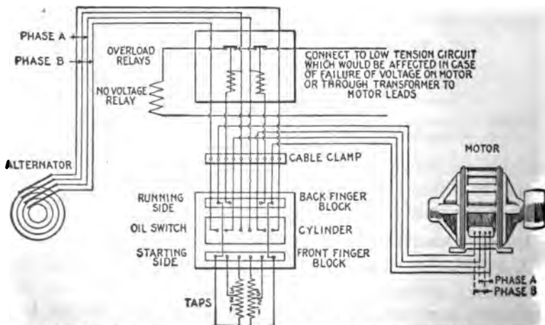
FIG. 2,465. —Diagram of connections of General Electric two phase starting compensator with no voltage release and overload relays for 1,040 to 2,500 volt circuits.
