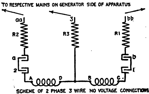
SCHEME OF 2 PHASE 3 WIRE NO VOLTAGE CONNECTIONS
