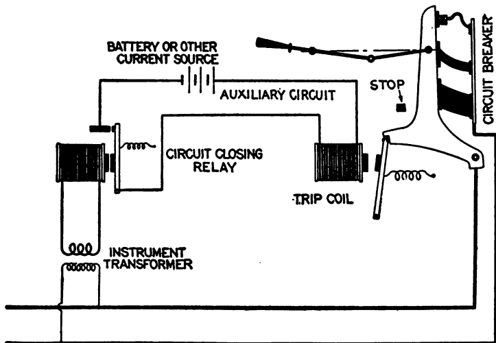
FIG. 2,279.—Diagram illustrating the operation of a circuit closing relay. When the predetermined abnormal condition is reached in the main circuit, the relay closes the auxiliary circuit, thus energizing the trip coil and opening the breaker.
