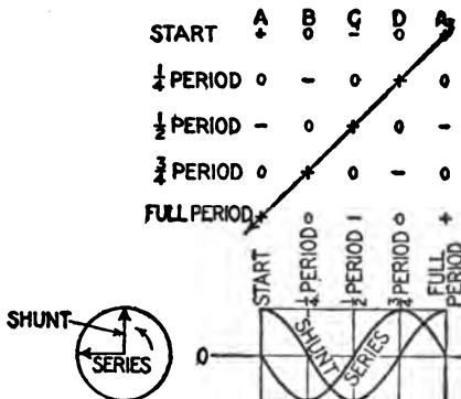
Figs. 2,531 to 2,533. —Diagram of electro-magnetic circuit of Westinghouse induction type watt hour meter, and diagram showing rotation of field. The dotted lines show the main paths of the magnetic flux produced by the two windings, the directions, however, are constantly reversing owing to the alternations of the current in the coils. Denoting the shunt and series pole tips by the letters as shown, a clear statement of the relation of the fields for each quarter period may be given. The signs + and - represent the instantaneous values of the poles indicated. Thus, at one instant the shunt pole tips A, C, and A 1 are maximum +, -, and +, respectively because the instantaneous value of the current is maximum, while the value of the series flux is zero. At \frac{1}{4} period later the shunt current is zero, giving zero magnetic pressure at the pole tips, while the series current has reached a maximum value, giving maximum - and + at the pole tips B and D. At the next \frac{1}{4} period the shunt current is again maximum, but in a direction opposite to what it was at the beginning, making the pole tips A, C, and A 1 +, -, and +, respectively, while the series current again is zero, etc., the values for the complete cycle being given in fig. 2,533. It will be observed from the table that both the + and - signs move constantly in the direction from A 1 to A, indicating a shifting of the field in this direction, the process being repeated during each cycle.
