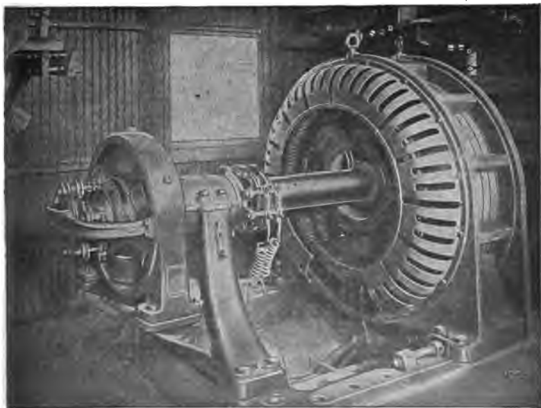
FIG. 2,479. —General Electric 400 kw., 550 volt, 600 R.P.M., synchronous condenser with direct connected exciter installed in sub-station No. 1 of the Colorado Light & Power Co., Cripple Creek, Colo. The machine is designed for alternating current starting by means of a compensator. The field is provided with a standard synchronous motor winding, and, in addition, an amortisseur winding which assists in starting and serves as a damping device to minimize hunting.
