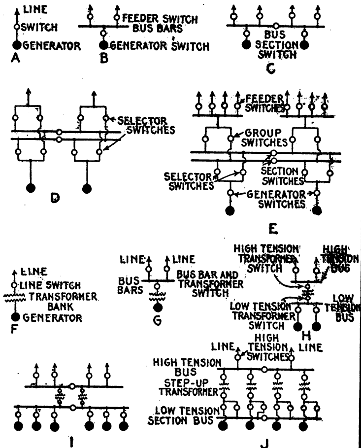
cs. 2,645 and 2,646.—Diagrams illustrating general principles of switchboard connections.
