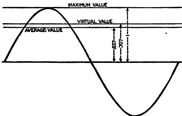
FIG. 2,491. —Line curve of alternating current, illustrating various current or pressure values. The virtual value, or .707 \times maximum value, is the value indicated by an ammeter or voltmeter. Thus, if the maximum value of the current be 100 volts, the virtual value as indicated by an ammeter is 100 \times .707 = 70.7 amperes.
