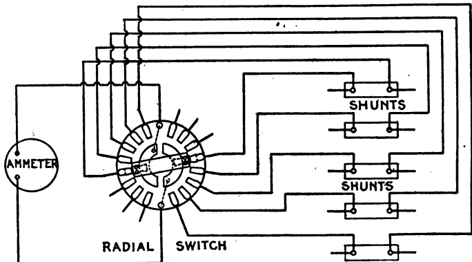
FIG. 2,670.—Wiring diagram for Crouse-Hinds radial ammeter switch as illustrated in fig. 2,668. The switch proper is on the rear of the switchboard, and the hand wheel dial and indicator on the front.
