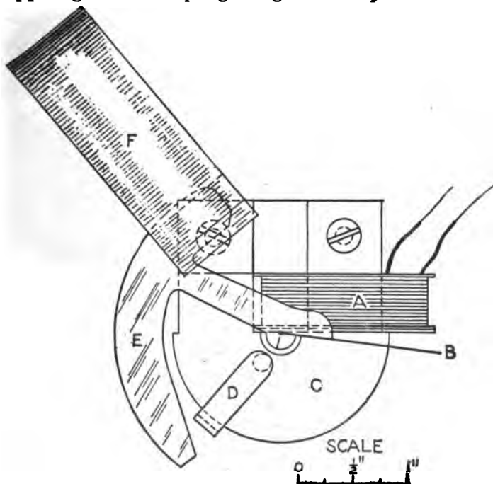
FIG. 2,507. —Diagram showing construction and operation of Hoskins instrument. It is of the modified induction type in which the torque is produced from the direct repulsion between a primary and a secondary, or induced current. As shown in the diagram, the instrument embodies the principle of a short circuited transformer, consisting of a primary or exciting coil A, a secondary or closed coil B, linked in inductive relation to the primary by a laminated iron core C, constructed to give a completely closed magnetic circuit, that is, without air gap. The secondary is so mounted with respect to the primary as to have a movement under the influence of their mutual repulsion when the primary is traversed by an alternating current. This movement of the secondary B is opposed by a spiral spring, so that the extent of movement will be dependent upon and will indicate the strength of the primary current. To increase the sensitiveness of the instrument and also to adjust the contour of the scale, an adjustable secondary D, which has an attraction effect upon the coil B, is provided upon the core. The effect of this coil is inversely proportional to its distance from the end of the swing of the coil B. The vane, E, which is a part of the stamping B, is adjusted to swing freely and with a large amount of clearance, between the poles of a permanent magnet F, which acts as a damper on the oscillation of the moving element, but does not cause any friction or affect the accuracy of the calibration. The primary, like that of a transformer, is an independent electrical circuit and may be highly insulated. This meter will withstand several hundred per cent. overload for some time because of the very high value of the self-induction and the fact that the controlling spring is not in the circuit and therefore cannot burn off.
