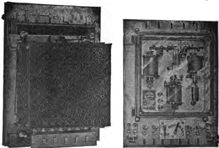
FIGS. 2,454 and 2,455. —Front and rear views of General Electric automatic voltage regulator. The regulator has a direct current control magnet, an alternating current control magnet, and a relay. The direct current control magnet is connected to the exciter bus bars. This magnet has a fixed stop core in the bottom and a movable core in the top which is attached to a pivoted lever having at the opposite end a flexible contact pulled downward by four spiral springs. For clearness, however, only one spring is shown in the figure. Opposite the direct current control magnet is the alternating current control magnet which has a pressure winding connected by means of a pressure transformer to the alternator or bus bars. There is an adjustable compensating winding on the alternating current magnet connected through a current transformer to the principal lighting feeder. The object of this winding is to raise the voltage of the alternating current bus bars as the load increases. The alternating current control magnet has a movable core and a lever and contacts similar to those of the direct current control magnet, and the two combined produce what is known as the "floating main contacts." The relay consists of a U shaped magnet core having a differential winding and a pivoted armature controlling the contacts which open and close the shunt circuit across the exciter field rheostat. One of the differential windings of the relay is permanently connected across the exciter bus bars and tends to keep the contacts open; the other winding is connected to the exciter bus bars through the floating main contacts and when the latter are closed, neutralizes the effect of the first winding and allows the relay contacts to short circuit the exciter field rheostat. Condensers are connected across the relay contacts to prevent severe arcing and possible injury.
