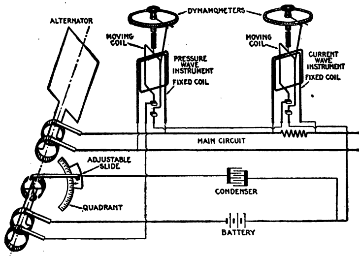
FIG. 2,501.—Modified four part commutator method of wave form measurement (Duncan's modification). By this method one contact maker can be used for any number of waves having the same frequency. Electro-dynamometers are used and the connections are made as here shown. The moving coils are connected in series to the contact maker, and the fixed coils are connected to the various sources to be investigated, then the deflection will be steady and by calibration with direct current can be made to read directly in volts.
