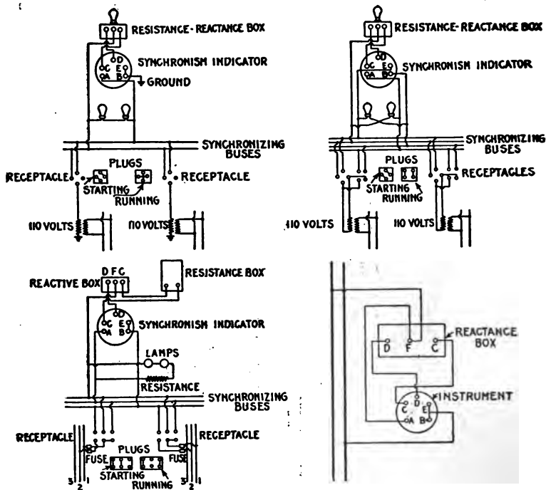
FIGS. 2,573 TO 2,576. —Connections of General Electric synchronism indicator. Fig. 2,573, connections with grounded secondaries on pressure transformers; fig. 2,574, connections with ungrounded secondaries on pressure transformers; fig. 2,575, connections for 200 to 240 volt circuits, with six point receptacles; fig. 2,576, connections for checking location of needle. The various letters referred to in the diagrams will be found marked on the ends of the instrument studs and back of reactance coil box. It is important that the instrument be connected in circuit in the proper manner so that the needle will come to the mark on the upper part of the scale when synchronism is obtained. In case the pointer become moved or a change in its position be necessary, it is advisable to make a check on the indication before relocating the needle. This test can be made as follows: Connect together (fig. 2,573) studs marked B and E and connect stud A to terminal F on the external reactance box. When these connections are made, the instrument can be connected to a single phase circuit of normal voltage and if the instrument be correct, the pointer will stand vertically at the point of synchronism. If it do not, the needle can be moved and should be fastened in the correct position. The synchronizing lamps when connected as illustrated in the diagrams, show dark when synchronism is reached. This is the only connection possible when grounded secondaries are used, as in fig. 2,573, and for the high voltage indicators when used as in fig. 2,575, but with ungrounded secondaries (fig. 2,574) the lamps may be connected as indicated, when they will show bright at the moment of synchronism. The connections to the synchronism indicator remain the same as before.
