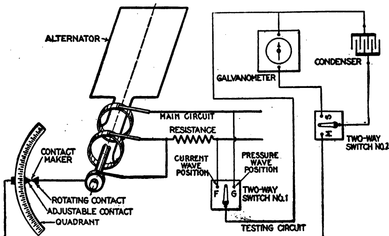
FIG. 2,889.—Diagram illustrating Joubert's step by step method of wave form measurement.
