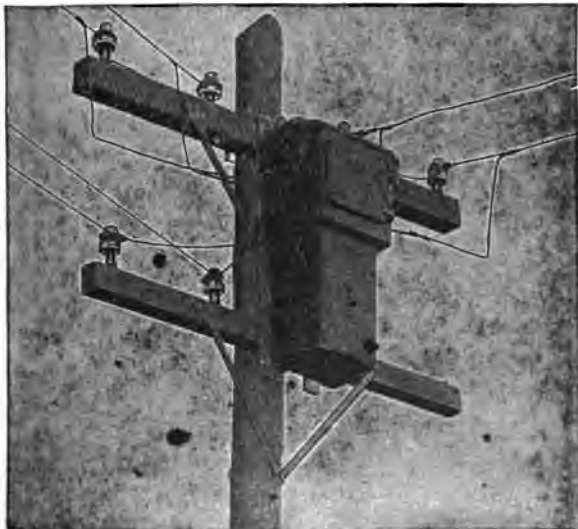
FIG. 2 44 J).—General Electric pole type regulator in service; its construction is shown in fig. 2,450.
