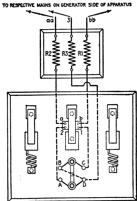
2 PHASE 3 WIRE NO VOLTAGE CONNECTIONS
