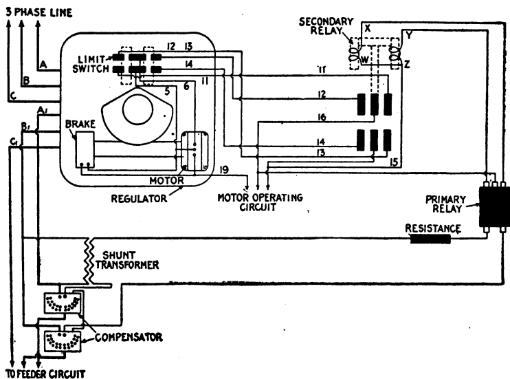
FIG. 2,480.—Diagram of connections of automatic induction regulator and accessory apparatus on three phase feeder circuit.
