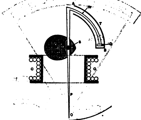
FIG. 2,497. —One form of plunger instrument as made by Siemens. It has gravity control is dead beat, and is shielded from external magnetic influence. The moving system consists of a thin soft iron pear shaped plate I pivoted on a horizontal spindle S running in jewelled centers. To this spindle S is also attached a light pointer P and a light wire W, bent as shown, and carrying a light piston D, which works in a curved air tube T. This tube T is closed at the end B but fully open at the other, A, and constitutes the air damping device for making the instrument dead beat.
