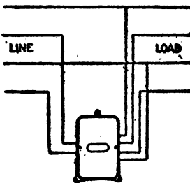
Figs. 2,538 to 2,541. —Connections of Fort Wayne multi-phase watt hour meters (type k—forms MAB and MAK), for 100–625 volt circuits, 5–150 amperes. Fig. 2,538 two and three phase, three wire circuit, 25–36 cycles; fig. 2,539 two and three phase, 3 wire circuit, 36 cycles and above; fig. 2,540, two phase 4 wire circuit, 25–36 cycles; fig. 2,541 two phase, 4 wire circuit 36 cycles and above.
