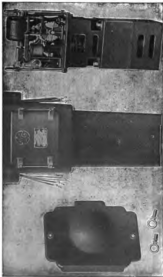
FIGS. 2,439 TO 2,443. —General Electric poise type regulator removed from tank. It consists essentially of a primary and secondary coil, operating motor, and voltage relay mechanism. The regulator and mechanism is suspended in a cast iron tank, the lower part, containing the regulator core and coils, being filled with oil. The leads for the regulator are brought out at the upper part of the tank. The outgoing leads are compressed into bushings and connected to the leads of the regulator by means of terminals. The arrangements being such that the regulator with mechanism can be removed from the tank without difficulty. Besides the cover, the tank is also provided with a hinged door on the front side so as to give access to the mechanism. The door is provided with a gasket and the construction is practically ruin and dust proof. However as there is always danger of the door not being clamped down perfectly, thus making it possible for water to enter the tank, a pocket has been provided inside the tank and underneath the door to collect the water. Capacity up to 2.3 kw., to control 2,300 volts, 60 cycle, 10 ampere feeders, and for a voltage range of 10 per cent, above or below normal, the operating motor and relay being designed for 110 or 220 volts. No provision is made for line drop compensation, although this can be obtained by installing a current transformer and a line drop compensator externally to the regulator.
