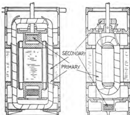
Figs. 2.444 to 2.446. —Sectional views of General Electric pole type regulator winding and core. The secondary core has only two slots containing a single coil, while the rotor or primary core has four slots. Two of these slots are occupied by a single primary coil, and the two circular slots in quadrature thereto contain the compensating or short circuit winding. This winding also serves to hold the primary punchings together, and it consists of two copper rods riveted to the two cast brass flanges. The secondary coil is form wound, while the primary coil is wound directly on the core. The rotor flanges, both top and bottom, are provided with discs which are turned in alignment with the punchings, and these discs bear against the top and bottom flanges between which the secondary punchings are clamped. These secondary flanges are also turned in alignment with the secondary punchings, so that an even air gap between the primary and the secondary is assured. The secondary coil is wound with an opening in the upper horizontal part which affords passage for the operating shaft of the rotor. A bearing for this shaft is provided in the table which supports the mechanism and from which the regulator is suspended. Flexible leads are brought out from the rotor and twisted around the shaft as in standard regulator practice. The regulator being two pole, the rotor is turned through an angle of 180 deg. to obtain the full range of the regulator.
