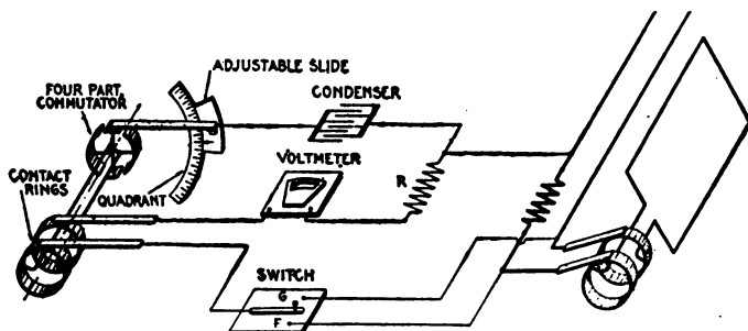
FIG. 2,500.—Four part commutator method of wave form measurement. The contact device consists of two slip rings and a four part commutator. One slip ring is connected to one terminal of the source, the other to the voltmeter, and the commutator to the condenser. By adjusting R when a known direct current pressure is impressed across the terminals, the voltmeter can be rendered direct reading.
