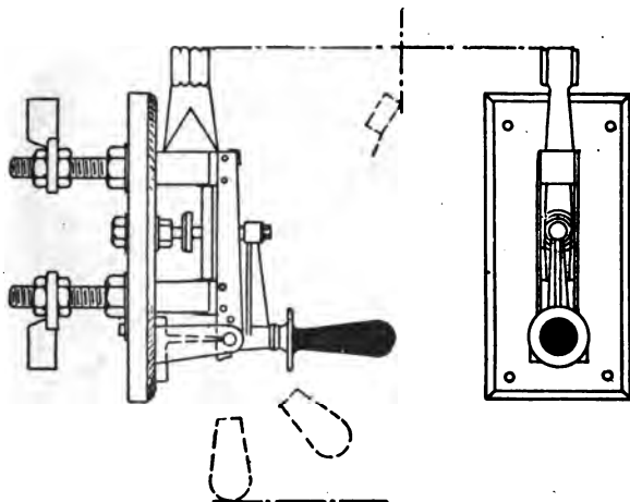
FIG. 2.247.—Thermal overload circuit breaker. In construction two contact blocks are fixed rigidly to, but insulated from, the switch arm. They are connected electrically by two parallel strips of suitable metal, each fitted with a steel catch piece. When the switch is closed the strips are sprung apart over a fixed catch, and the full rated current does not release the catch. Overload causes the strips to move apart, and the circuit breaker flies off under the action of a spring.
