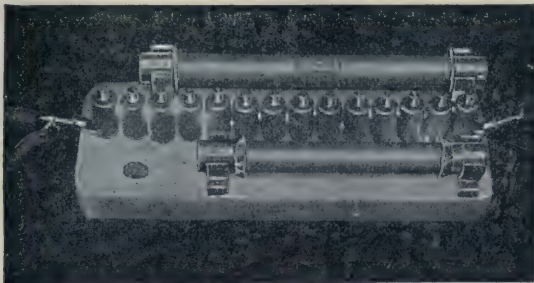
FIG. 2,352. —General Electric 2,200 volt arrester in the act of discharging, and shunting the line current. The figure shows an actual discharge taking place. It will be seen that the heavy line current passes across only four of the gaps, and then goes through the resistance rods; while the static discharge passes straight across the entire series of thirteen gaps. When the gaps of an arrester are shunted by even a low resistance, discharges of very high frequency find it relatively difficult to pass through the resistance rods, owing to the impedance of the rods, but comparatively easy to pass across all the gaps, owing to the capacity effect in breaking down the gaps. The higher the frequency, the more pronounced is this effect, hence the discharges select different paths through gaps and resistances depending upon the frequency. By frequency is meant, not the frequency of the line current but the lightning frequency, which may run into hundreds of thousands, or into millions of cycles. The equivalent needle gap for this arrester is shown by tests to be nearly the same for all frequencies and quantities of discharge; that is, the arrester is equally responsive to all frequencies.
