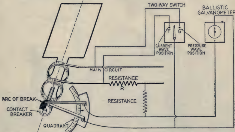
FIG. 2,596. —Diagram illustrating zero method of wave measurement with contact breaker . The voltage of the battery must be at least as great as the maximum pressure to be measured and must be kept constant.
