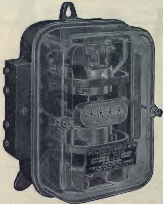
FIG. 2,537. —Fort Wayne multiphase induction watt hour meter. The construction of the mechanism is essentially two single phase motor elements , one at the bottom of the meter in a suitable position, the other inverted and placed at the top of the meter. Each element acts on a separate cup , but both cups are mounted on a single shaft so that the registration is due to the resultant torque of the two elements. The meter is provided with three supporting lugs, the one at the top being keyholed and one of the bottom two, slotted to facilitate leveling. The registering mechanism is mounted on a cast iron bracket at the middle of the meter between the two motor elements. The supporting bracket is attached to the meter base by two screws and aligned by two dowel pins. The register is of the four dial type, reading in kilowatt hours. Each division of the right hand circle, or that passed over by the most rapidly moving pointer, equals one kilowatt hour in meters without a dial constant. In meters of larger capacities, dial constants of 10, 100 and 1,000 are used, in which case it is only necessary to add one, two or three ciphers to the observed reading.
