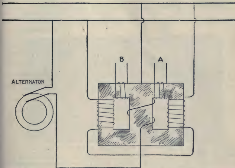
FIG. 2,322.—Differential relay transformer and reverse current circuit breaker discriminating device. A differential relay is one whose electromagnet has two windings . In normal working these oppose and neutralize one another. Should, however, either winding become stronger or weaker than the other, the balance is upset, the magnet is energized, and the relay comes into operation. A modification of such a relay for alternating current is here shown, from which it will be seen that when the currents are as indicated, the circuit A has the larger pressure induced in it, whereas, should the main current reverse with reference to the shunt current, the circuit B would have the larger induced pressure.
