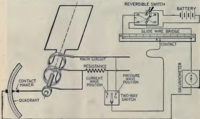
FIG. 2,595. —Diagram illustrating zero method of wave measurement with contact maker . The voltage of the battery must be at least as great as the maximum pressure to be measured and must be kept constant.
