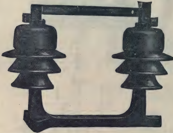
FIG. 2,208. —Westinghouse single pole disconnecting switch. Disconnecting switches are used primarily for isolating apparatus from the circuit for purposes of inspection and repair; also for sectionalizing feeders. They are not designed for opening under load, and therefore no attempt should be made to open them with current in the circuit. In connection with lightning arrester installations, disconnecting switches are particularly useful, providing a simple and effective means for isolating the arresters while cleaning and inspecting. The switch is opened and closed with a hook on the end of a wooden pole, which hook engages in a hole provided in the switch blade. This type of disconnecting switch is intended for wall mounting. The live parts are mounted on porcelain insulators carried on a cast iron yoke or base, forming a simple and substantial construction.
