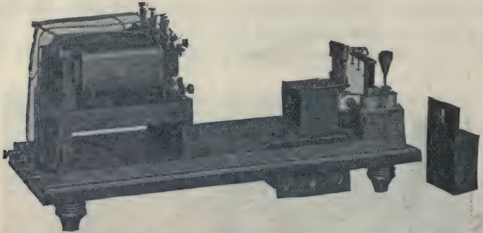
FIG. 2,601.—General Electric moving coil oscillograph with case removed, showing interior construction and arrangement of parts. The oscillograph is furnished complete with a three element electromagnet galvanometer, optical system, shutter and shutter operating mechanism, film driving motor and cone pulleys, photographic and tracing attachments, 6 film holders, and the following repair parts, for vibrators: 6 extra suspension strips; 6 vibrator mirrors; 1 box gold leaf fuses; 1 bottle mirror cement; 1 bottle damping liquid.
