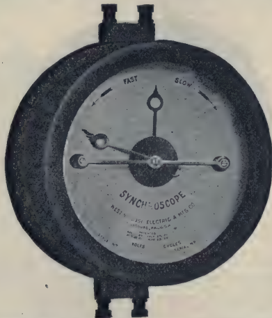
FIG. 2,570. —Westinghouse rotary type of synchroscope or synchronism indicator. The indication is by means of a pointer which assumes at every instant a position corresponding to the phase angle between the pressures of the busbars and the incoming machine, and therefore rotates when the incoming machine is not in synchronism. The direction of rotation indicates whether the machine be fast or slow, and the speed of rotation depends on the difference in frequency. The pointer is continuously visible, during both the dark and light periods of the synchronizing lamps.
