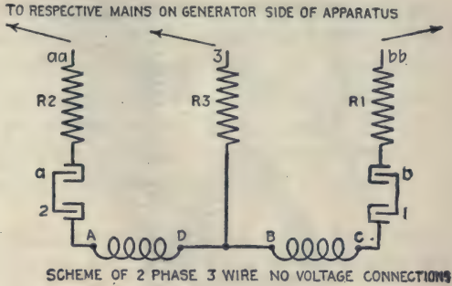
FIGS. 2,334 and 2,335.—Diagram showing two phase three wire no voltage connections for I-T-E circuit breaker. The two no voltage coils for two phase, three wire circuits are connected respectively to binding posts B, C and A D on the face of the base, and from A and C connections are made to lower contacts 2 and 1 respectively of the disconnecting switch. Binding posts B and D are connected together on the back of the board. (In instruments supplied on individual bases, these connections are made in the factory, let into channels in back of base and covered with wax.) Each of the upper contacts a and b is connected respectively through resistance R2 and R1 to one of the mains at aa and bb as shown. D is connected through resistance R3 to the common wire of both phases at 3 B and D being connected as aforesaid, thus forming a common connection for both no voltage coils. Terminals aa and bb of the resistances must be connected to the outside main across the two phases, terminal 3 to the main common to both phases, the connections being so made that these terminals will be subject to the full voltage of the circuit irrespective of the position of the starting switch.
