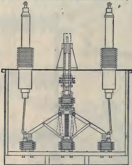
FIG. 2,220. —Kelman switching mechanism. The pantograph arrangement of the contact blades gives a double horizontal break deep down in the oil. This gives over the break a heavy head of oil which immediately closes in around the thin blades as they leave the contacts in opening, thus effectually extinguishing the arc. The opening spring acts within the pantograph itself without any intervening mechanism, and the light weight of the few moving parts enables the spring to accelerate the blades rapidly, thus obtaining a quick break. The contacts are of the return bend type, which makes a flexible contact, to obtain alignment with the blades at all times. The pantograph and contacts are supported on corrugated porcelain insulators on a hardwood base or insulator board. The insulators are fitted with iron ends for securing the different parts. At each end of the insulator board is an upright or lifting board which serves to lift the switching mechanism out of the tank. The leads are heavily insulated.
