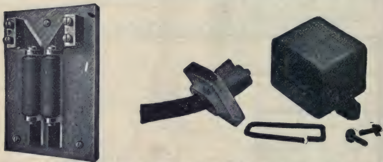
FIGS. 2,359 to 2,364. —Westinghouse safety spark gaps. Fig. 2,359, indoor type; figs. 2,360 to 2,364, outdoor type. It is well known that with transformers, operating on high voltage lines and having large ratios of transformation, there may occur, on the low tension side, momentary voltages to ground greatly in excess of the normal. These momentary increases in voltage between the low tension circuits and ground are commonly called “static disturbances.” In general they are the result of a change in the static balance of the high tension side and its connecting circuits. Unless certain precautions are taken, such a static disturbance on the low tension side may cause serious stresses in the secondary insulation of a transformer with a high ratio of transformation. This induced static voltage is independent of the ratio of transformation. The static stresses are more serious in a high ratio transformer simply because the insulation of its secondary is less able to withstand them. A method of relieving this disturbance is to connect a discharge spark gap between some point of the low tension side of the transformer to be protected (a middle or neutral point, if one be available) and the ground. The spark gap opening is such that any voltage very much in excess of the maximum normal will cause a discharge to ground, and thus the low tension side is practically tied to ground during such disturbance, while at other times it is ungrounded. The Underwriters recommend the grounding of the neutral point of low tension circuits when the conditions are such that the maximum normal voltage between the point connected and ground will not exceed 250 volts. The rule allows one side of a 250 volt circuit or the middle point of a 550 volt circuit to be grounded. The spark gaps shown above are designed for use on transformer secondary circuits and for protecting individual series arc lamps. These spark gaps are single pole, and consist of two cylinders of non-arcing metal with an air gap between. One of the cylinders is connected to the ground, the other to the line.
