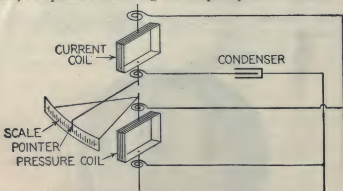
FIG. 2,568.—Langsdorf and Gegole frequency meter. The operation of this meter is based on the fact that if an alternating pressure of E Volts be impressed on a condenser of capacity C , in farads, the current in amperes will be equal to 2\pi \sim EC , provided the pressure be constant. In construction, the scale is mounted on the same axis as the pressure coil, across the mains so as to render the instrument independent of variation of voltage. For a discussion of this meter, see Electrical Review , vol. LVIII, page 114.
