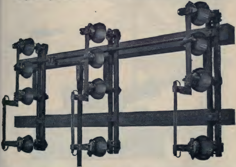
FIG. 2,216. —Pacific 22,000 volt, 100 ampere, pole top switch equipped with fuse tubes; designed to meet the need for a small group controlled disconnecting switch, having several features making it suitable for use with service transformer installations and line branches. The switch is made with clamped pipe arms permitting adjustment. It is equipped with fuse tubes and fittings, but should the fuses be not desired, the arm may be shortened. Provision is made for fitting insulator pins to the top of the arms, when the switch is mounted vertically, which will hold insulators at right angles to the switch, making it possible to end a line on the top of these arms and then drop down through the switch to the bank of transformers. The switch is so constructed that gravity tends to hold it in either the open or the closed position. Provision can be made for locking.
