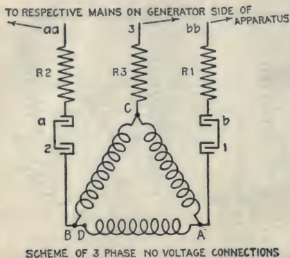
FIG. 2,336 and 2,337.—Diagram showing three phase no voltage connections for I-T-E circuit breaker. The no voltage coils for three phase circuits are connected in \Delta by means of binding posts A, B, C and D on the face of the base, and from the A and B of the no voltage coils, connections are made respectively to spring contacts 1 and 2 of the small disconnecting switch. Each of the contacts a and b of the disconnecting switch is connected through resistance R2 and R1 to one of the mains at aa and bb . The terminal C is connected through resistance R3 to the middle main as shown at point 3. The terminal D is linked on the back of the board to terminal B to complete the \Delta connection. The terminals aa , bb and 3 of the circuit breaker must, in all cases, be so connected that they will be subject to full voltage of the circuit irrespective of the position of the starting switch. Each no voltage coil is supplied with two terminal wires, one covered with green and one with black insulation. In replacing these coils particular care should be taken to see that the terminal wires connected to any one binding post are of unlike color.
