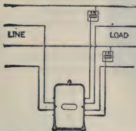
Figs. 2,538 to 2,541. —Connections of Fort Wayne multi-phase watt hour meters (type k_3 —forms MAB and MAK), for 100–625 volt circuits, 5–150 amperes. Fig. 2,538 two and three phase, three wire circuit, 25–36 cycles; fig. 2,539 two and three phase, 3 wire circuit, 36 cycles and above; fig. 2,540, two phase 4 wire circuit, 25–36 cycles; fig. 2,541 two phase, 4 wire circuit 36 cycles and above.
