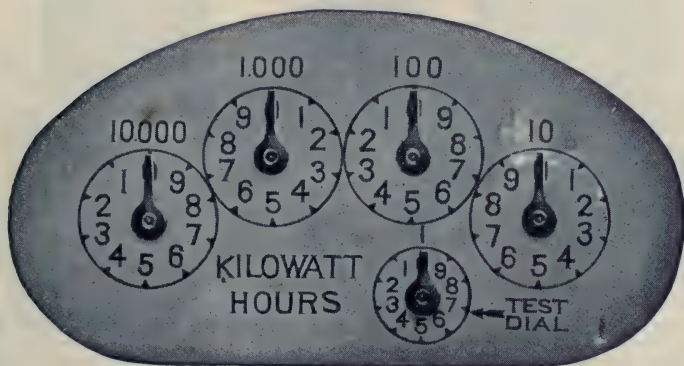
FIG. 2,550. —Canadian dial of Sangamo single phase induction watt hour meter. It has a small test circle indicating one kilowatt hour per revolution in all sizes where the first regular circle indicates 10. This is provided to conform with the requirements of the Canadian government and it is intended that the hand on the test circle shall make not less than \frac{1}{2} revolution in one hour with full load on a meter. In the case of a 10 ampere meter, it will make one complete revolution in one hour and for a 20 ampere, two revolutions, and so on. The train or indicating mechanism is carried on a rigidly formed and swaged brass bracket, accurately located by two dowel pins set in the top face of the main grid, and is held to the grid with two screws easily accessible when it is desired to remove the train for any purpose. All indicating trains used on type "H" meters are marked with symbols on the back of the train and on the compound attachment to indicate the gear ratio of each combination; this ratio being different for meters of different capacities in order to obtain a direct reading in kilowatt hours on the dial.
