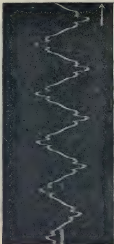
FIG. 2,635.—Short circuit current on direct current end of rotary converter, 21,500 amperes maximum. Upper curve, direct current voltage; lower curve, direct current amperage. Duration of short circuit about .1 second.
