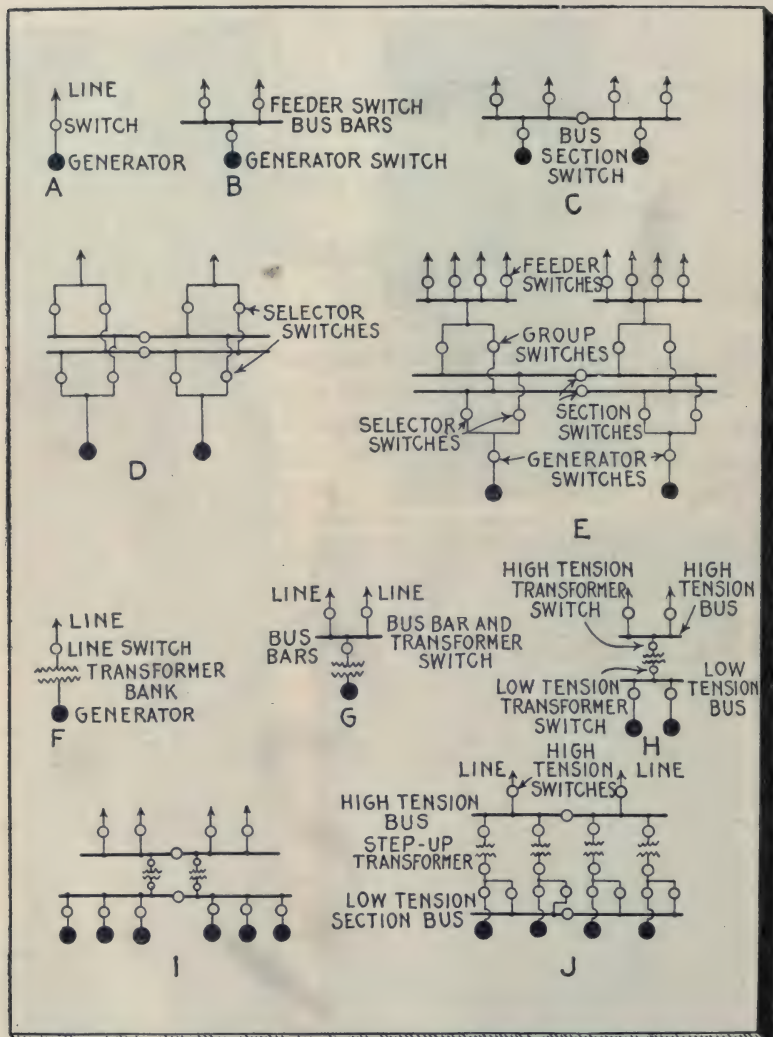
FIGS. 2,645 and 2,646.—Diagrams illustrating general principles of switchboard connections.
