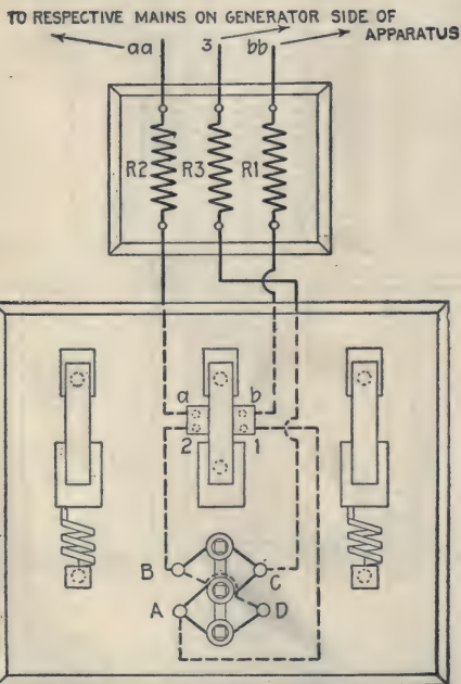
FIG. 2,336 and 2,337.—Diagram showing three phase no voltage connections for I-T-E circuit breaker. The no voltage coils for three phase circuits are connected in \Delta by means of binding posts A, B, C and D on the face of the base, and from the A and B of the no voltage coils, connections are made respectively to spring contacts 1 and 2 of the small disconnecting switch. Each of the contacts a and b of the disconnecting switch is connected through resistance R2 and R1 to one of the mains at aa and bb . The terminal C is connected through resistance R3 to the middle main as shown at point 3. The terminal D is linked on the back of the board to terminal B to complete the \Delta connection. The terminals aa , bb and 3 of the circuit breaker must, in all cases, be so connected that they will be subject to full voltage of the circuit irrespective of the position of the starting switch. Each no voltage coil is supplied with two terminal wires, one covered with green and one with black insulation. In replacing these coils particular care should be taken to see that the terminal wires connected to any one binding post are of unlike color.
