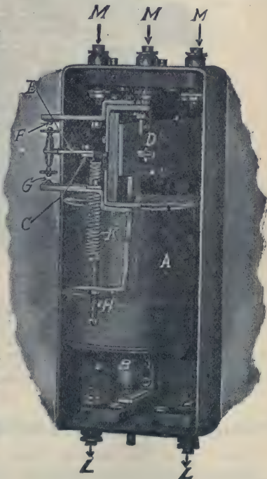
FIG. 2,426. —Westinghouse voltage regulating primary relay; view of mechanism with case removed. This relay is practically a voltmeter arranged for making and breaking contacts with fluctuations of voltage. As shown in the figure, it consists essentially of a solenoid and a balance beam carrying two movable contact points on one end and attached to the solenoid core at the other. The oscillation of the core causes the contact carrying end of the beam to move between two stationary contact points connected to the auxiliary or secondary relay circuit. The stationary contact points are fitted with adjusting screws for either increasing or decreasing the distance between them, to the amount of change in the voltage required for making or breaking contact; in other words, for varying the sensitiveness of the relay. Means for varying the normal voltage which it is desired to maintain are provided in the spring attached to the balance beam and controlled by the micrometer adjusting screw. Increasing the tension of the spring results in lowering the normal voltage position. The relay is wound for a normal voltage of 110 volts, and has a range of adjustment from 90 to 130 volts. The total energy required for its operation is about 50 watts at normal voltage. Voltage transformers having at least 50 watts capacity are, therefore, required. The parts are: A, solenoid; B, solenoid core; C, end of balance beam; D, pivots, bearings; E, movable contact arm; F, upper stationary contact point; G, lower stationary contact point; H, adjusting screw; K, adjusting spring; L, feeder binding posts; M, auxiliary circuit and secondary relay binding posts.
