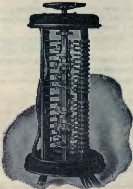
FIG. 2,431. —Westinghouse drum type variable transformer voltage regulator. It consists of a drum and finger type switch. A preventive resistance is used between the different contacts, making it unnecessary to open the circuit when moving from one tap of the regulating transformer to the next tap. A spring actuated, quick moving, central stopping mechanism is used to prevent burning the resistances. The regulator is arranged to give 40 points of regulation. In many cases this large number of points is not absolutely necessary, but it is desirable to use them because the voltage per step is thus reduced to a small value, and a corresponding increase in the life of the contacts results because of the reduced sparking at the lower voltage. Two drums are employed. The first drum has ten contacts and a corresponding number of fingers, the latter being mounted upon an insulated bar. These fingers are connected to the floating coils of the regulating transformer, and as the drum is rotated, the finger connected to the line is brought into contact successively with each of the ten taps. The second drum is of similar construction and consists of a changing and reversing switch. It connects the two floating coils to the various taps on the main secondary coil of the regulating transformer at the proper time, and also reverses the transformer so that the total winding can be used for either raising or lowering the voltage. All the points of regulation are obtained by a continuous motion of the handle, the various connections produced in the manner are shown in the diagram, fig. 2,433. The top and base of the regulator are made of cast iron and the top is supported by steel bars, two of which are insulated, and used to support the metallic bases finger to which the cable leads are attached. The drums consist of metal castings mounted upon insulated shafts. The first drum, which is the only one upon which arcing can take place, is provided with removable copper contact tips. The main castings are made of aluminum to secure low inertia of the drum. A sheet iron cover is used to enclose the regulator, and the leads are brought out through the bottom of the controller.
