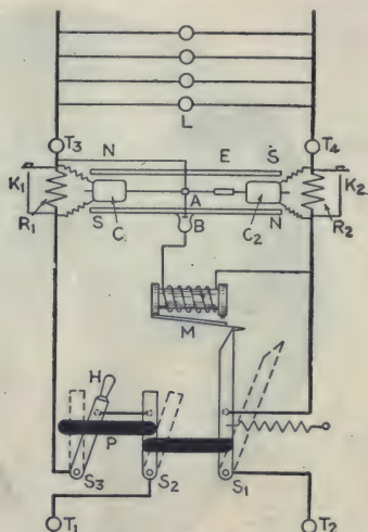
FIG. 2,582.—Wallis-Jones automatic earth leakage cut out. It is an instrument which so protects a direct current circuit that the circuit is broken whenever a leak occurs from either main to earth, and so that the circuit cannot be permanently re-established until the leak has been removed. The instrument and its connections may be explained by the aid of the accompanying diagram, in which T_1 and T_2 represent the points of connection from the mains, and T_3 and T_4 , the points of connection to the circuit to be protected. S_1 , S_2 , and S_3 will preferably be ordinary tumbler switches, but they are diagrammatically represented as plain bar switches, their fixed contacts being diagrammatically represented by dotted circles. When the three switches S_1 , S_2 , and S_3 are closed, the current passes from T_1 to T_3 through the small resistance R_1 , through circuit L to T_4 , and back through the resistance R_2 to T_2 . In shunt with R_1 and R_2 , are the two moving coils C and C_2 , working in the magnetic field of the magnets NS , NS , and rigidly fixed on one spindle, which is broken electrically by an ebonite block E . The points of connection to the shunts are adjusted so that when the same current passes out through one and back through the other, the effect on the two coils is equal and opposite, and there is thus no movement. Should, however, any minute portion of the current through R_1 leak to earth instead of returning via R_2 , the balance is disturbed, C becomes stronger than C_2 , the system is deflected, and a contact is made by the arm A at B , no matter in which direction the coils deflect. The system is similarly deflected for a leak on the other lead. In the diagram these contacts are shown at right angles to their normal plane. As soon as the contact is made, the electro-magnet M is energized, the arm of S_1 is released and the spring at once pulls it off its contact, at the same time breaking S_2 . The positions of the blades of the switches are open are shown dotted. The only means the user has of closing the circuit is by putting on S_3 by the handle H , which is outside the locked box. The first effect of putting on S_3 is to break its circuit; it then by means of the slotted bar P begins to pull on S_2 and S_1 , which can thus be closed again, and held closed by the trigger as before. The circuit, is, however, still broken till S_3 is pushed back. Then if the leak is still on, the slot in P allows S_1 and S_2 to open at once as before. It is therefore impossible to keep the circuit closed while the leak exists. The working condition of the instrument can be tested at any time by switching a lamp on in the circuit and depressing one of the keys K_1 , K_2 . This short circuits R_1 or R_2 , throws the coils out of balance, and the switch opens. The contact arm is closed in an inner dust tight case, and it will be noted that it makes contact only; the break occurs at the switches, thus avoiding any sparking. Since the two coils work in the two gaps of one and the same field, changes in the strength of the magnets have no effect, the apparatus is enclosed in a locked metallic box, and the only part to which the user has access is the handle H , and, if desired, the testing keys K_1 , K_2 .
