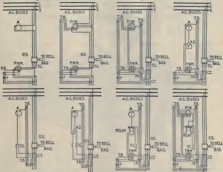
Figs. 2,659 to 2,666. —Diagram of connections for three phase feeder panels. Key to symbols: A, ammeter; A.S., three way ammeter switch; B.A.S., bell alarm switch; C.T., current transformer; F, fuse; O.S., oil switch; P.I.W., polyphase indicating wattmeter; P.W.M., polyphase watt-hour meter; T.B., terminal board; T.C., trip coils for oil switch.
