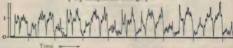
FIG. 2,587.—Oscillogram by Bailey and Cleghorne (Proc. I. E. E., Vol. XXXVIII), showing the sparking pressure or pressure between the brush and the commutator segment at the moment of separation. The waves fall into groups of three owing to the fact that there were three armature coils in each slot.
