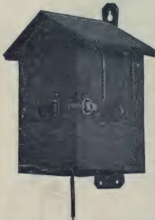
FIG. 2,371. —Westinghouse three pole or four pole arrester in weather proof wooden case which protects the arrester units from rain and snow when they are installed in exposed locations, as on poles or buildings.
