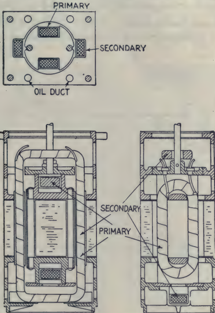
Figs. 2,444 to 2,446. —Sectional views of General Electric pole type regulator winding and core. The secondary core has only two slots containing a single coil, while the rotor or primary core has four slots. Two of these slots are occupied by a single primary coil, and the two circular slots in quadrature thereto contain the compensating or short circuit winding. This winding also serves to hold the primary punchings together, and it consists of two copper rods riveted to the two cast brass flanges. The secondary coil is form wound, while the primary coil is wound directly on the core. The rotor flanges, both top and bottom, are provided with discs which are turned in alignment with the punchings, and these discs bear against the top and bottom flanges between which the secondary punchings are clamped. These secondary flanges are also turned in alignment with the secondary punchings, so that an even air gap between the primary and the secondary is assured. The secondary coil is wound with an opening in the upper horizontal part which affords passage for the operating shaft of the rotor. A bearing for this shaft is provided in the table which supports the mechanism and from which the regulator is suspended. Flexible leads are brought out from the rotor and twisted around the shaft as in standard regulator practice. The regulator being two pole, the rotor is turned through an angle of 180 deg. to obtain the full range of the regulator.
