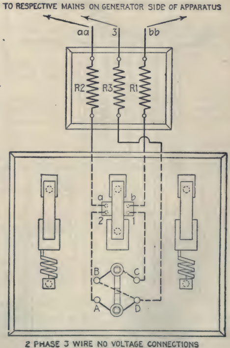
FIGS. 2,334 and 2,335.—Diagram showing two phase three wire no voltage connections for I-T-E circuit breaker. The two no voltage coils for two phase, three wire circuits are connected respectively to binding posts B, C and A D on the face of the base, and from A and C connections are made to lower contacts 2 and 1 respectively of the disconnecting switch. Binding posts B and D are connected together on the back of the board. (In instruments supplied on individual bases, these connections are made in the factory, let into channels in back of base and covered with wax.) Each of the upper contacts a and b is connected respectively through resistance R2 and R1 to one of the mains at aa and bb as shown. D is connected through resistance R3 to the common wire of both phases at 3 B and D being connected as aforesaid, thus forming a common connection for both no voltage coils. Terminals aa and bb of the resistances must be connected to the outside main across the two phases, terminal 3 to the main common to both phases, the connections being so made that these terminals will be subject to the full voltage of the circuit irrespective of the position of the starting switch.
