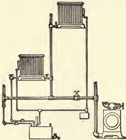
FIG. 207.—Paul System.
