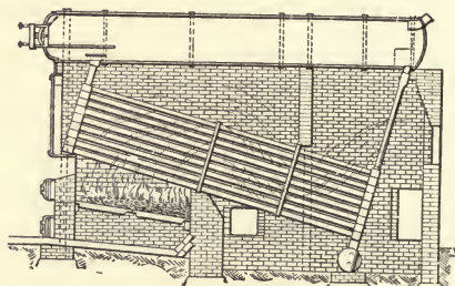
FIG. 138.—Babcock & Wilcox Boiler.
