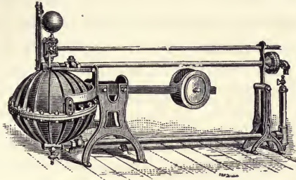
FIG. 184.—Gravitating Return-trap.
