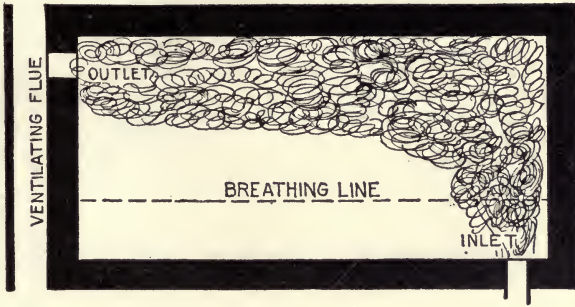
FIG. 23.—Air Introduced at Bottom, Discharged at Top.
