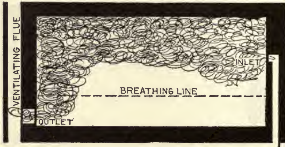
FIG. 26.—Air Admitted on Side, Discharged near Bottom.
