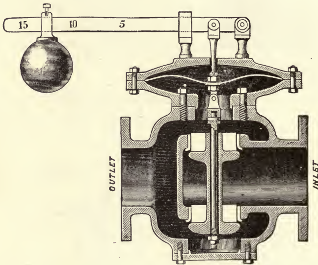
FIG. 212.—Holt's Reducing-valve.
