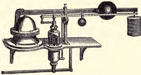
FIG. 172.—Piston Damper-regulator.
