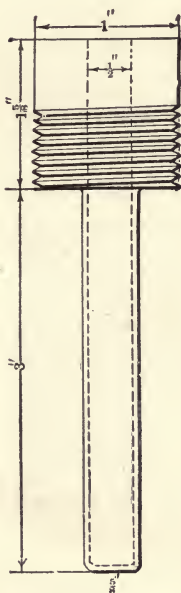
FIG. 9.—Thermometer-cup.
