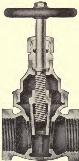
FIG. 84.—Gate Valve.
