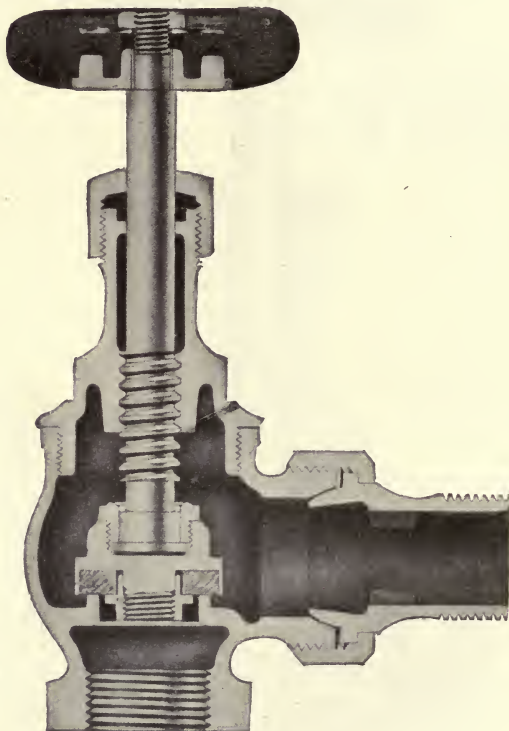
FIG. 86.—Angle Valve.
