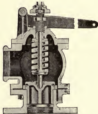
FIG. 163.—Section of Spring or Pop Safety-valve.
