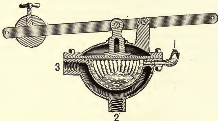
FIG. 278.—Lawler Hot-water Damper-regulator.
