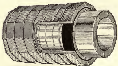
FIG. 39.—Wyckoff Built-up Wood Tubing.
