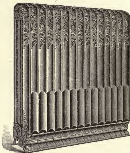
FIG. 127.—Direct-indirect Radiator.
