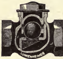
FIG. 96.—Horizontal Check with Ball Clack.
