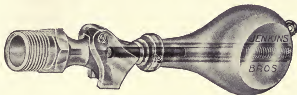
FIG. 165.—Try-cock.
