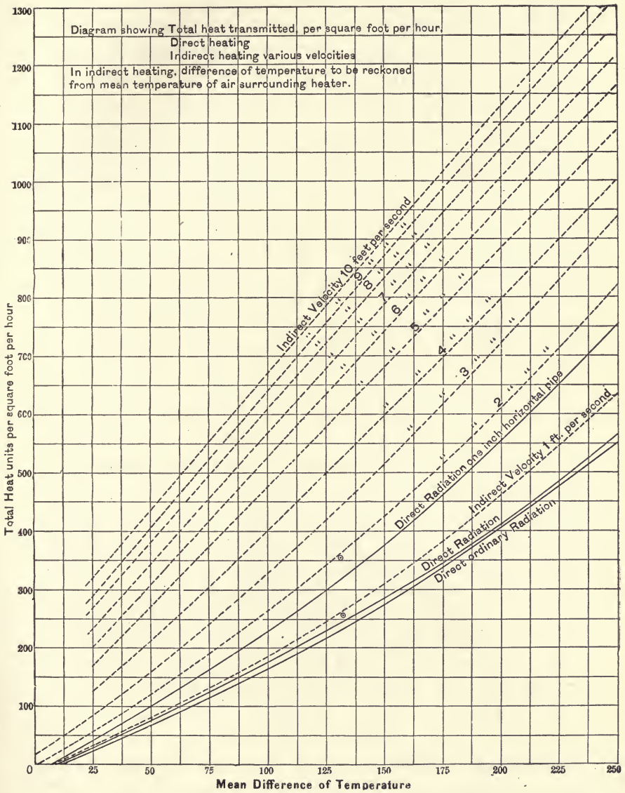
Fig. 106.—Diagram of Heat from Radiating Surfaces.
