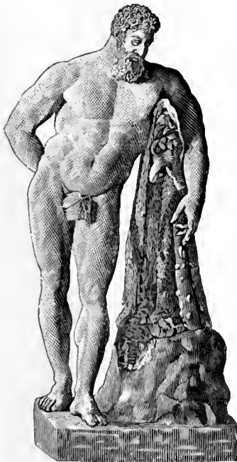
HERCULES—FARNESE.
