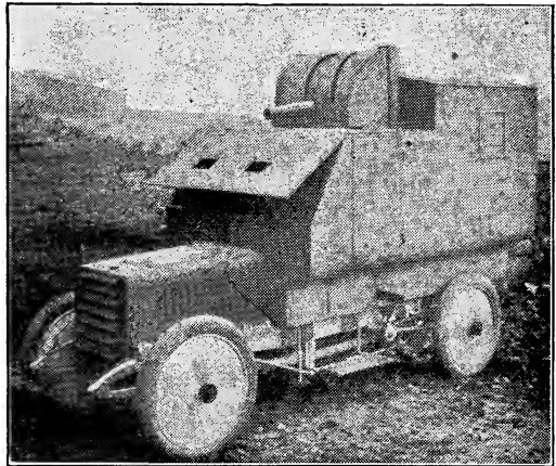
The automobile has been seized upon as a convenient and useful adjunct to the army. A number of different types of armed and armored automobiles have been brought into use by the various nations. This illustration shows one of the types so constructed that the cannon may be sufficiently elevated to shoot the war-balloons and air-ships.
