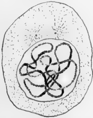
FIG. 2.—Spireme. Radiations from centrosomes.
