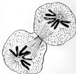
FIG. 9.—The cytoplasm dividing.
