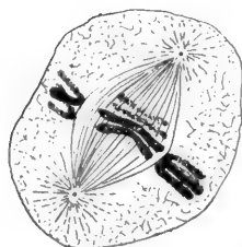
FIG. 7.—Splitting of the chromosomes.
