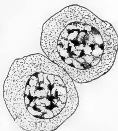
FIG. 11.—The two daughter cells complete.
