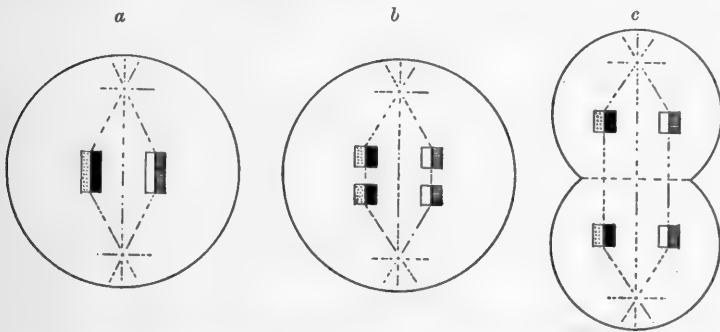
FIG. 17.—Showing the parallel joining of the chromosomes and their subsequent distribution to the daughter cells in the meiotic (reducing) division, according to the Louvain School.
