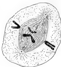
FIG. 5.—Chromosomes attached to spindle fibres (lateral view).
