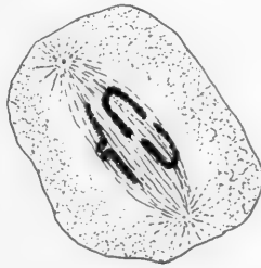
FIG. 13.—The pairs of chromosomes separating in the meiotic division.
