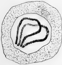
FIG. 12.—Early stage in the meiotic division.
