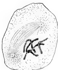
FIG. 4.—Disappearance of nuclear membrane.
