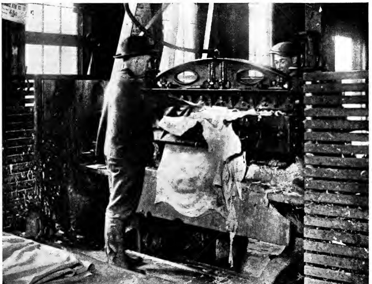
Delivery End showing two Splits
