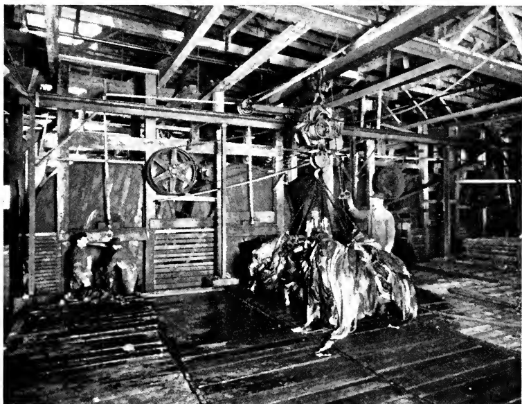
Soaking and Liming Pits with Crane Conveyor
