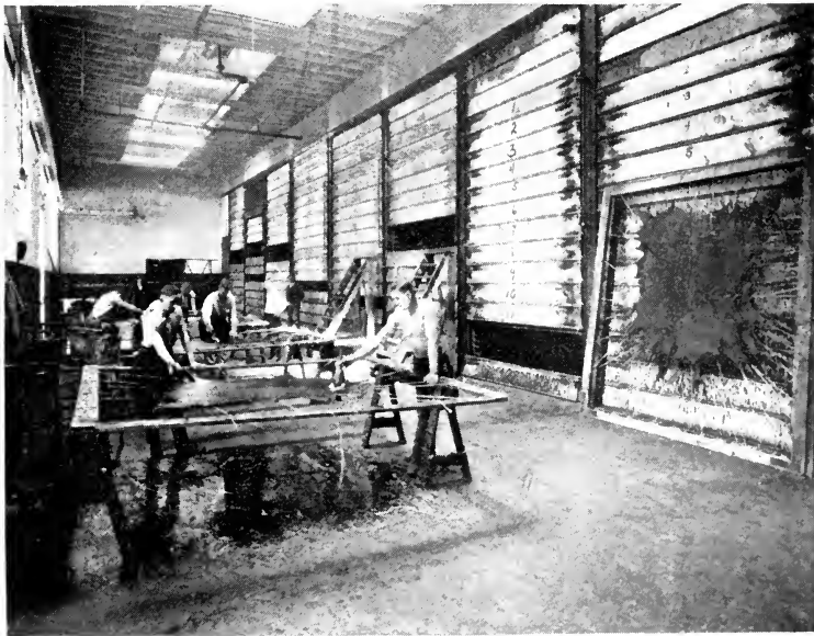
Varnishing Room, Showing Ovens
