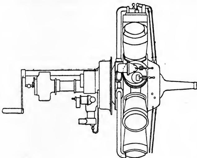
Clerget 115 h.p. Rotary Aero Engine, Side Elevation.
