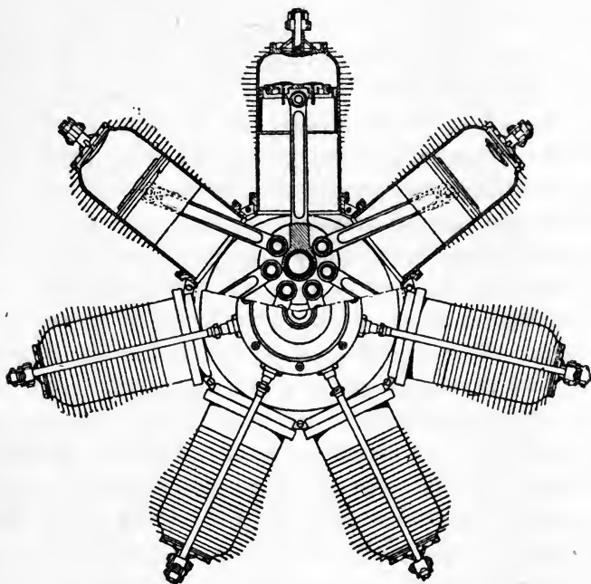
Bayerischer 7 Cylinder Rotary Engine, 1913.
