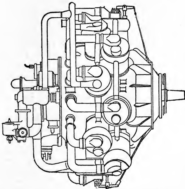
Salmson 200 h.p. Radial Engine, Side View.
