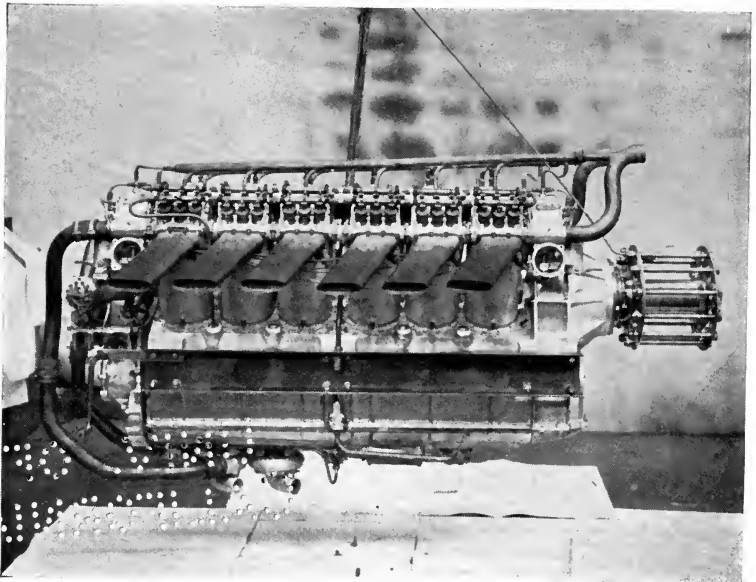
Sikh, 12-cylinder, side view.
