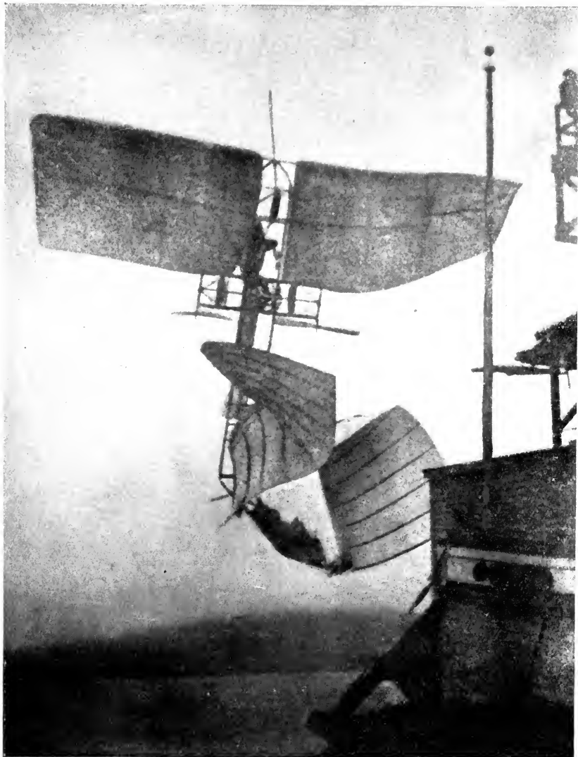
Trial of full-size Langley Aerodrome, 8th December, 1903.
