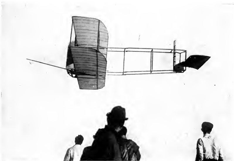
Orville Wright making the world's record in gliding flight, 10 minutes 1 second, stationary against a wind of 25 miles per hour, east of Kill Devil Hill.
