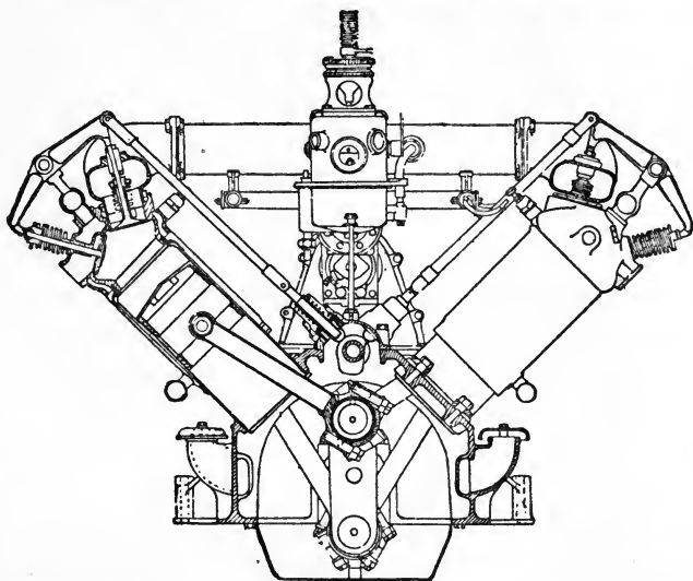
End View of Wolseley 120 horse-power Vee-type Engine.
