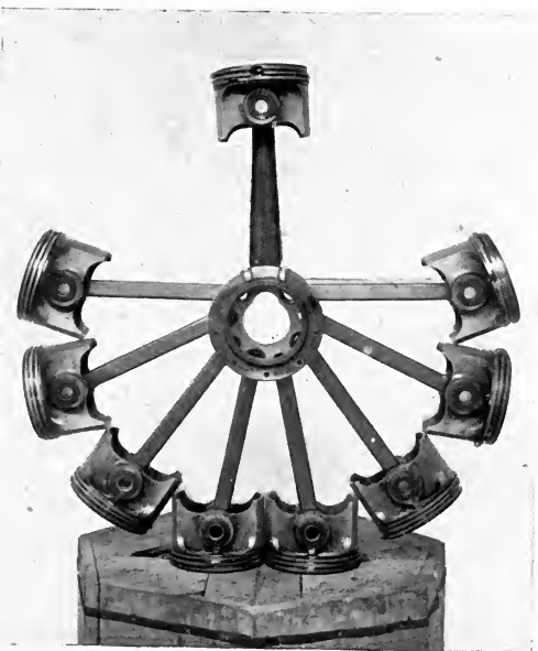
'Dragonfly' piston assembly.
