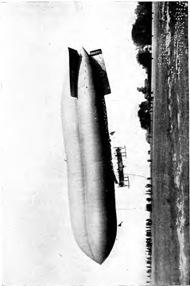
Coastal airship, showing gun on top of envelope.
