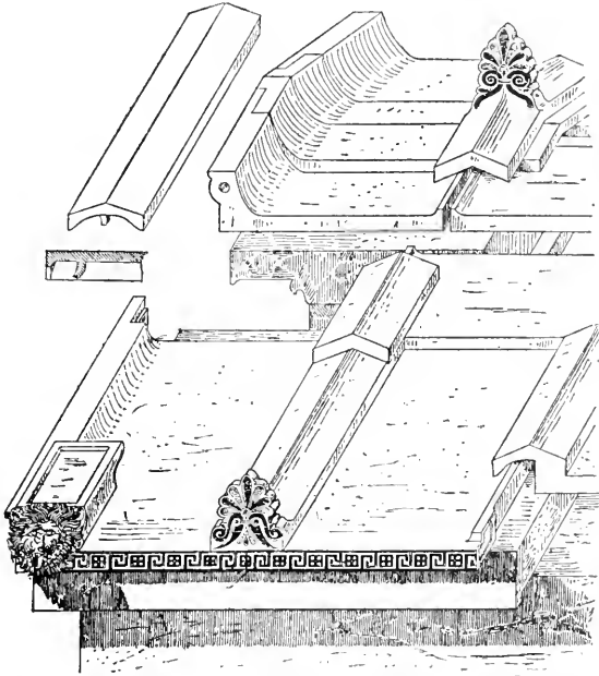
FIG. 9. DIAGRAM OF ROOF-TILING, HERAION, OLYMPIA.
