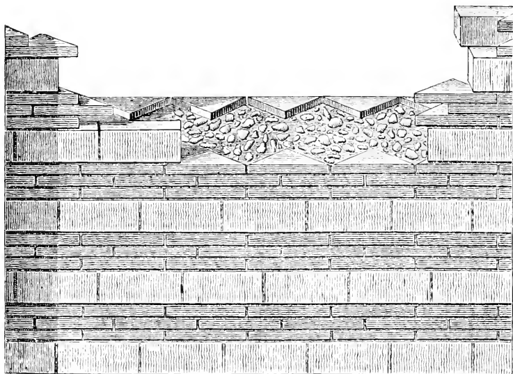
FIG. 100. DIAGRAM SHOWING CONSTRUCTION OF WALL OF OPUS MIXTUM.
