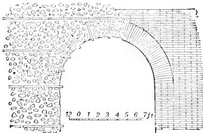
FIG. 189. CONCRETE ARCH; HALF WITH BRICK FACING REMOVED.
