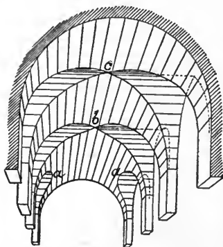
FIG. 109.—PENETRATIONS AND INTERSECTIONS OF VAULTS.
