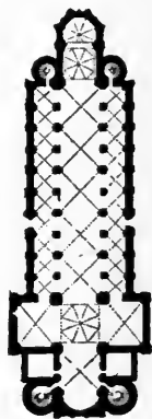
FIG. 99.—PLAN OF MINSTER AT WORMS.
