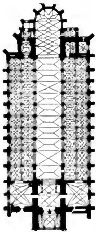
FIG. 143.—PLAN OF ULM CATHEDRAL.
