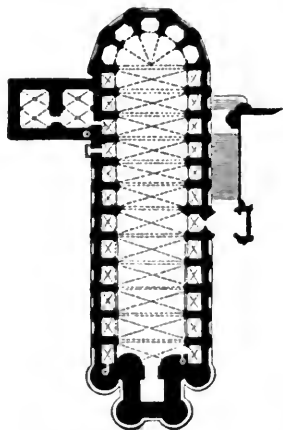
FIG. 123.—PLAN OF CATHEDRAL OF ALBY.
