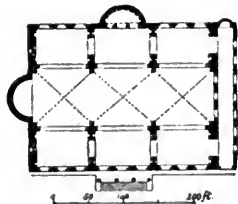
FIG. 58.—BASILICA OF CONSTANTINE. PLAN.
