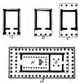
FIG. 31.—TYPES OF GREEK TEMPLE PLANS.
