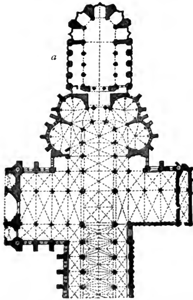
FIG. 137.—EASTERN HALF OF WESTMINSTER ABBEY.
