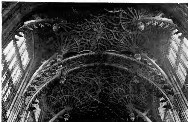
FIG. 136.—FAN-VAULTING, HENRY VII.'S CHAPEL, WESTMINSTER ABBEY.
