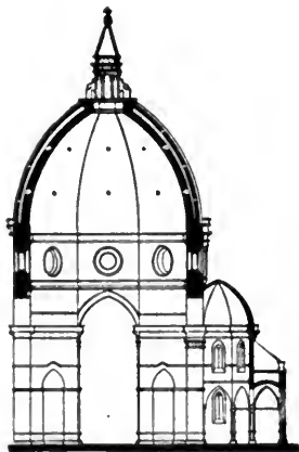
FIG. 159.—SECTION OF DOME OF DUOMO, FLORENCE.
