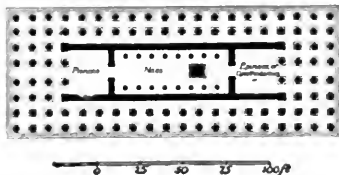
FIG. 39.—TEMPLE OF OLYMPIAN ZEUS, ATHENS.
