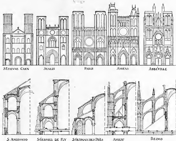
FIG. 147—ARRANGEMENT OF MONUMENTS AND DETAILS TO ILLUSTRATE THE DEVELOPMENT OF THE BUTTRESS AND THE DEVELOPMENT OF THE FACADE
