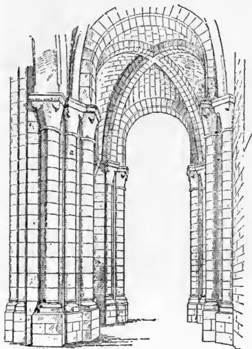
FIG. 133—BEAUVAIS. SAINT ETIENNE. DRAWING OF ONE OF THE AISLE VAULTS AND ITS SUPPORTS. (FROM MOORE)
