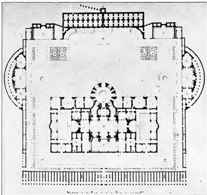
FIG. 48—ROME. THERMÆ OF CARACALLA. PLAN. (RESTORED BY BLOUET)
