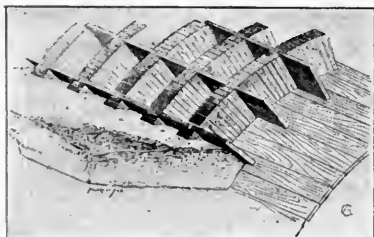
FIG. 60—ROMAN CELLULAR VAULT. (CHOISY)
