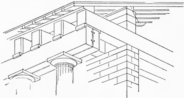
FIG. 20—THE GREEK DORIC ORDER, WITH A RETRANSLATION INTO WOOD. (AFTER DURM)
