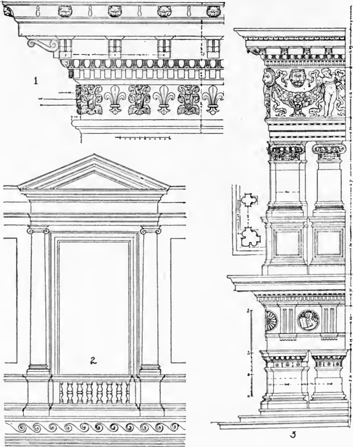
FIG. 211—"HIGH RENAISSANCE" DETAILS. (AFTER GROMORT)
