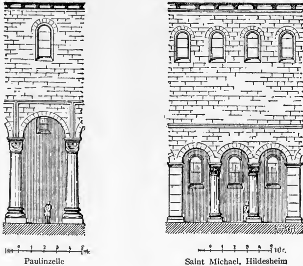
FIG. 113—SYSTEMS OF GERMAN ROMANESQUE CHURCHES
