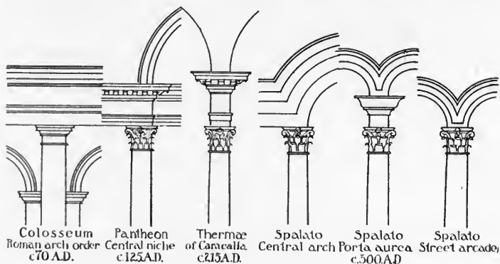
FIG. 59—DEVELOPMENT IN THE RELATIONS OF ARCH AND COLUMN IN ROMAN ARCHITECTURE
