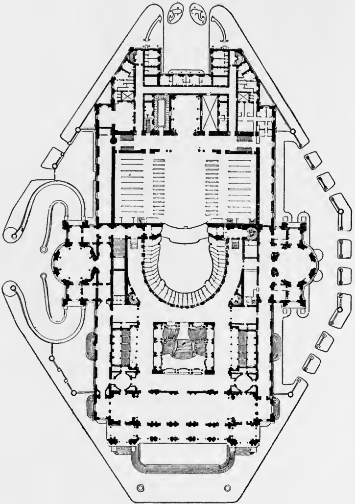
FIG. 275—PARIS. OPERA HOUSE. PLAN
