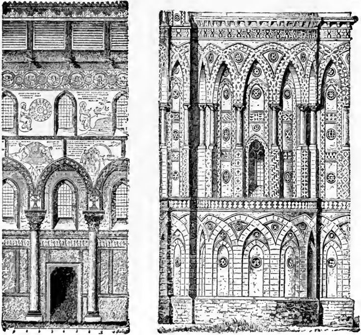
FIG. 110—MONREALE. CATHEDRAL. SYSTEM OF THE NAVE AND THE EXTERIOR OF THE CHOIR
