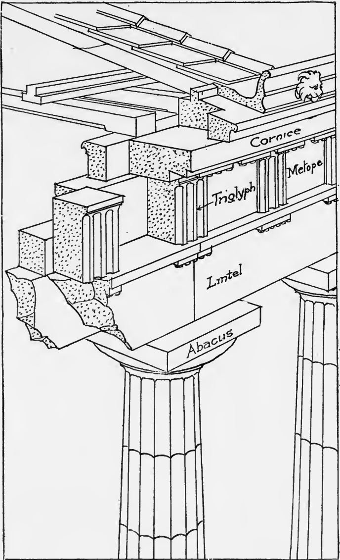
FIG. 19—THE GREEK DORIC ORDER
