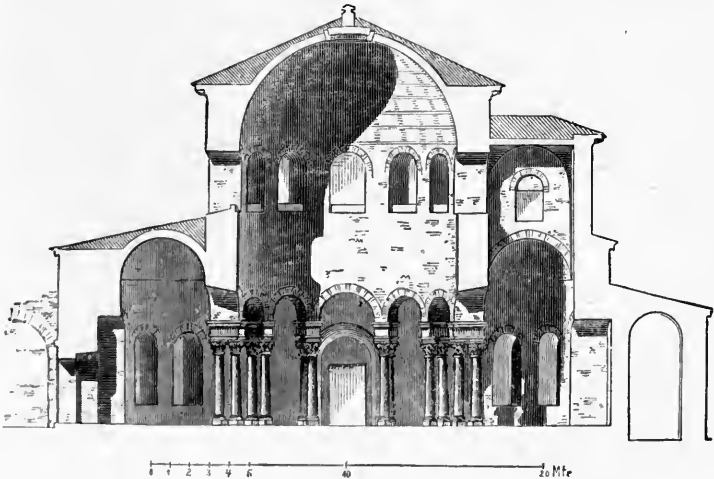
FIG. 71—ROME. SANTA COSTANZA. SECTION SHOWING THE CONSTRUCTION
