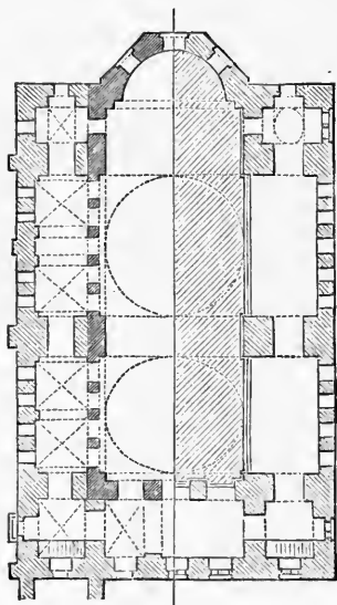
FIG. 78—CONSTANTINOPLE. SAINT IRENE. PLAN
