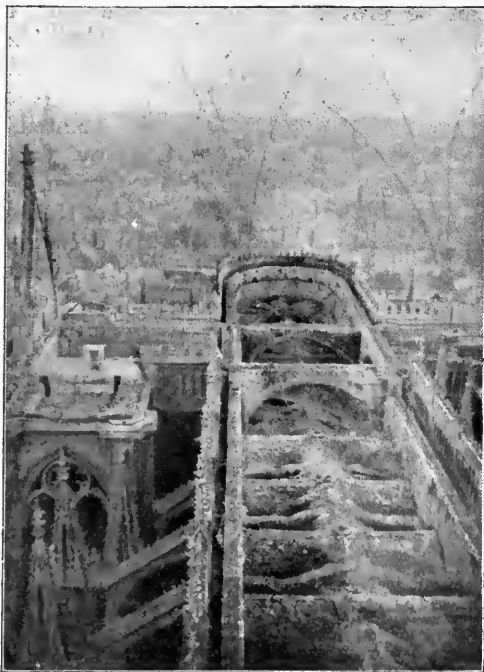
FIG. 144—REIMS. THE CATHEDRAL. VIEW OF THE VAULTS AFTER THE FIRST BOMBARDMENT IN 1914, SHOWING THE LEVEL CROWNS OF DEVELOPED GOTHIC VAULTS
