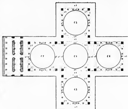
FIG. 84—CONSTANTINOPLE. THE HOLY APOSTLES. PLAN, RESTORED
