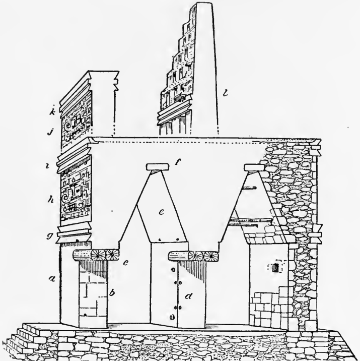
FIG. 283—TRANSVERSE SECTION OF A TYPICAL MAYA BUILDING. (HOLMES)
