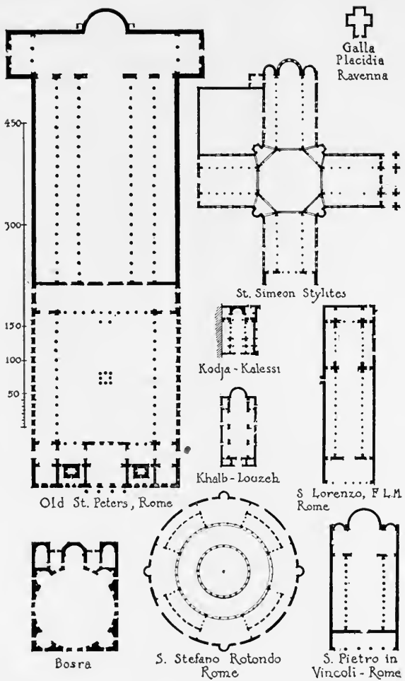
FIG. 63—PLANS OF EARLY CHRISTIAN CHURCHES
