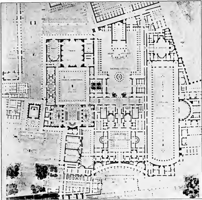
FIG. 56—ROME. PALACES OF THE CÆSARS. PLAN. (RESTORED BY DEGLANE)
