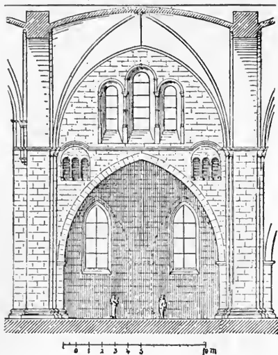
FIG. 166—MUNSTER. CATHEDRAL, SYSTEM
