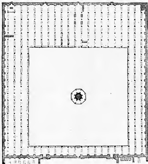
FIG. 310—CAIRO. MOSQUE OF AMRU. PLAN
