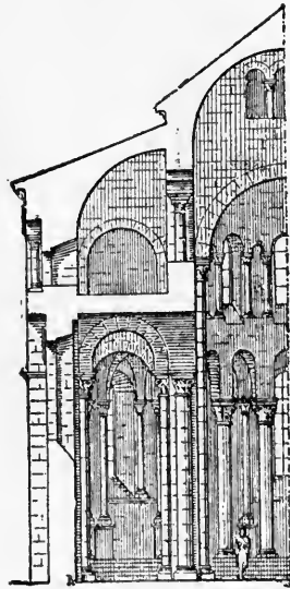
FIG. 120 — CLERMONT - FER-RAND. NOTRE DAME DU PORT. TRANSVERSE SECTION, SHOWING HALF-BARREL VAULT OVER THE AISLE
