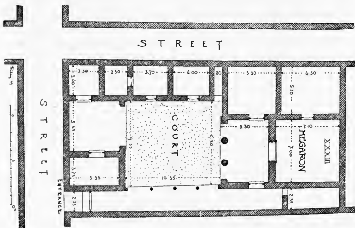
FIG. 33—PRIENE. "HOUSE XXXII". (WIEGAND)
