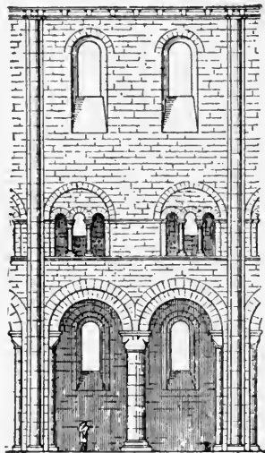
FIG. 127—JUMIEGES. ABBEY CHURCH. THE SYSTEM
