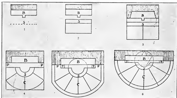
FIG. 46—SCHEMATIC REPRESENTATION OF THE DEVELOPMENT OF THE ROMAN THEATER. (FIECHTER)
