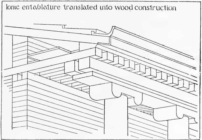
FIG. 22—IONIC ENTABLATURE, RETRANSLATED INTO WOOD. (AFTER DURM)
