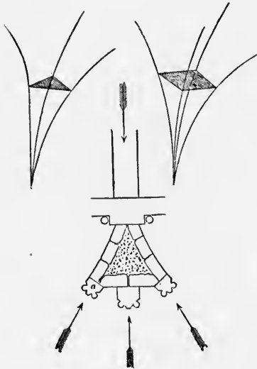
FIG. 145—SECTION OF GOTHIC VAULTING CONOID, SHOWING THE DIRECTIONS OF THE THRUSTS AND THEIR ABUTMENTS
