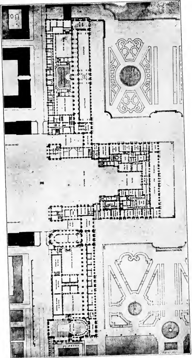
FIG. 237—VERSAILLES. PLAN OF THE PRINCIPAL FLOOR OF THE PALACE. (GROMORT)
