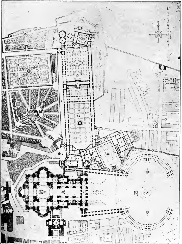
FIG. 222—ROME. PLAN OF SAINT PETER'S AND THE VATICAN. (GROMORT)
