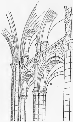
FIG. 101—MILAN. SANT' AMBROGIO. DRAWING OF ONE BAY SHOWING VAULT RIBS AND SUPPORTS. (MOORE)
