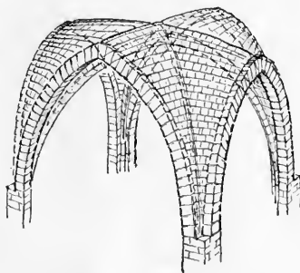
DEVELOPED GOTHIC VAULT
