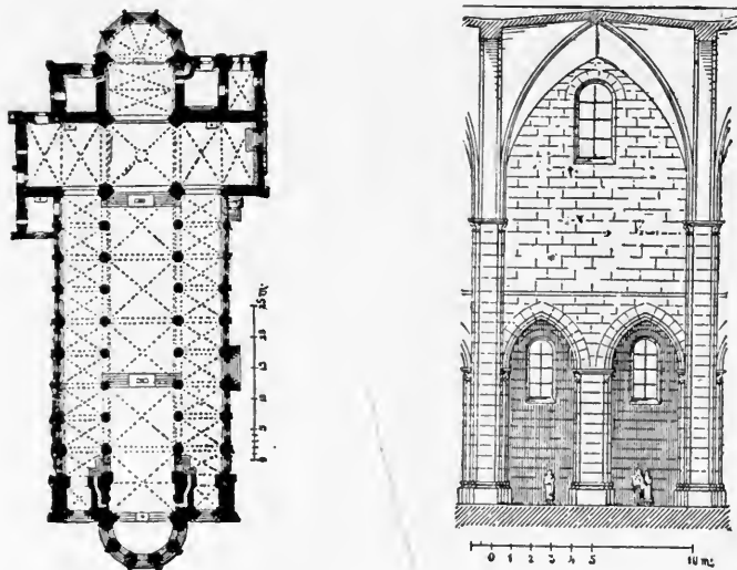
FIG. 165—BAMBERG. CATHEDRAL. PLAN AND SYSTEM
