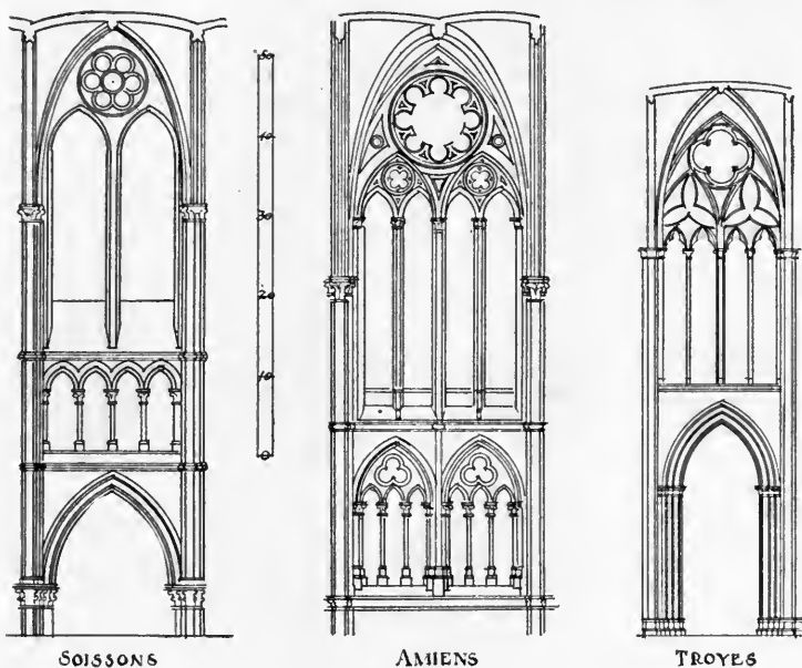
FIG. 151—THE DEVELOPMENT OF THE WINDOW OPENING. EXAMPLES OF PLATE AND BAR TRACERY
