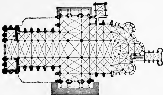
FIG. 155—CHARTRES. CATHEDRAL. PLAN
