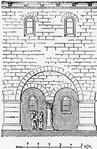
FIG. 114—DRUBECK. DRAWING OF ONE BAY, SHOWING THE SYSTEM
