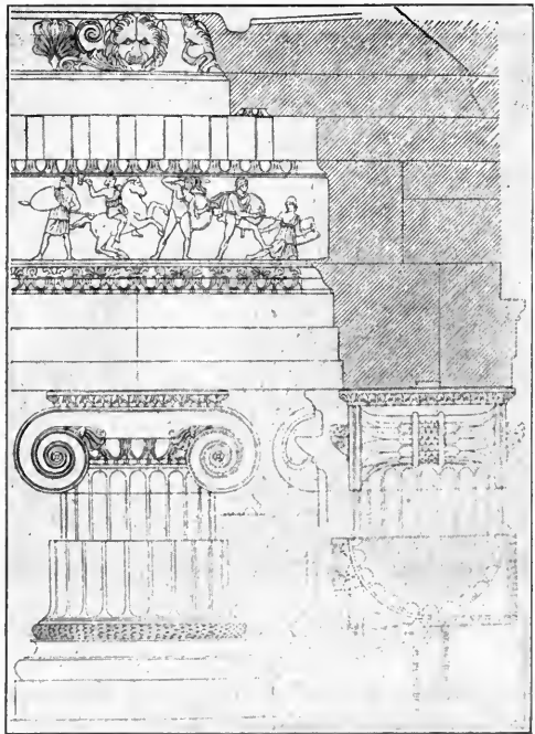
FIG. 23—MAGNESIA. TEMPLE OF ARTEMIS. DETAILS. (HUMANN)
