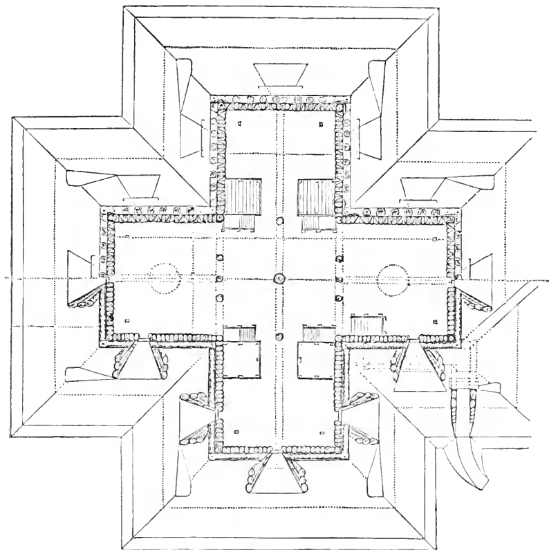
FIG. 7. PLAN OF ARTILLERY BLOCK-HOUSE.
