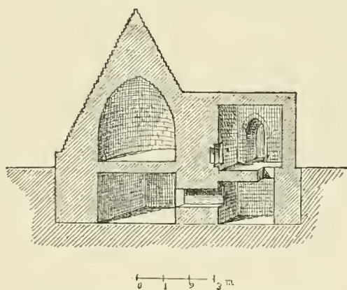
FIG. 163.—Section of the above tomb.
