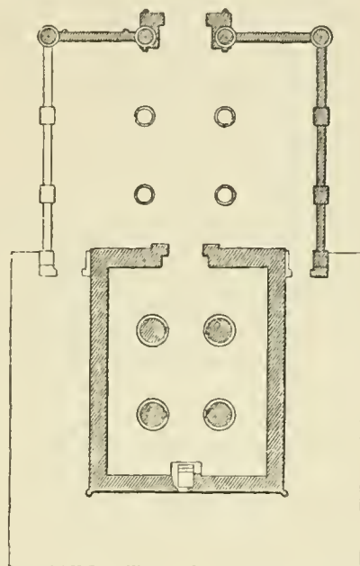
FIG. 232.—Temple of Amenophis III. at Eilithyia; from Lepsius.
