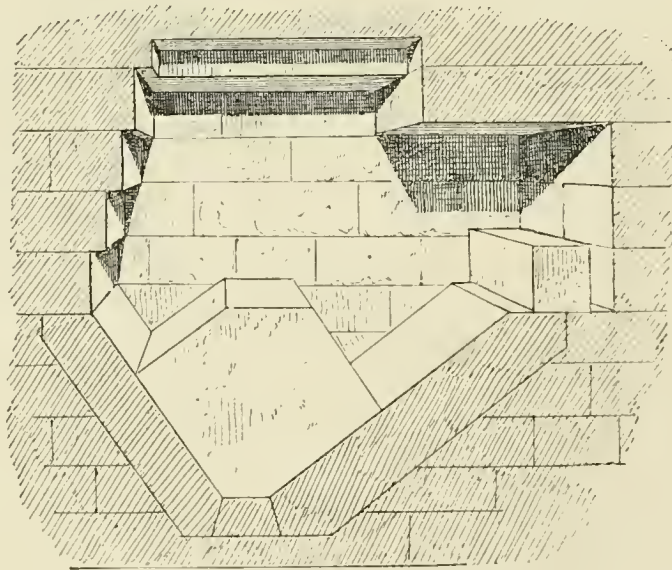
FIG. 151.—Portcullis closed.
