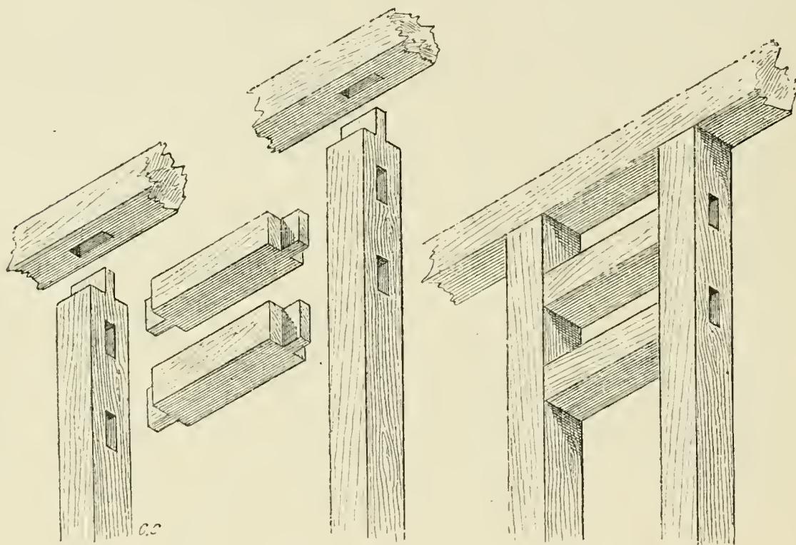
FIG. 82.—Elements of wooden construction.
