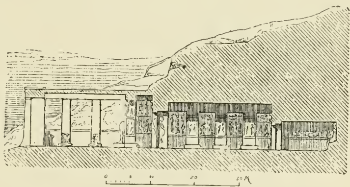
FIG. 241.—Longitudinal section, Derri ; from Hureau.
