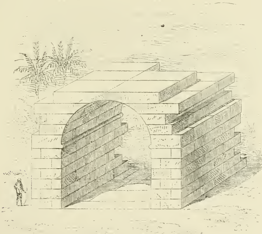
FIG. 76.—Off-set semicircular arch.
