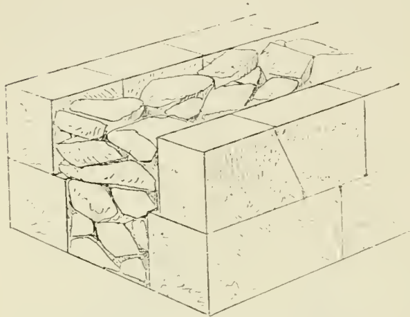
FIG. 70.—Double-faced wall.
