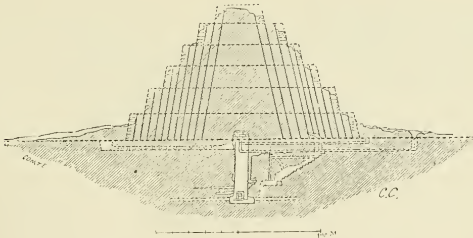
FIG. 134.—Section of the Stepped Pyramid ; from Perring.
