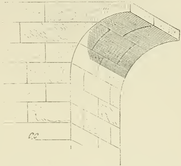
FIG. 75.—Arrangement of the courses in an off-set arch.
