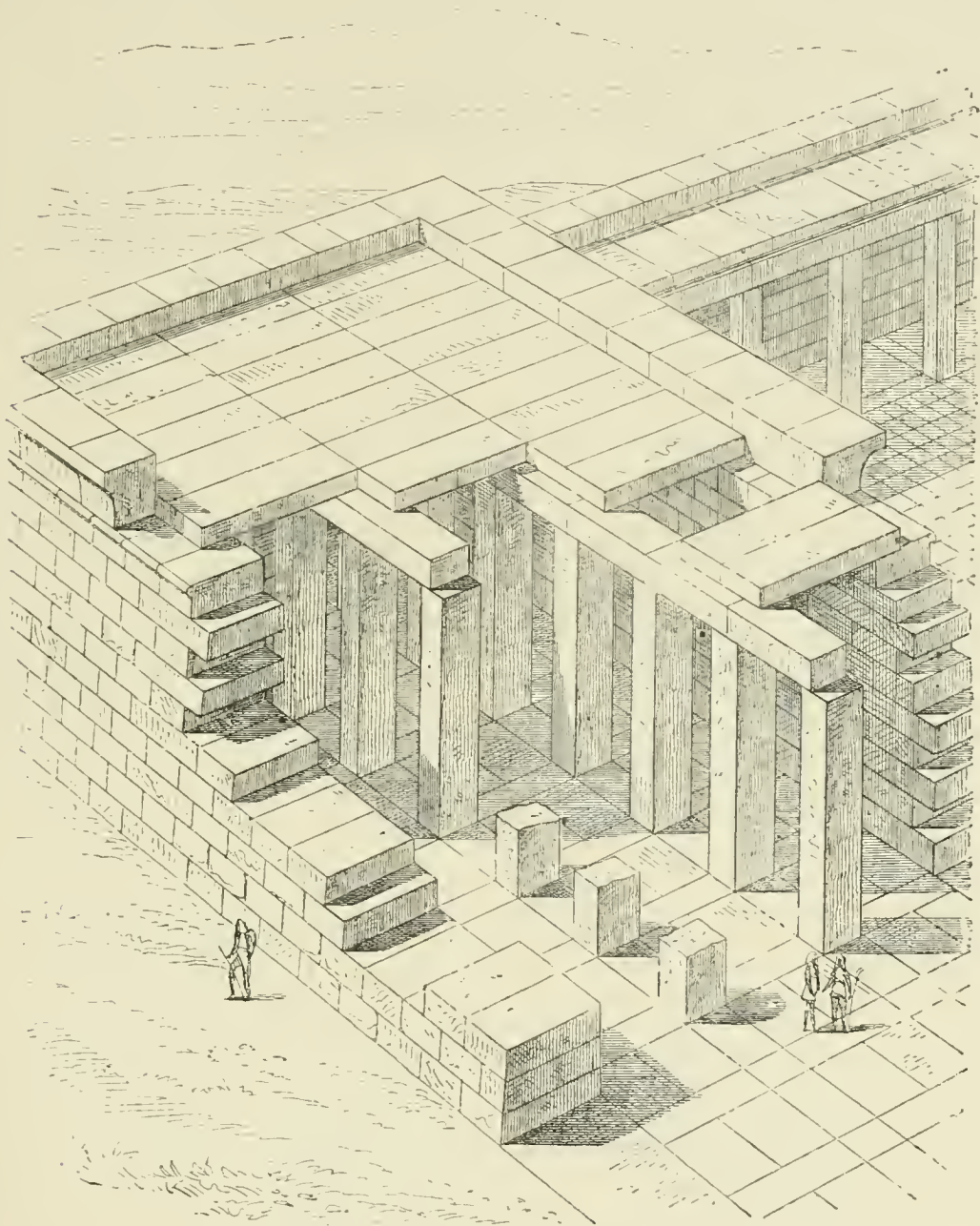
FIG. 73.—Egyptian construction, epitomized by Ch. Chipiez.
