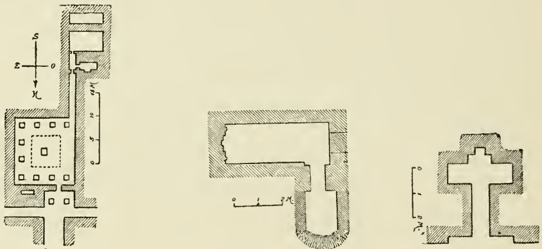
FIGS. 113, 114.—Mastaba at Sakkarah, from Prisse.
