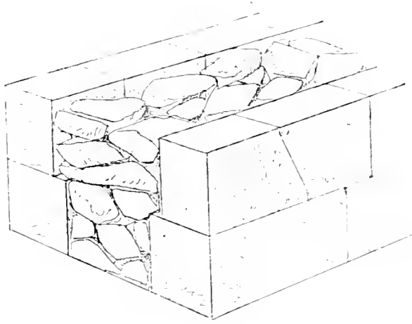
FIG. 70.—Double-faced wall.
