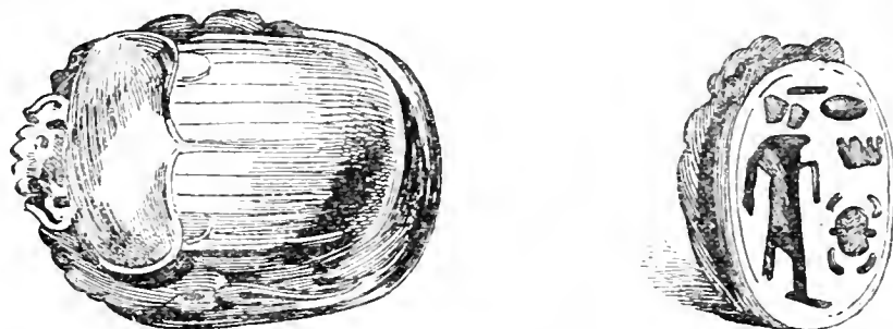
FIGS. 101, 102.—Scarabs. Louvre.
