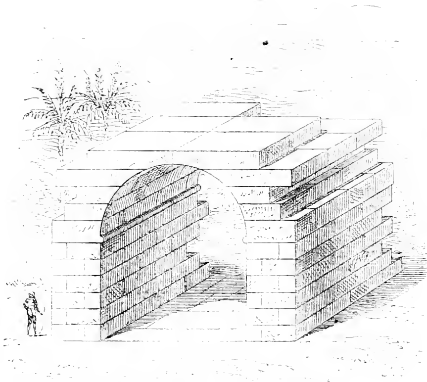
FIG. 76.—Off-set semicircular arch.
