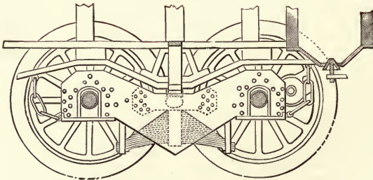
BALDWIN FLEXIBLE-BEAM TRUCK, 1842.—ELEVATION.
