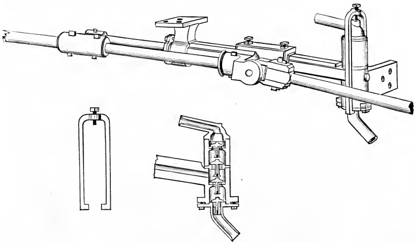
PUMP AND STIRRUP.
