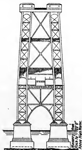
Elevation of Tower. Fig. 128.
