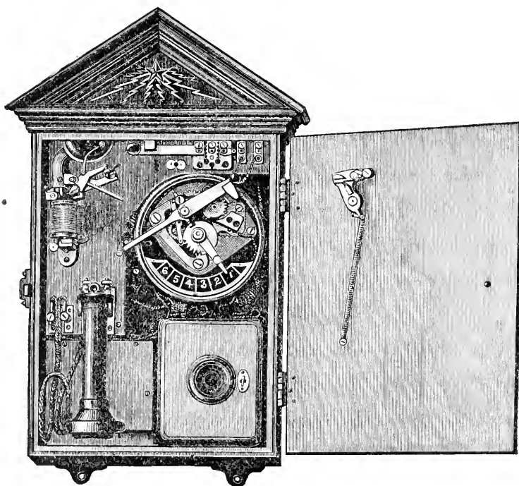
SIGNAL INSIDE BOX—OPEN.
