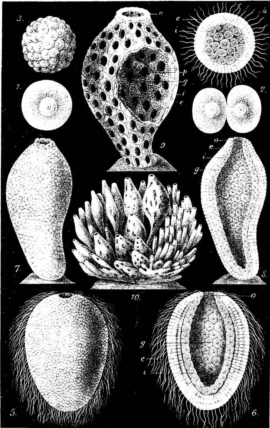
Development of a Calcareous Sponge (Olynthus)
