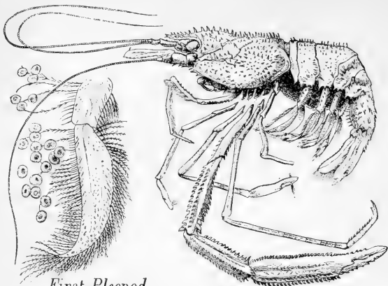
First Pleopod
