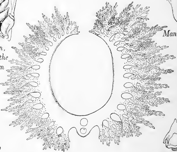
Epistome
