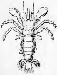
Pylocheles spinosus
