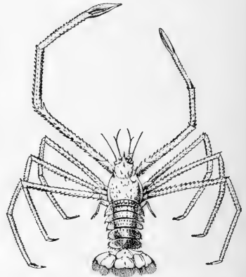
Ptychogaster Milne-edwardsi
