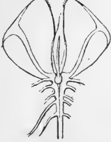
Lower Lip
