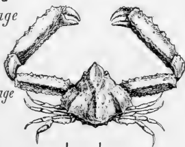
Lambrus intermedius
