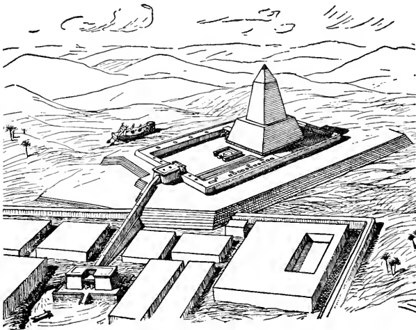
FIG. 71. RESTORATION OF THE SUN-TEMPLE OF NUSEBNE AT ABUSIR. (After Borchardt.)
