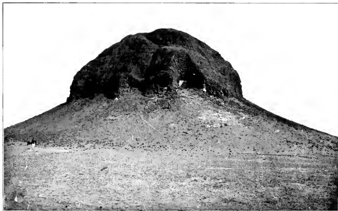
FIG. 91.—BRICK PYRAMID OF SESOSTRI II, AT ILLAHUN.
