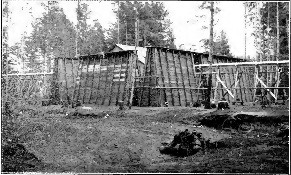
SEPARATING HOUSE.
