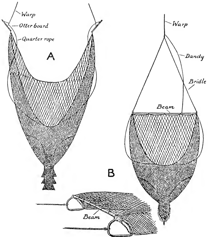
Fig. 137.—TRAWLS.
