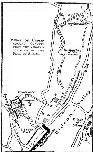
FIG. 98—THE SILOAM TUNNEL
