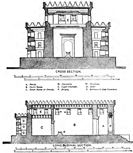
FIG. 66—CROSS AND LONGITUDINAL SECTIONS OF SOLOMON'S TEMPLE
