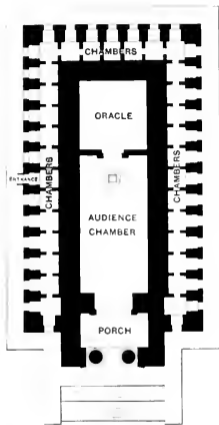
GROUND PLAN
