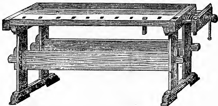
FIG. 24. SLOYD SCHOOL BENCH DESIGNED AT NÄÄS From Salomon: The Teacher's Handbook of Sloyd
