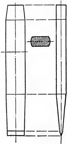
COLD CHISEL
