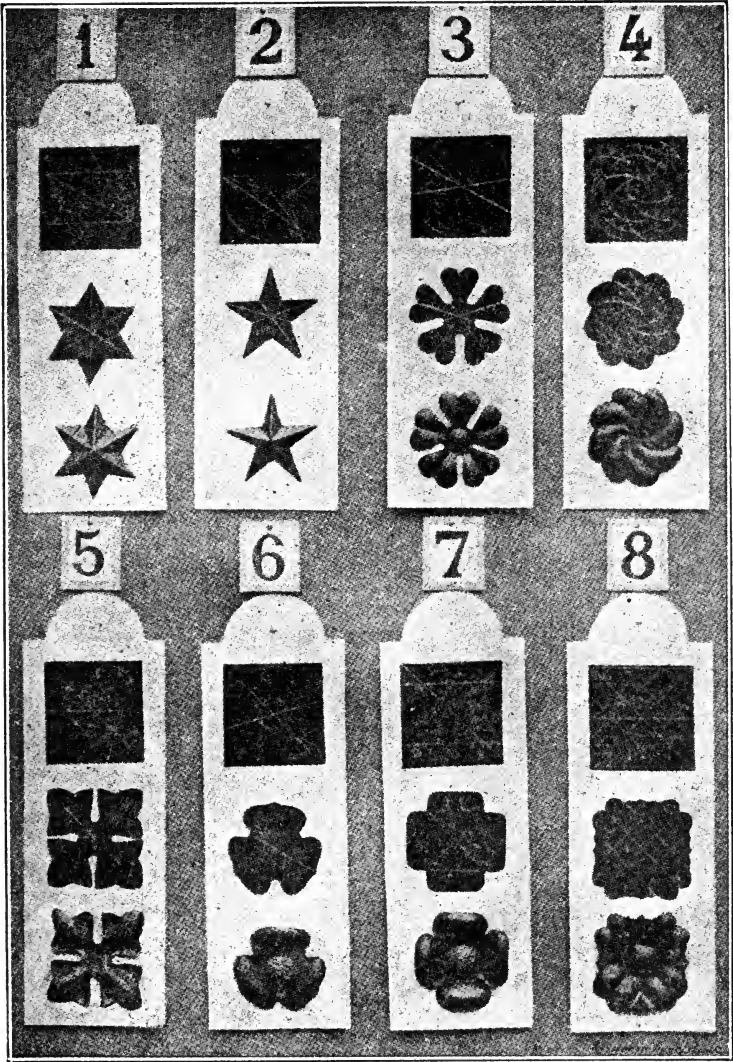
FIG. 56. COURSE IN RAISED SHEET METAL RECOMMENDED BY RENÉ LEBLANC
