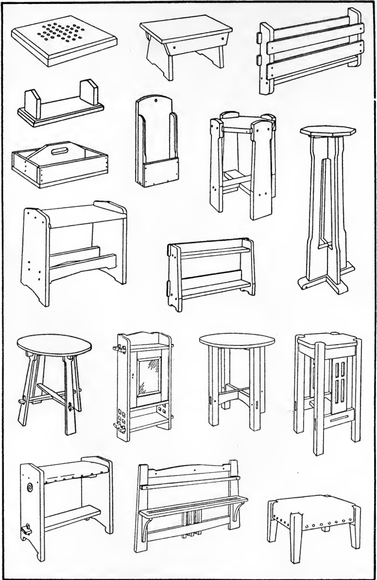
FIG. 129. GRAMMAR-GRADE PROBLEMS DESIGNED OR ADAPTED BY IRA S. GRIFFITH, 1912
