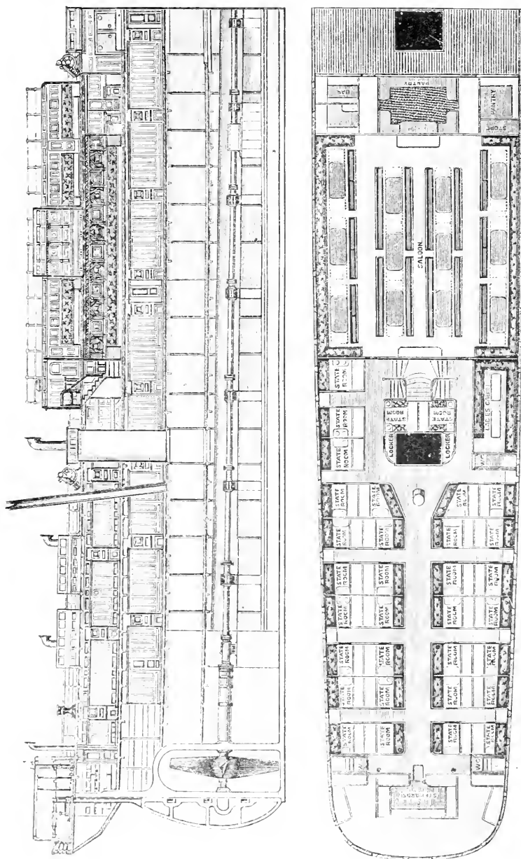
SECTION AND DECK OF CABINS OF THE CUNARD STEAM-SHIPS "BOTHNIA" AND "SCYTHIA."
