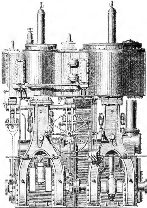
COMPOUND SURFACE ENGINE.
