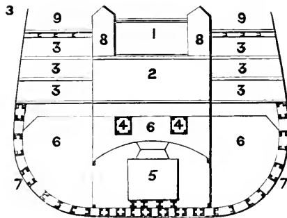
TRANSVERSE SECTION.
