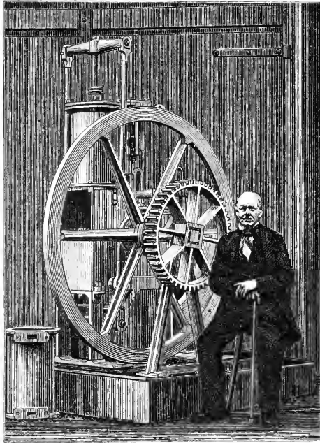
"COMET" ENGINE.
