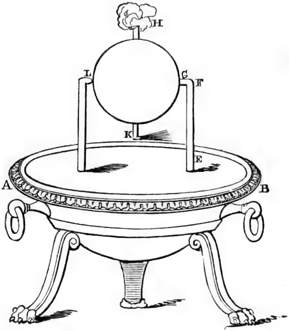
THE STEAM-ENGINE OF HERO
