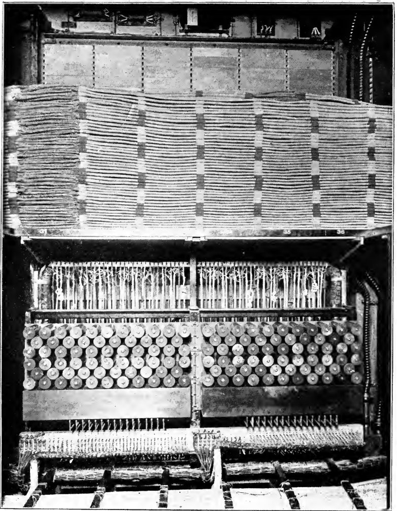
BACK SECTION OF MODERN SWITCHBOARD
