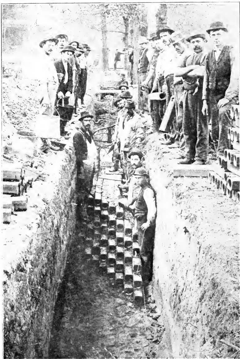
A SUBWAY LAID WITHOUT BOTTOM CONCRETE
