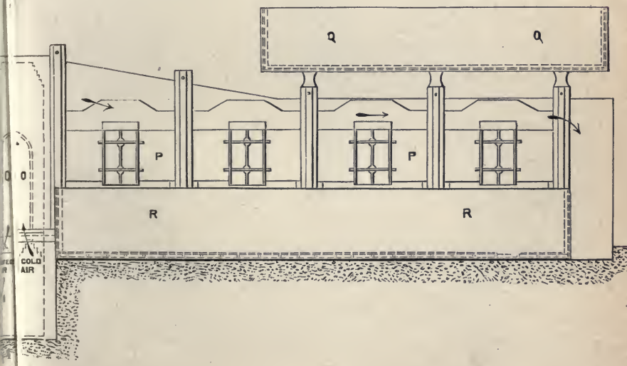
MAKING BLACK ASH (ELEVATION).
