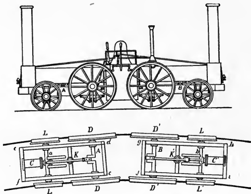
The "South Carolina," 1831, and plan of its running gear.
