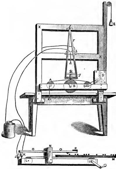
The First Telegraphic Instrument, as exhibited in 1837 by Morse.
