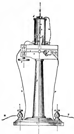
Edison's Platinum Lamp on Column Support, 1879.
