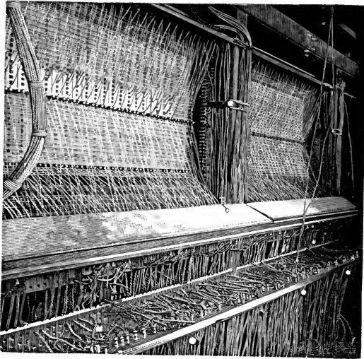
Under Side of a Modern Switchboard, showing 2,000 Telegraph Wires.
