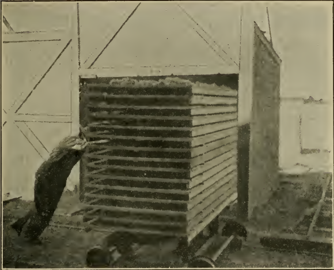
FIG. 40. Sulphuring Fruit on a Large Scale in California. The trays of fruit on car in picture have just been sulphured in the sulphur house in the background.
