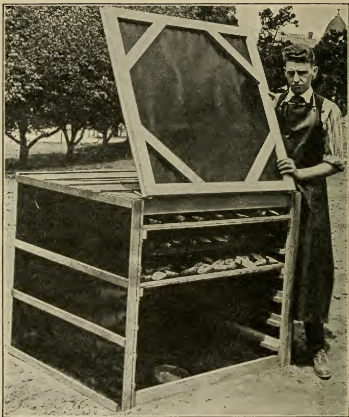
FIG. 39. Small Fruit Sulphuring Box for Home Use. Note pears cut in half for drying.
