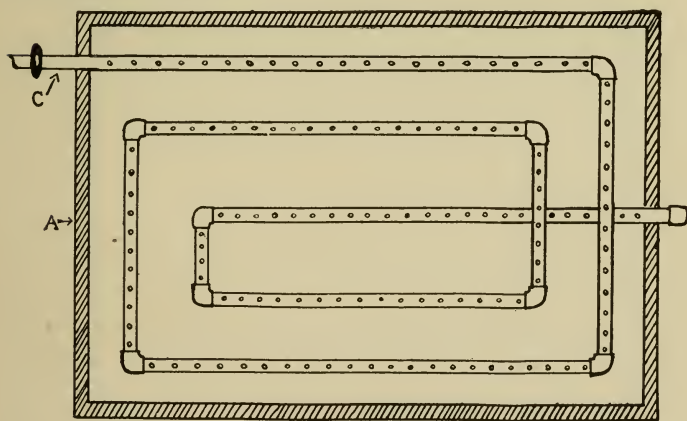
FIG. 27. Plan for Arrangement of Steam Coil of Fig. 26. Showing perforations for escape of steam for direct heating of water.
