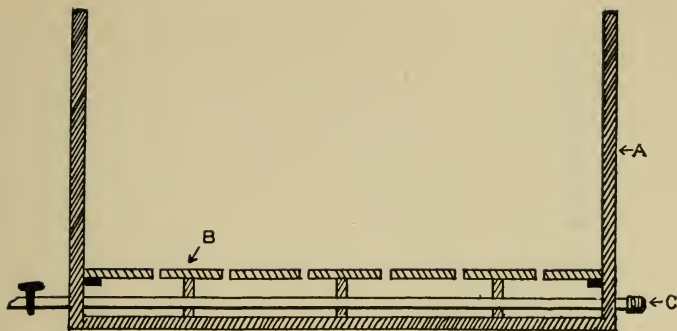
FIG. 26. Wooden Vat with Steam Coil for Use in Sterilizing Bottles of Juice or Cans of Food. A. Walls (of wood). B. False Bottom. C. Steam Coil.
