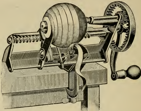
FIG. 4. Apple Peeling Machine for Home Use. (Courtesy of Berger and Carter Company, San Francisco, California.)
