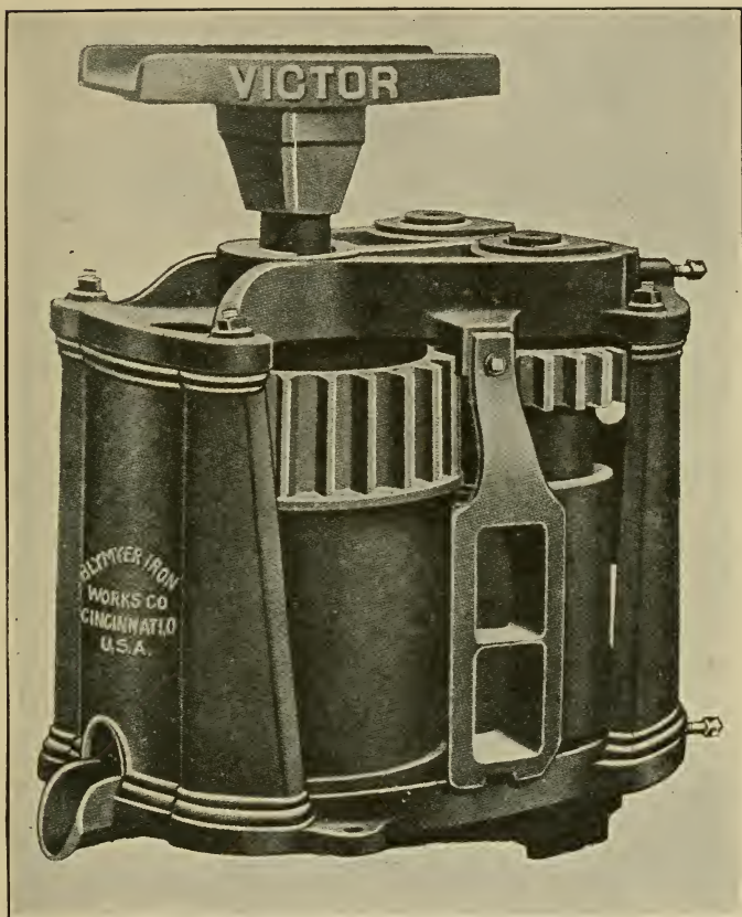
FIG. 58. Horse Power Sorghum or Cane Mill. (Courtesy Blymer Iron Works.)
