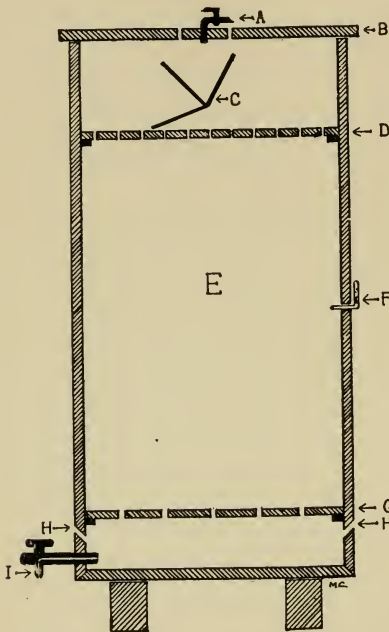
FIG. 50. Plan for Upright Vinegar Generator for Farm Use. A. Delivery pipe for fermented juice. B. Cover. C. Tilting trough to distribute liquid over false head. D. Perforated false head. E. Main cylinder of generator filled with shavings. F. Thermometer. G. Walls of generator. H. Air inlets. I. Outlet for vinegar.
