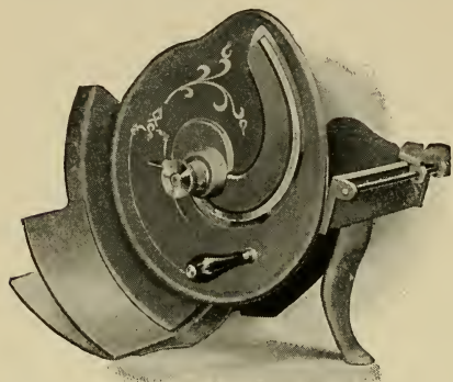
FIG. 61. Hand Power Vegetable Slicer (Courtesy Berger and Carter)
