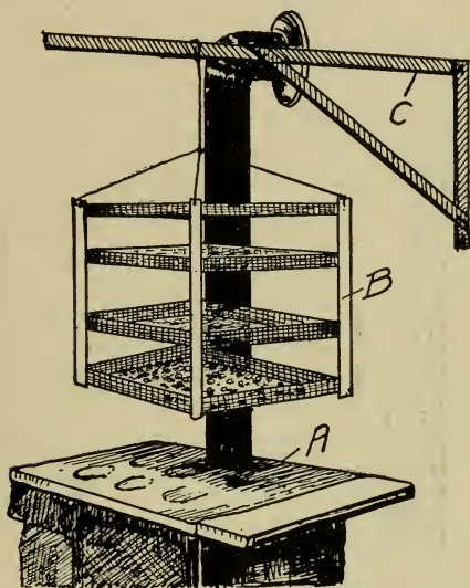
FIG. 44. A Home Made Dryer for Use above the Kitchen Stove. A. Stove. B. Frame with screen trays. C. Support. (After Farmers' Bulletin 841, United States Department of Agriculture.)
