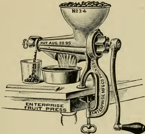
FIG. 20. Small Crusher for Home Use. (Courtesy of Berger and Carter Company, San Francisco, California.)
