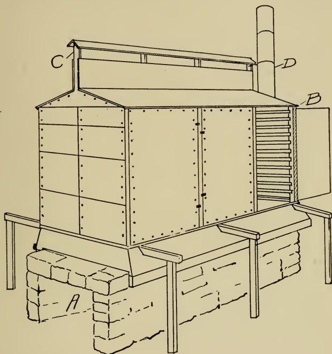
FIG. 46. Galvanized Iron Fruit and Vegetable Dryer for Farm Use. (After J. S. Caldwell, Extension Bulletin 27, Series I, State College of Washington.)
