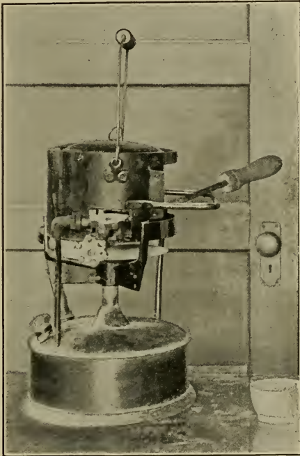
FIG. 11. Gasoline Fire Pot for Heating Soldering Irons.
