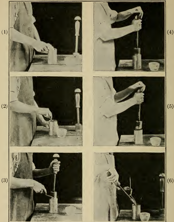
FIG. 57. Capping and Tipping a Solder Top Can. (1) Wipe off groove and cap with cloth to remove sirup, pulp, etc.; (2) Wipe groove with brush dipped in soldering fluid; (3) Apply hot capping steel and melt solder of solder hemmed cap or melt a little solder from solder wire; (4) Turn the steel two or three turns backward and forward to distribute solder evenly; (5) Raise the steel, but hold lid down for 2 or 3 seconds by center rod to allow solder to set; (6) wipe vent hole with soldering fluid; apply hot tipping steel and seal with drop of solder.
