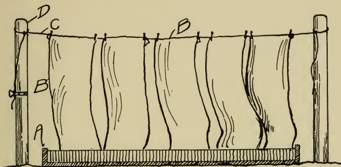
FIG. 29. Apparatus for Sun Evaporation of Fruit Juices. A. Shallow trough or pan to hold juice. B. Pieces of cheesecloth for evaporation of juice. C. Line to hold cloths. D. Posts for support of line.
