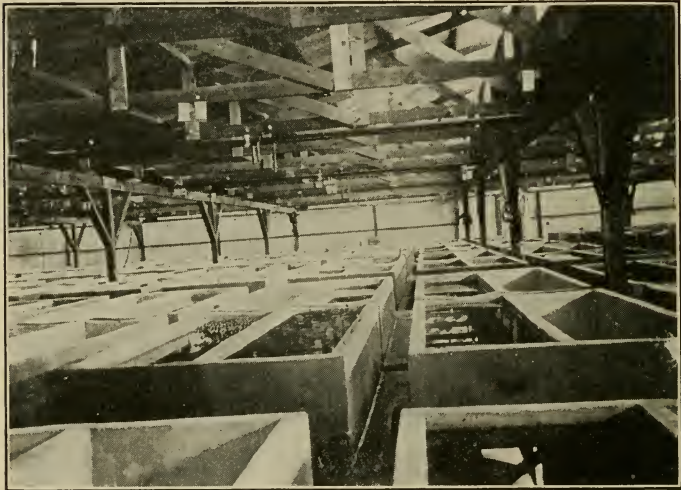
FIG. 55. Interior of Large Olive Pickling Plant.
