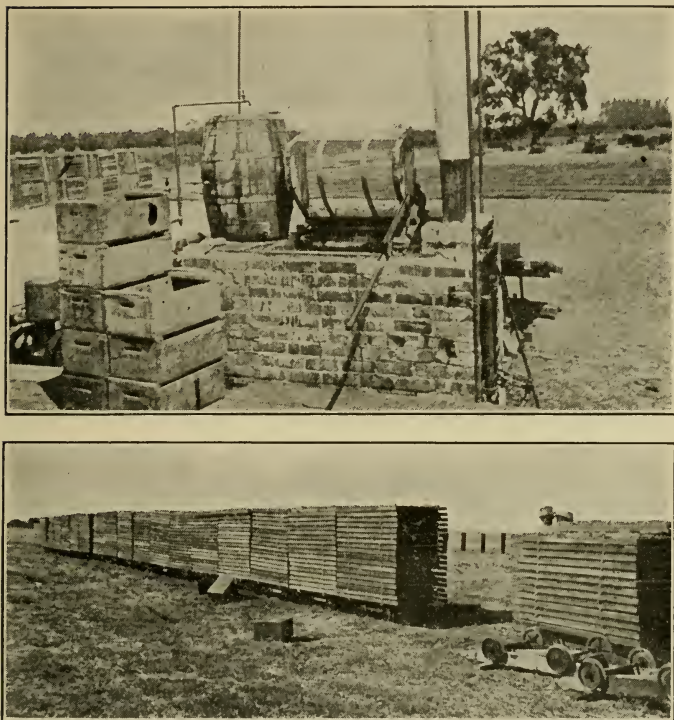
FIG. 37. Upper View, Fruit Dipper for Prunes. Lower View, Stacking Fruit that is nearly Dry. This permits drying to finish in the shade, giving a more uniform product.
