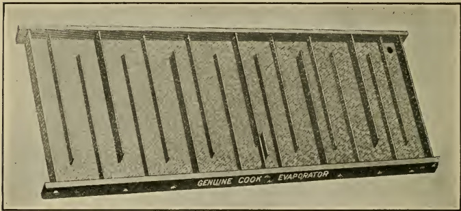
FIG. 59. Evaporating Pan for Sorghum and Other Sirups. (Courtesy Blymer Iron Works.)
