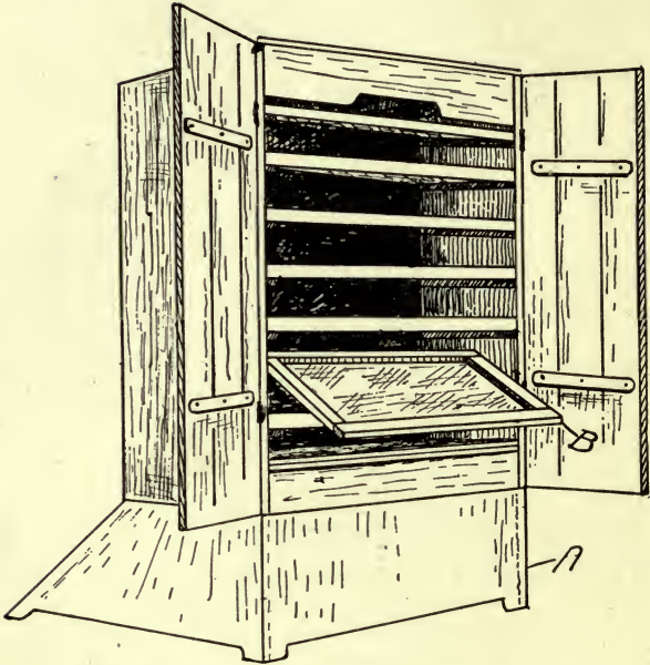
FIG. 45. Small Home Made Cabinet Dryer. Can be used on kitchen stove.
