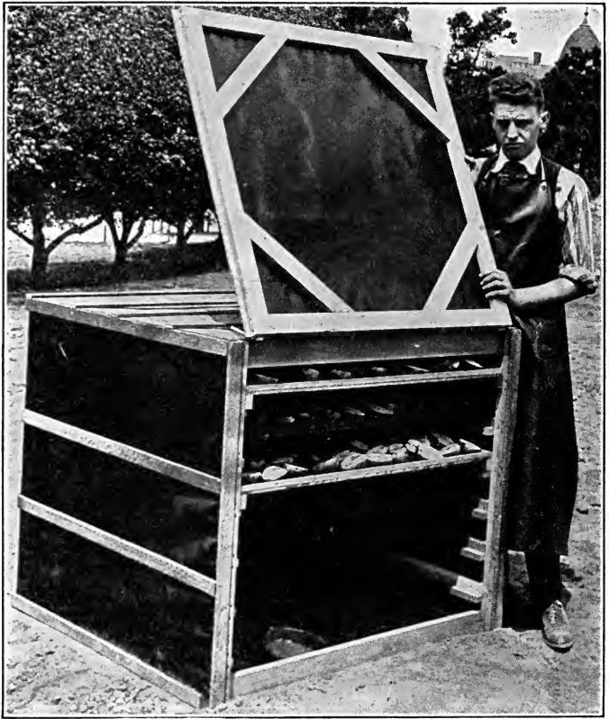
FIG. 39. Small Fruit Sulphuring Box for Home Use. Note pears cut in half for drying.
