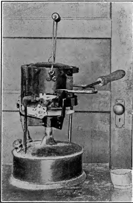
FIG. 11. Gasoline Fire Pot for Heating Soldering Irons.
