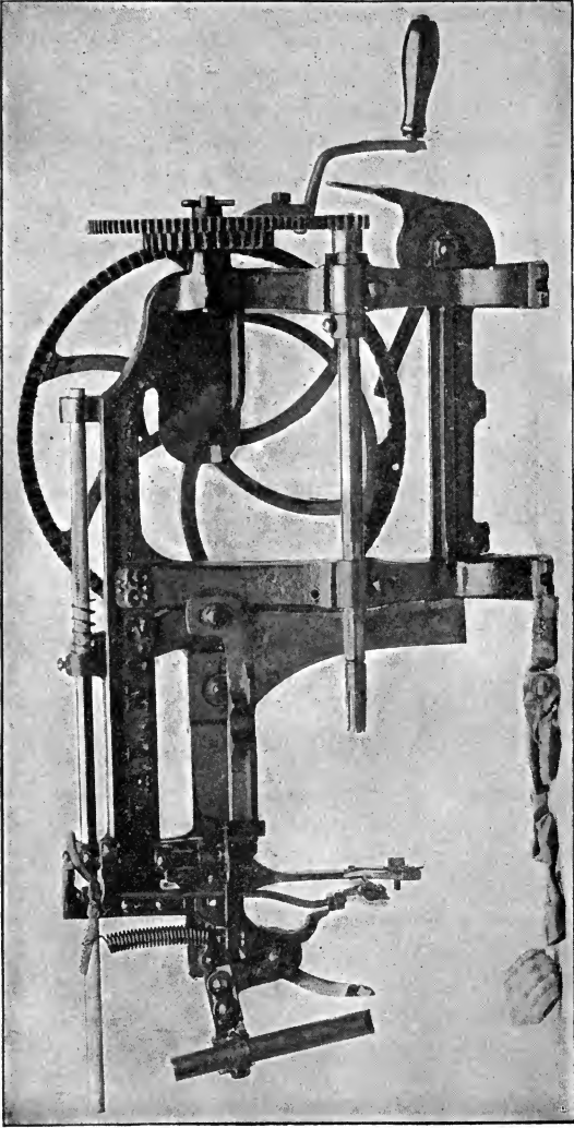
Fig. 60. Apple Peeler for Farm Use. (Courtesy of Berger and Carter)
