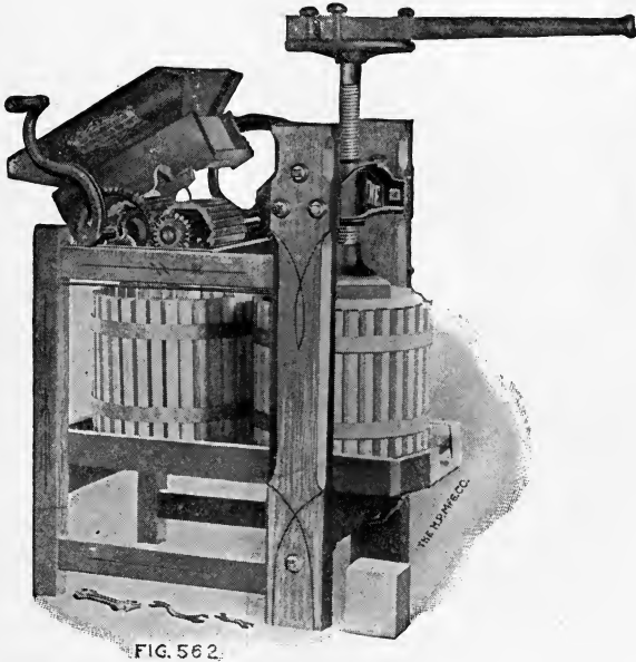
FIG. 22. Small Crusher and Press for Farm Use. (Courtesy of Berger and Carter Company, San Francisco, California.)
