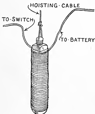
FIG. 180. — How the Electro-Magnet is Connected up.
