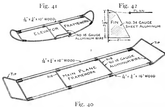
FIG. 40. — Detail of the Main Plane Framework of the Wells Model. FIG. 41. — Detail of the Elevator Framework. FIG. 42. — Detail of Fin.
