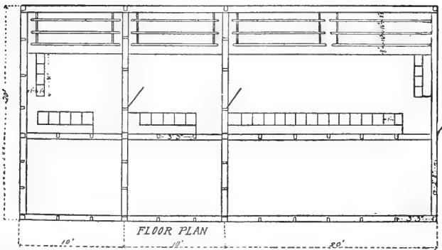
Details of the Clark semi-monitor, open-front house at the New Jersey State Experiment Station. A photograph of this house is shown on page facing 36
